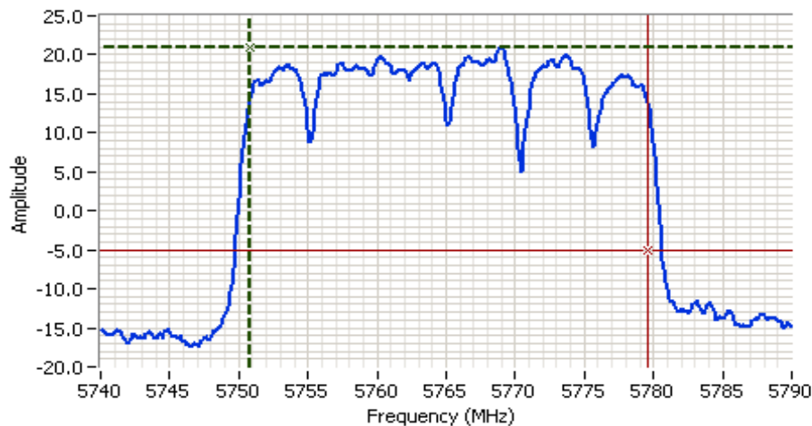
CU Ch Freq 5765 MHz @ 30 MHz Bandwidth
