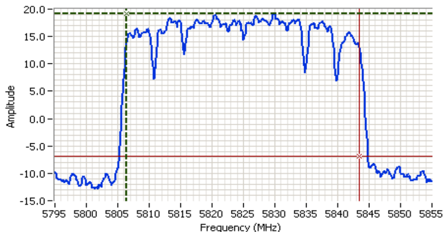
CU Ch Freq 5825 MHz @ 40 MHz Bandwidth
