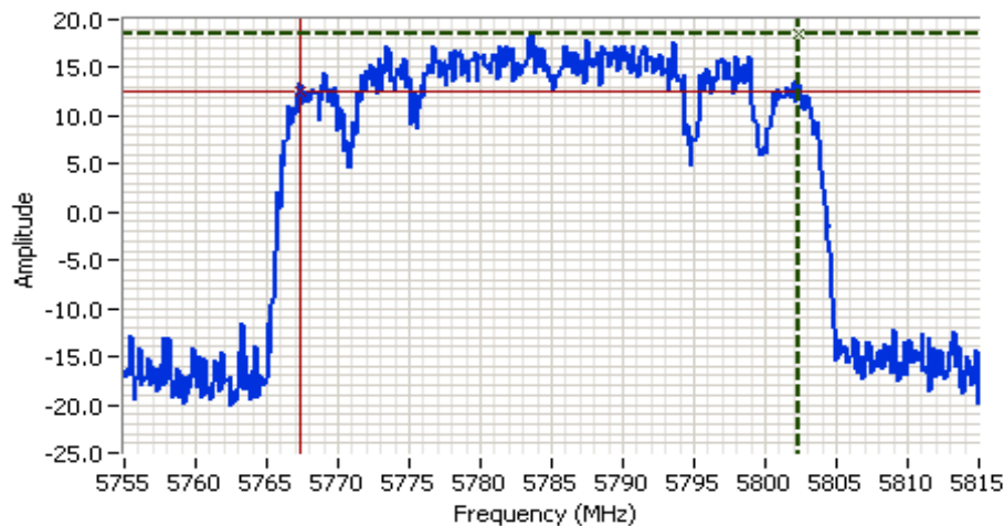
CU Ch Freq 5785 MHz @ 40 MHz Bandwidth
