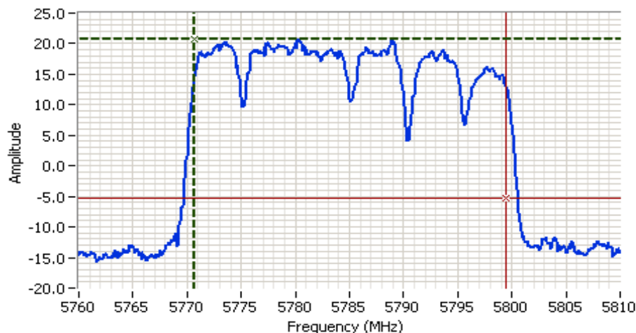
CU Ch Freq 5785 MHz @ 30 MHz Bandwidth
