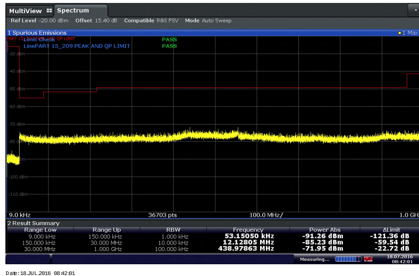
UNII 3 40MHz Bandwidth Low Channel 5745 MHz Below 1GHz
