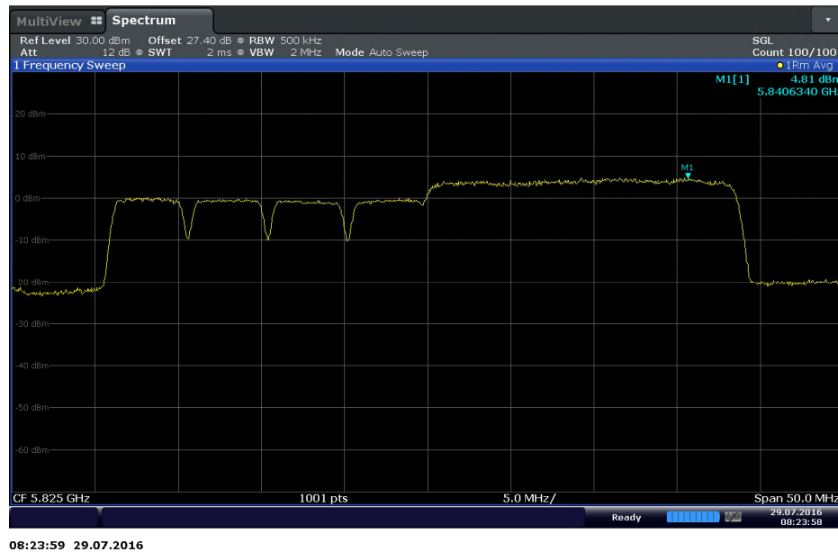
UNII 3 40MHz Bandwidth High Channel 5825 MHz
