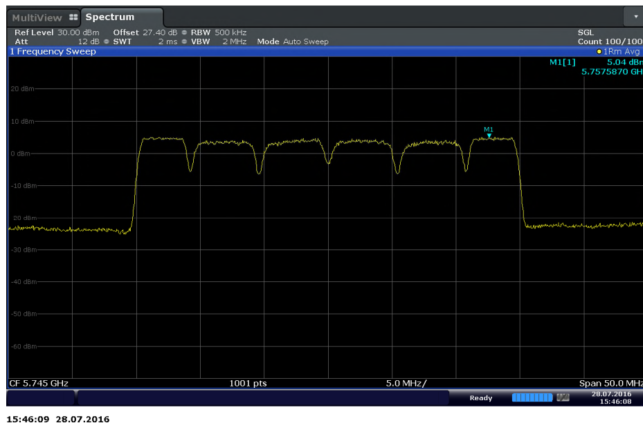
UNII 3 30MHz Bandwidth Low Channel 5745 MHz
