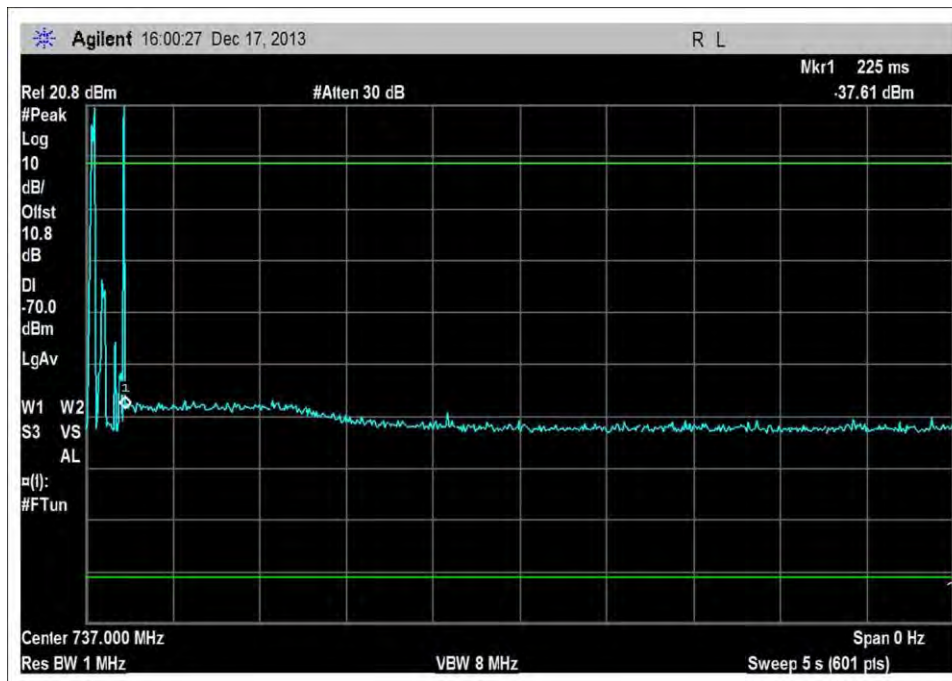
DL_716-746MHz_Single
