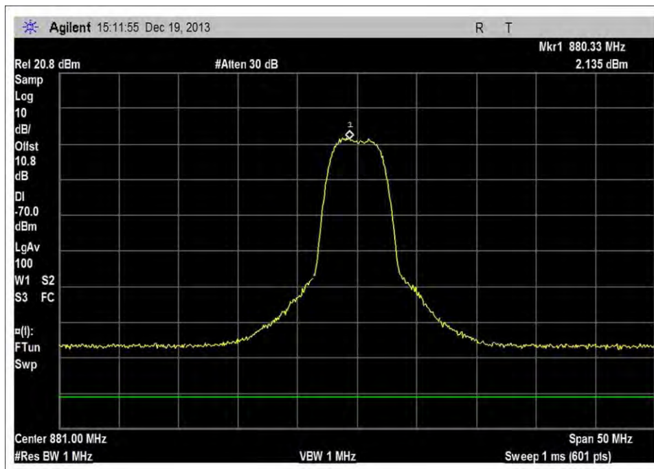
DL_869-894MHz_MNC410
