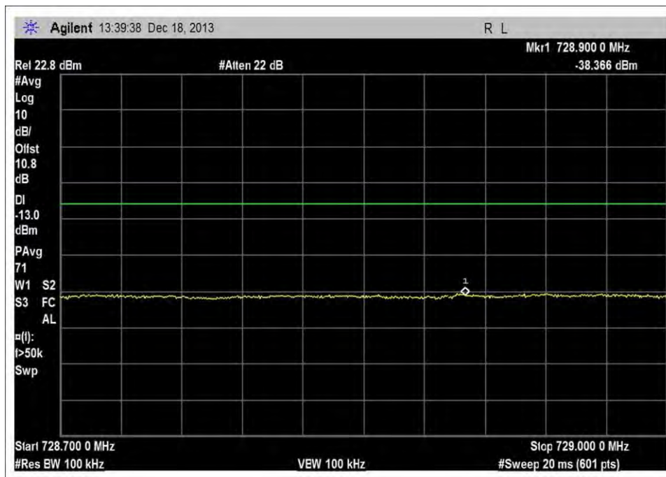
DL_716-746MHz_L_-20dBm
