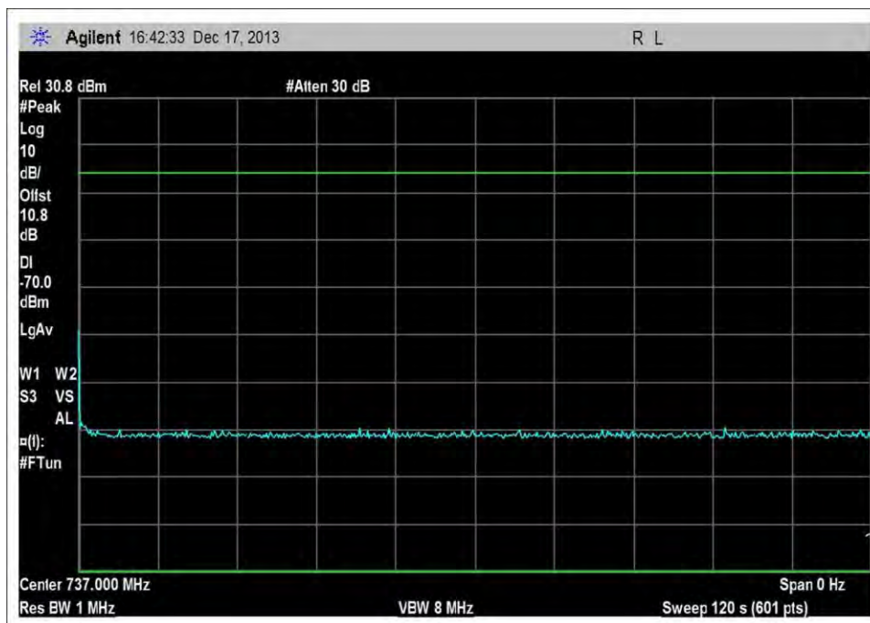
DL_716-746MHz_Single-120sec
