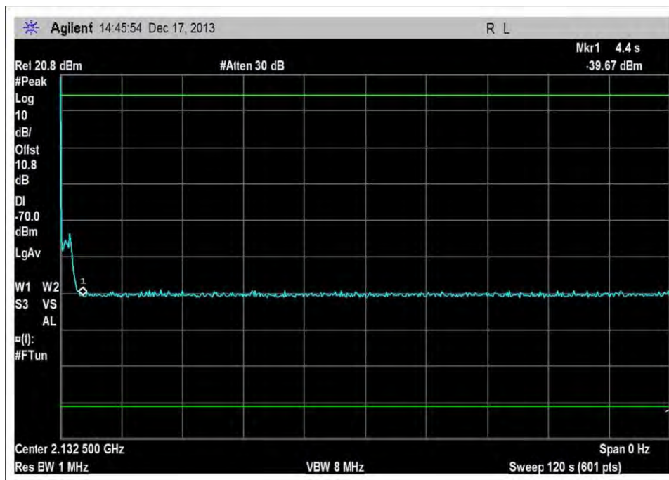
DL_2110-2155MHz_Single_120sec
