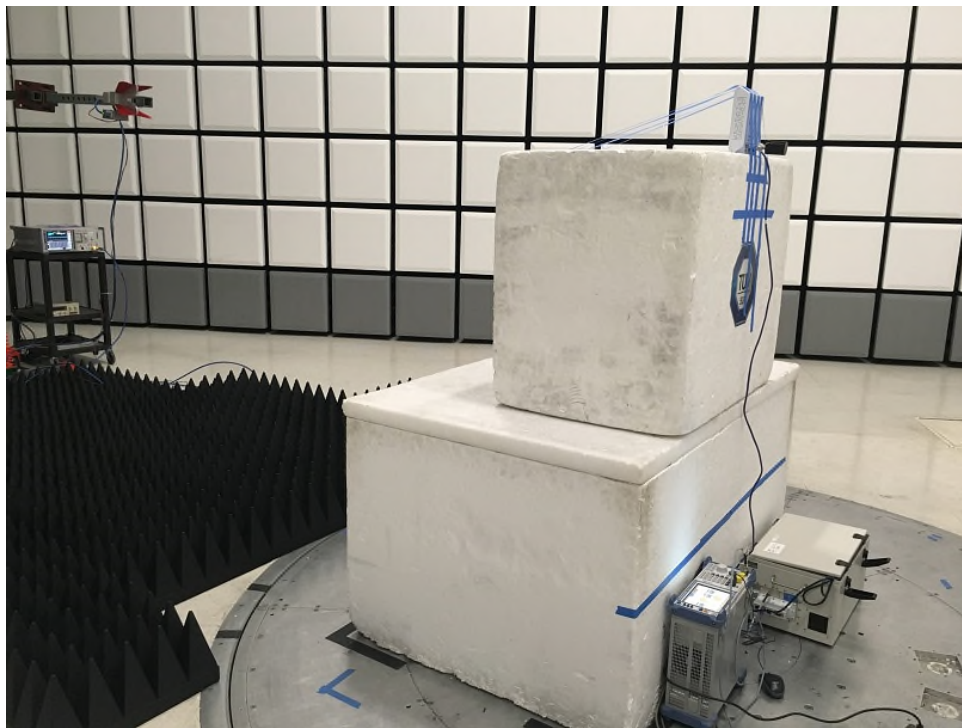
CU Radiated Emissions Above 1GHz Rear
