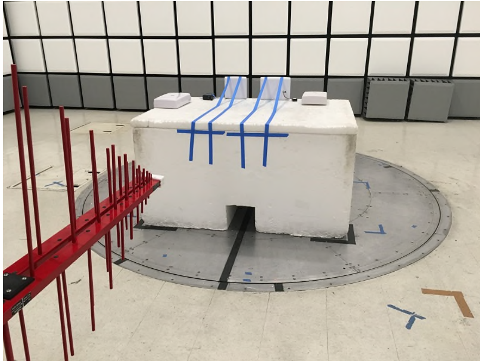
Radiated Emissions Below 1GHz Front (Unintentional)
