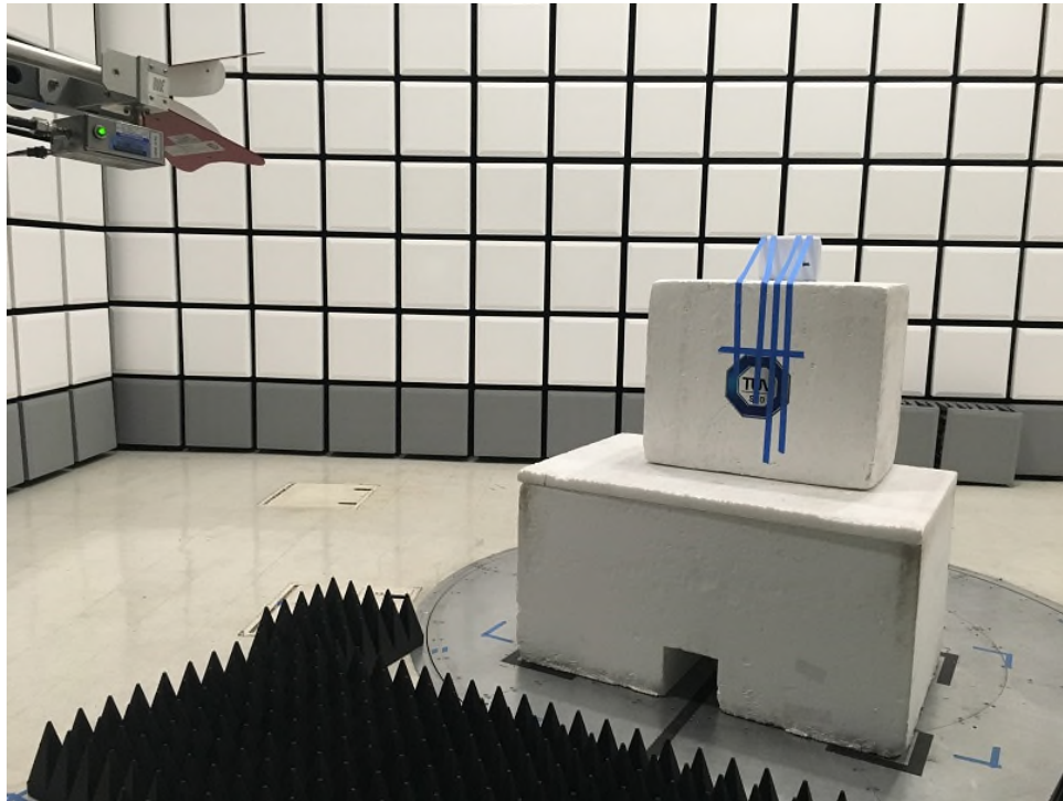
NU Radiated Emissions Above 1GHz Front
