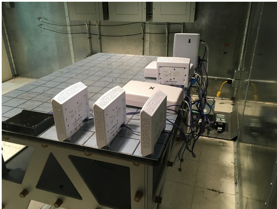
Conducted Emissions (Unintentional)
