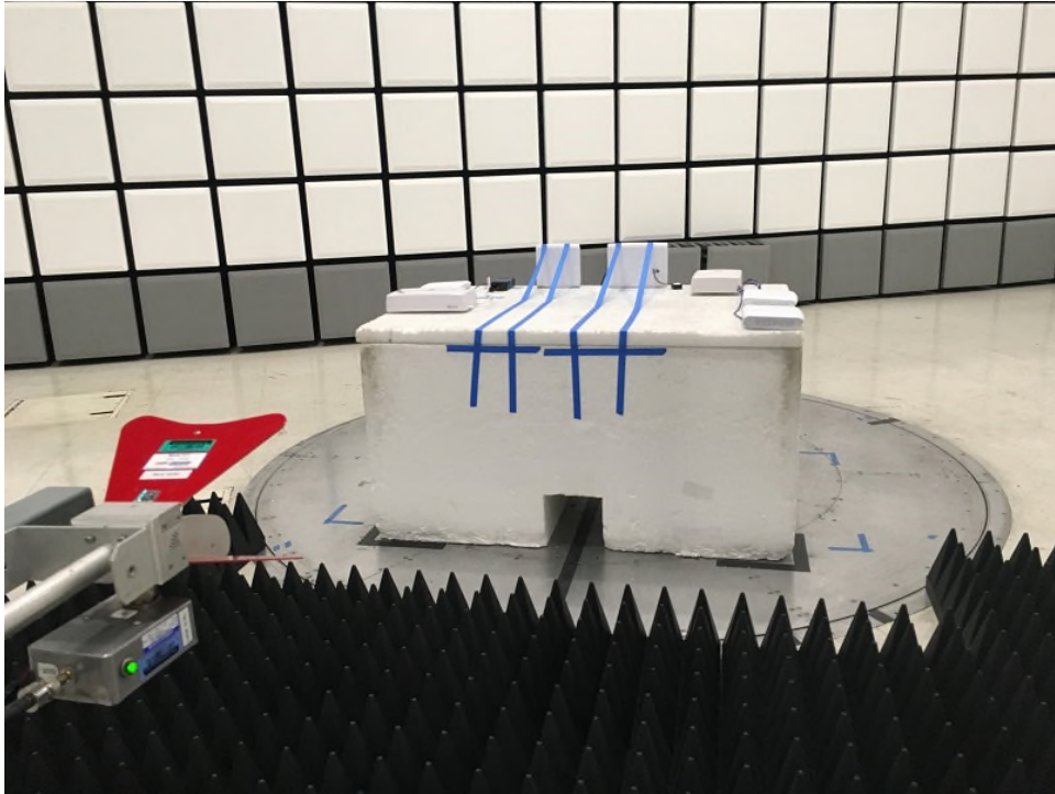
Radiated Emissions Above 1GHz Front (Unintentional)
