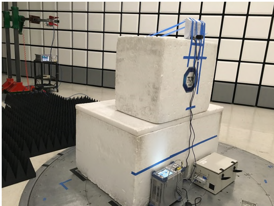
NU Radiated Emissions Above 1GHz Rear
