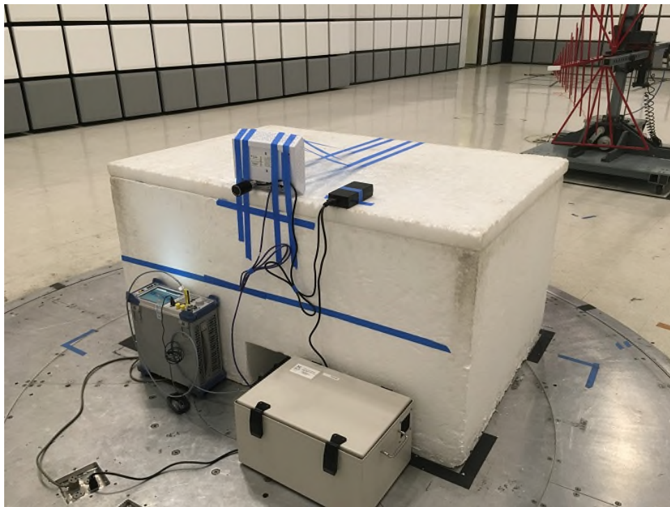
NU Radiated Emissions Below 1GHz Rear
