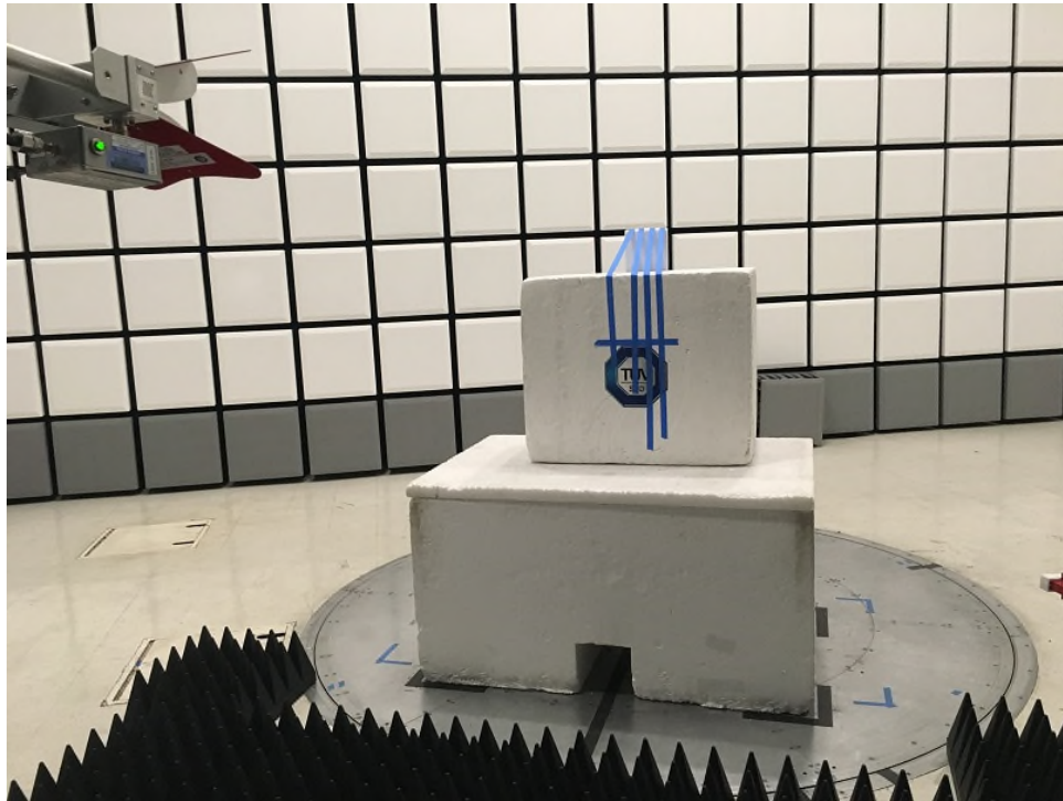
CU Radiated Emissions Above 1GHz Front
