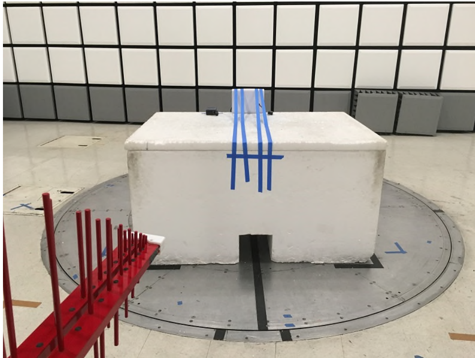
NU Radiated Emissions Below 1GHz Front
