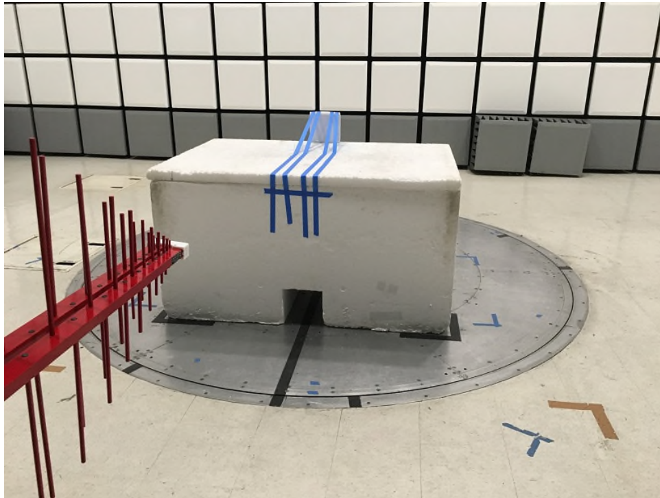
CU Radiated Emissions Below 1GHz Front
