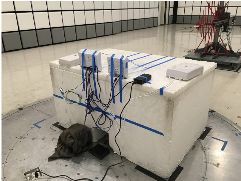
Radiated Emissions Below 1GHz Rear (Unintentional)
