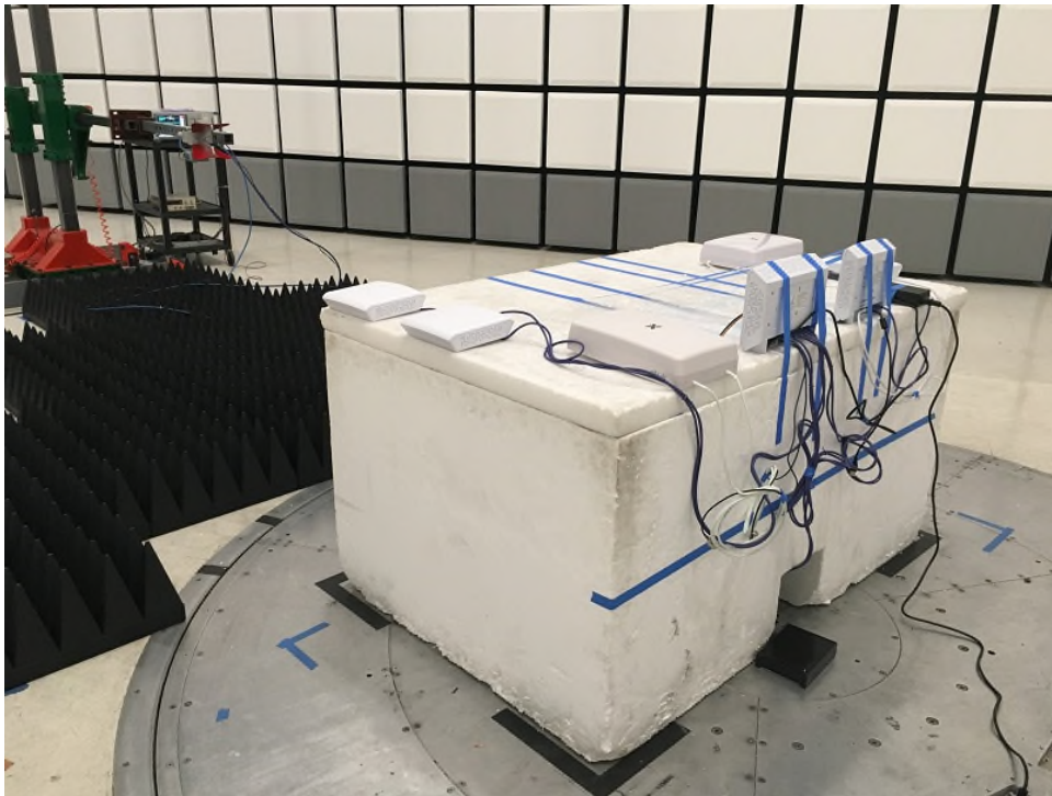
Radiated Emissions Above 1GHz 1GHz Rear (Unintentional)
