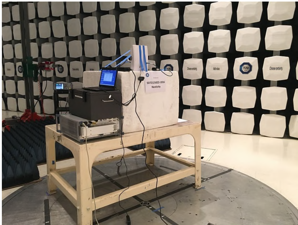
NU Radiated Emissionsv Above 1GHz Rear
