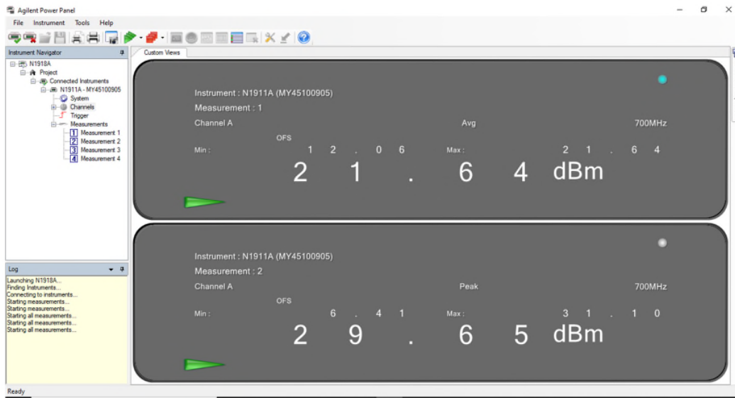
LTE Band 13 UL 5 MHz Bandwidth Middle Channel
