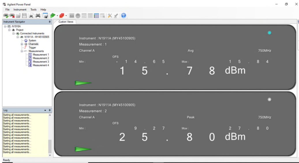
LTE Band 13 DL 5 MHz Bandwidth Middle Channel
