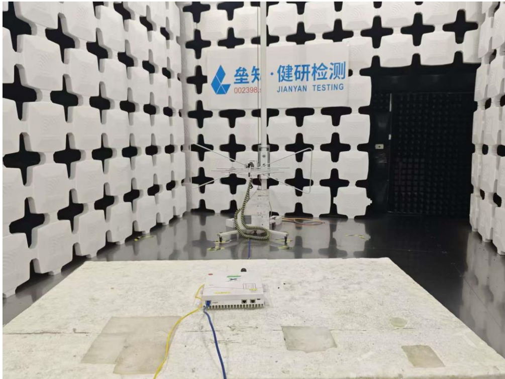
NU Radiated Spurious Emission Below 1GHz
