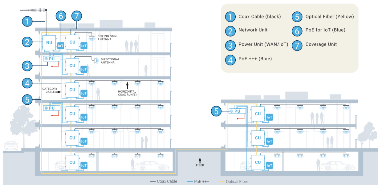
Figure 2: QUATRA 100M system layout illustrating NUs, CUs, PUs, optical and coaxial cabling, and PoE IoT device integration throughout the building.
