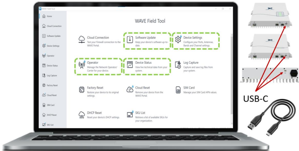
Figure 35: Commissioning with the WAVE Field Tool – connect a PC to each powered unit (NU, CU, PU) via USB-C data cable to update software, configure settings, and check device status.
