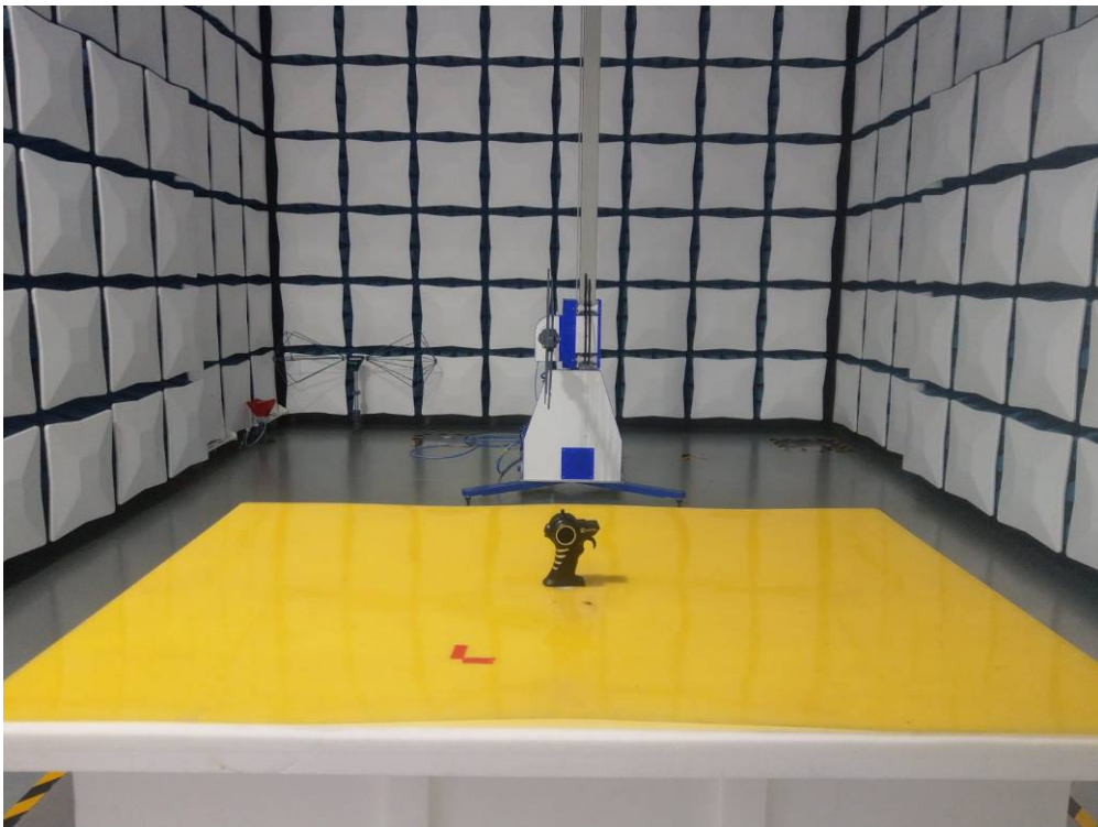
Setup for Radiated Emissions
