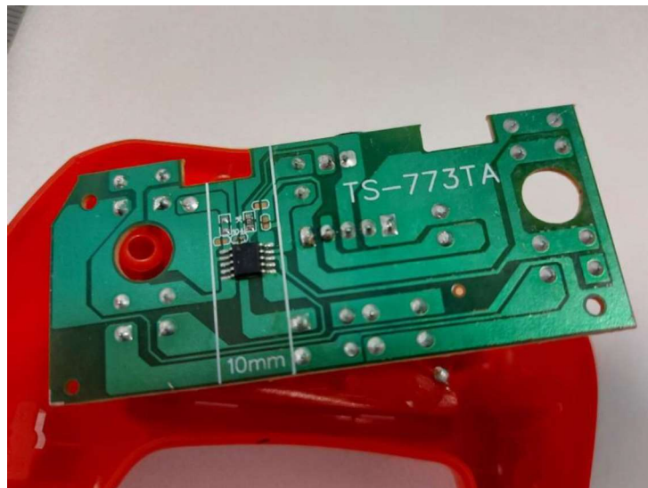
Internal View
