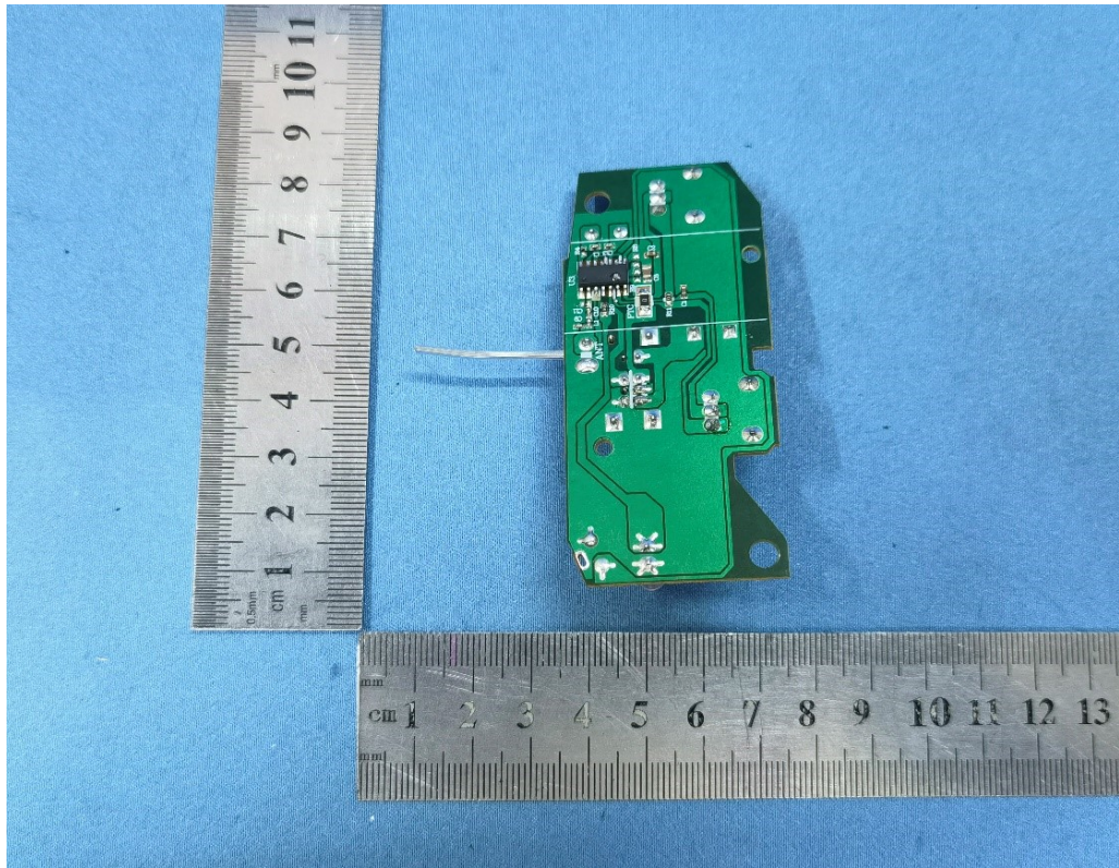
Internal View
