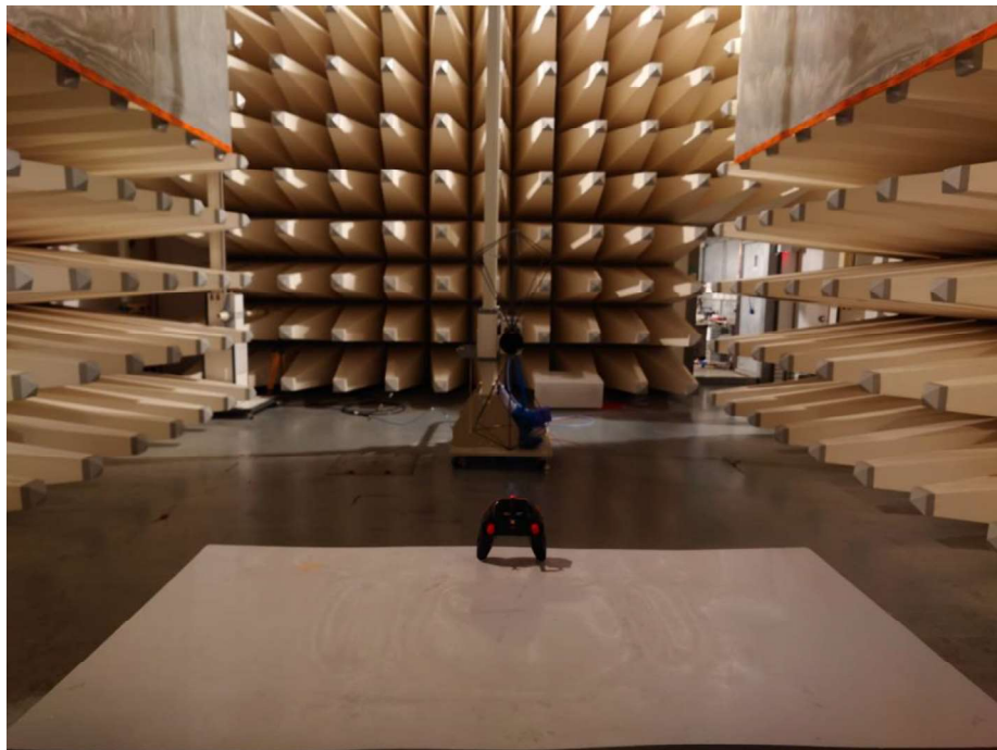
Set-up for Radiated Emission (30-200MHz)
