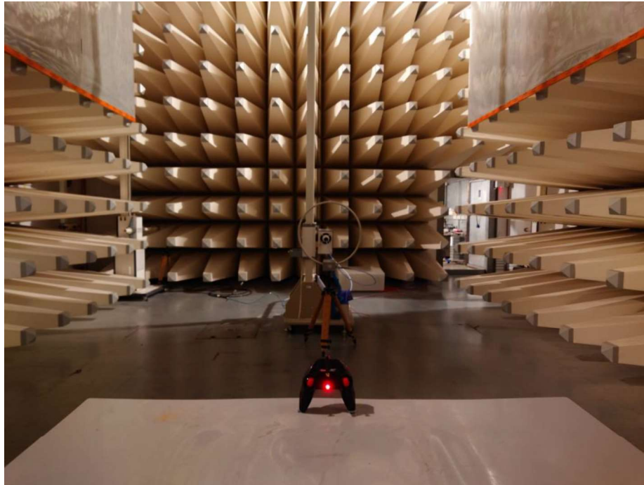
Set-up for Radiated Emission (9k-30MHz)
