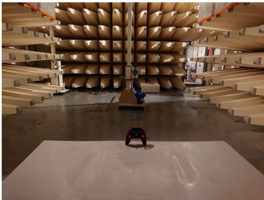
Set-up for Radiated Emission (200-1000MHz)
