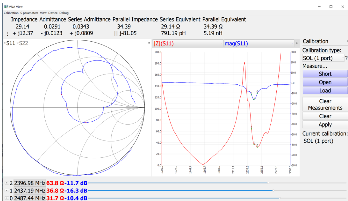
Fig.5 BT-PCB antenna test results
