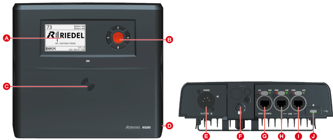
Figure 210: Antenna Operating Elements (front, bottom)
