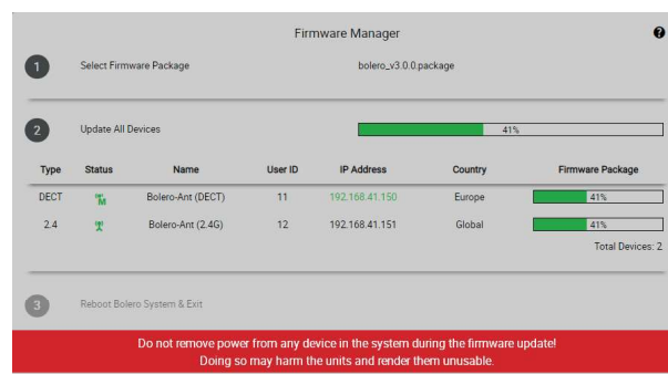
Figure 143: Firmware-Manager – progress
