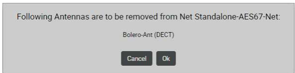
Figure 130: Confirmation dialog
