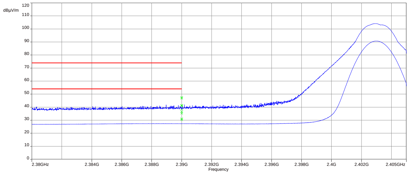
Plot 3: Lower band edge, vertical & horizontal polarization, antenna 2
