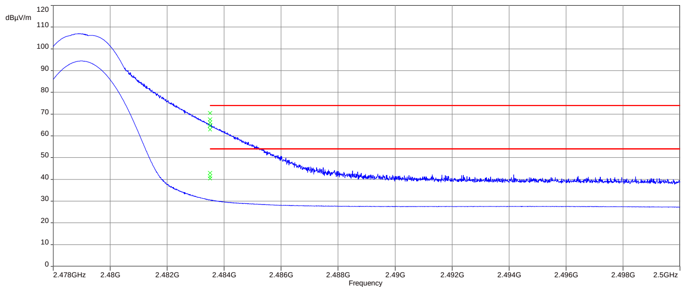
Plot 2: Upper band edge, vertical & horizontal polarization, antenna 1
