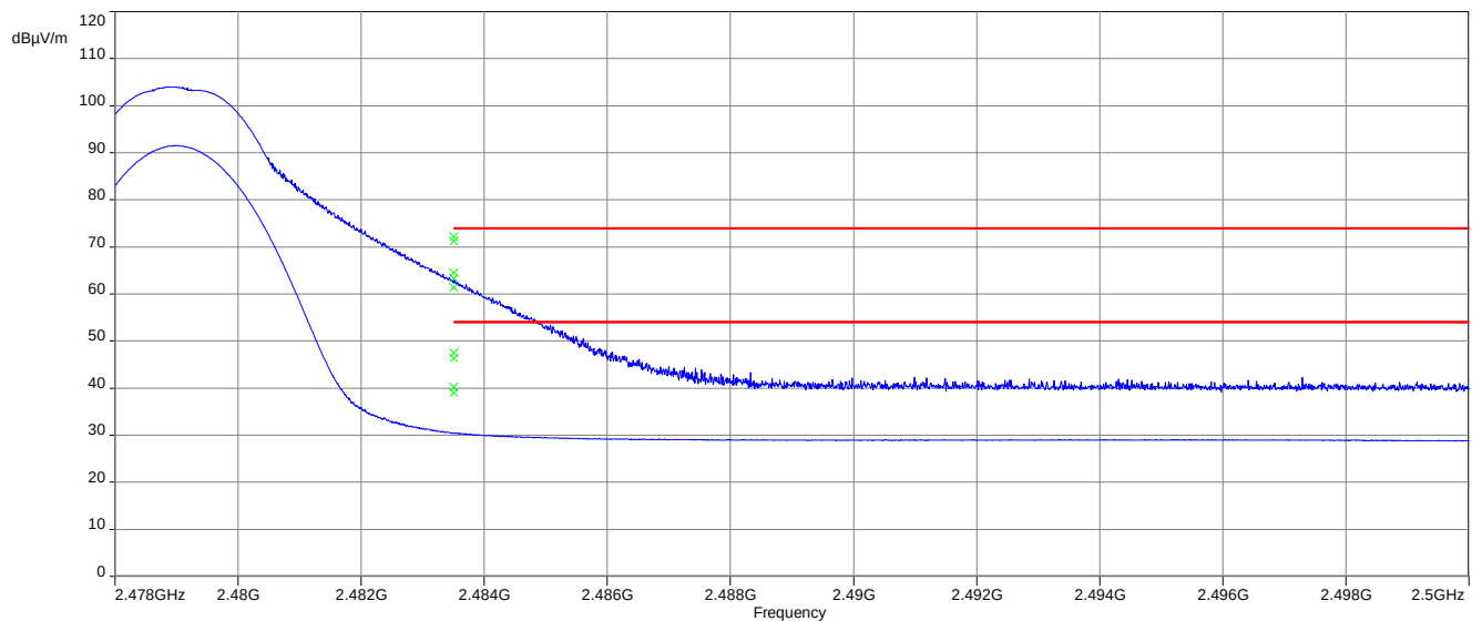
Plot 4: Upper band edge, vertical & horizontal polarization, antenna 2
