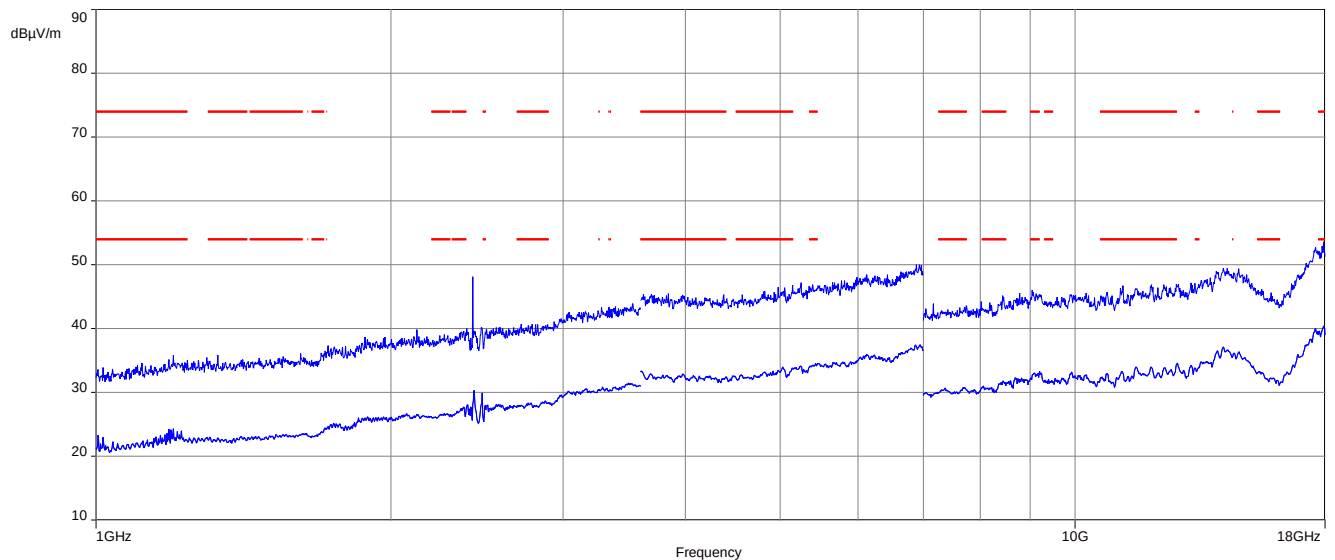
Plot 3: 1 GHz to 18 GHz, TX mode, highest channel, vertical & horizontal polarization
