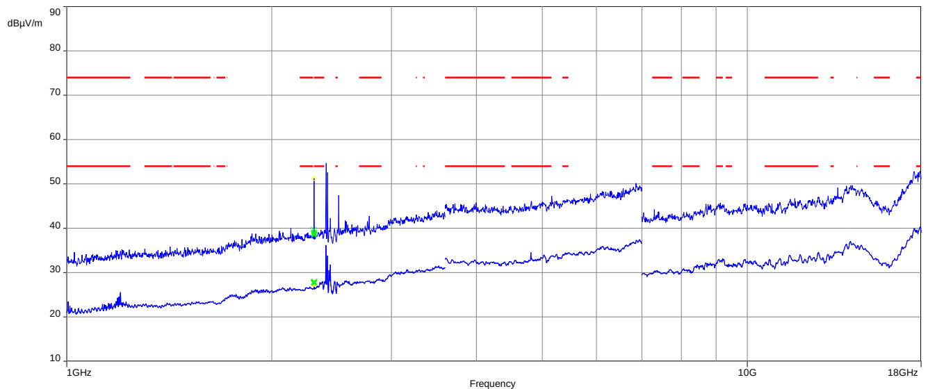
Plot 1: 1 GHz to 18 GHz, TX mode, lowest channel, vertical & horizontal polarization
