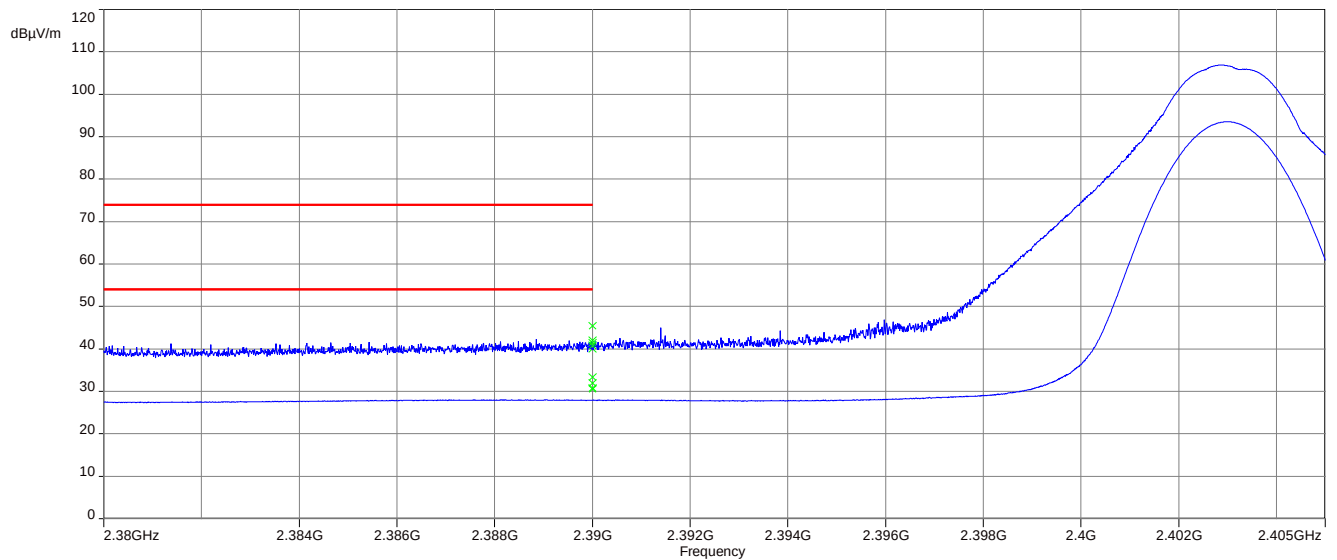
Plot 1: Lower band edge, vertical & horizontal polarization, antenna 1
