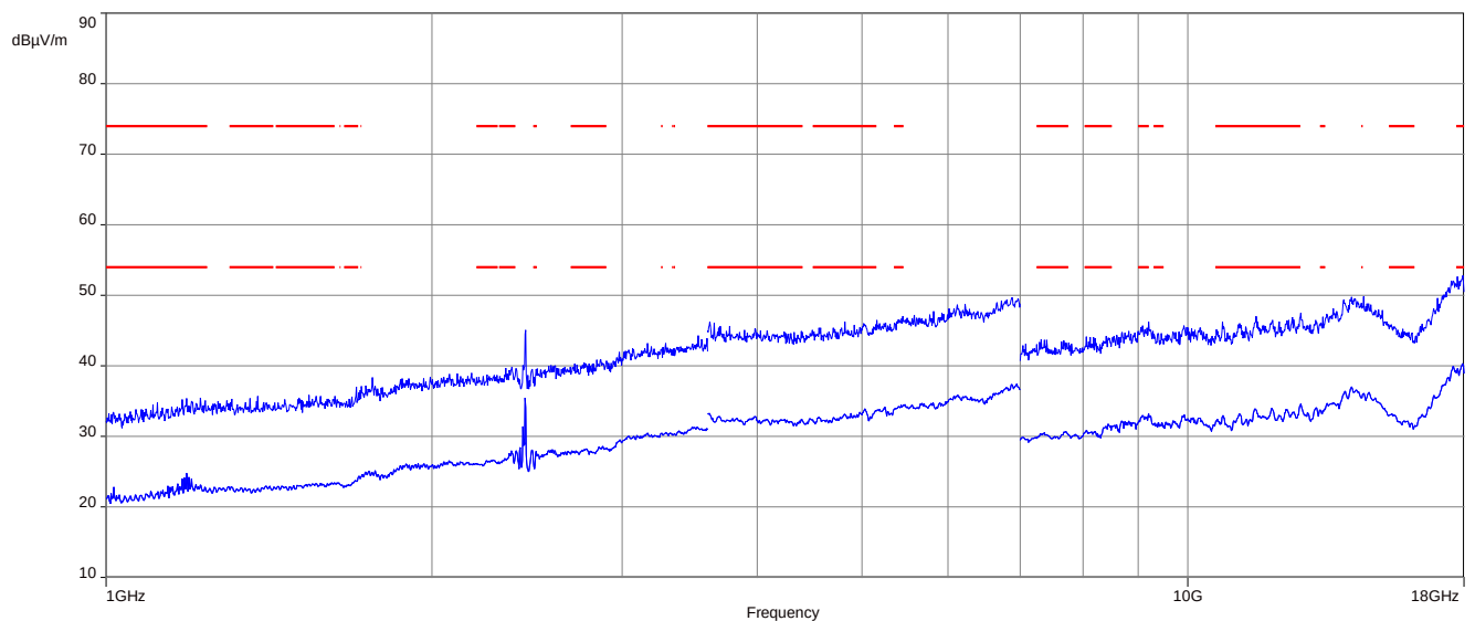
Plot 2: 1 GHz to 18 GHz, TX mode, middle channel, vertical & horizontal polarization
