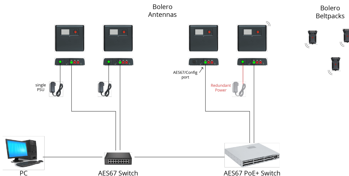
Figure 4: Standalone/AES67 (2110)
