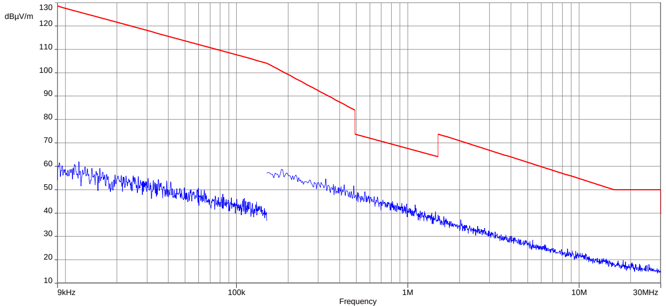
Plot 3: 9 kHz to 30 MHz, highest channel, transmit mode, Antenna 1
