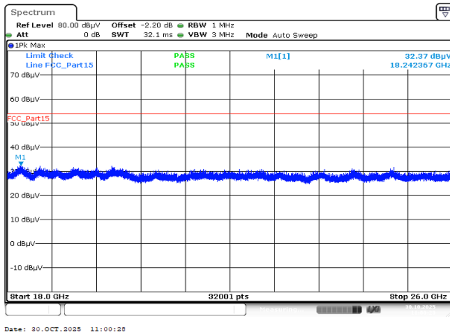
Plot 4: 18 GHz to 26 GHz, TX mode, channel 78, vertical & horizontal polarization
