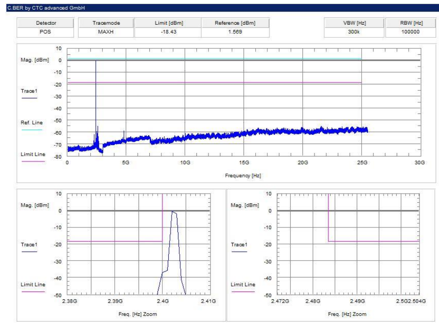
Plot 4: lowest channel – 2402 MHz, Pi/4-DQPSK modulation
