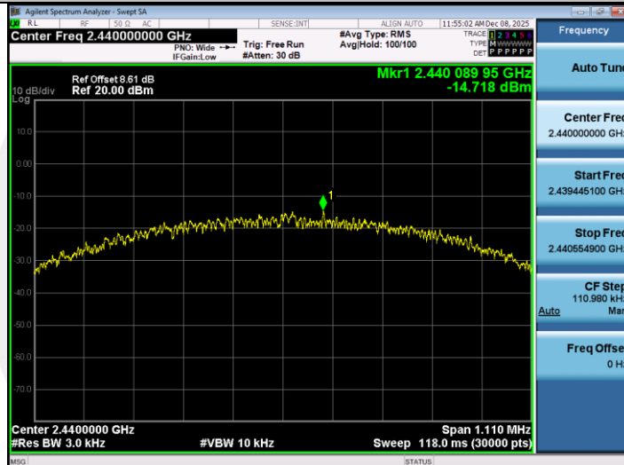
SRD-Ant1-2440-PASS
