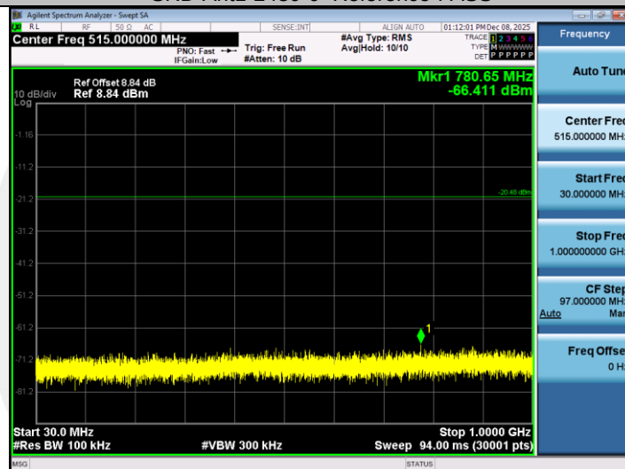
SRD-Ant1-2480-30~1000-PASS
