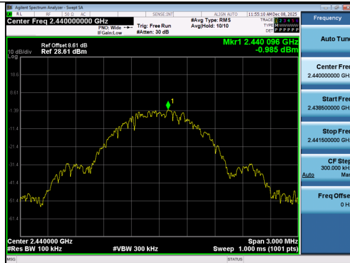
SRD-Ant1-2440-0~Reference-PASS
