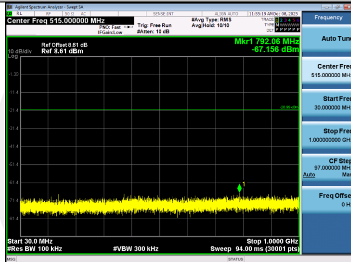
SRD-Ant1-2440-30~1000-PASS
