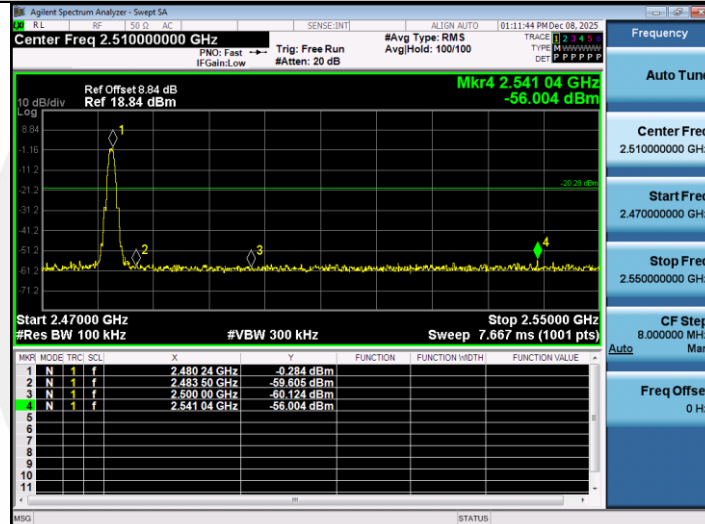
SRD-Ant1-2480-PASS
