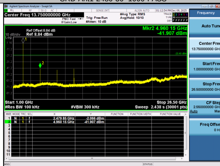
SRD-Ant1-2480-1000~26500-PASS
