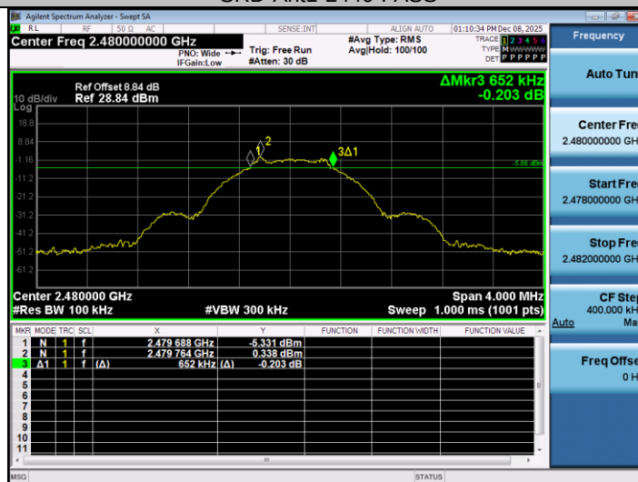
SRD-Ant1-2480-PASS
