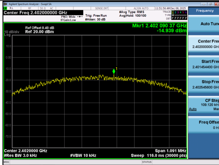
SRD-Ant1-2402-PASS
