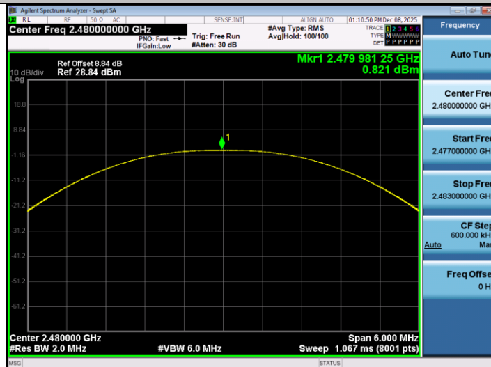
SRD-Ant1-2480-PASS
