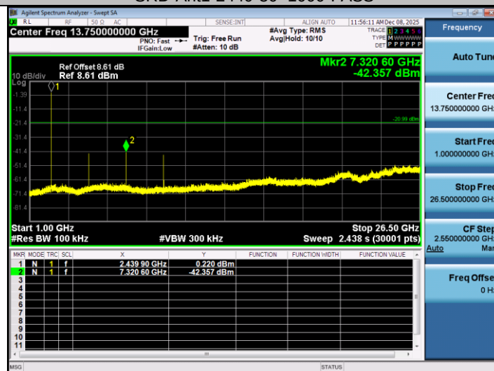
SRD-Ant1-2440-1000~26500-PASS
