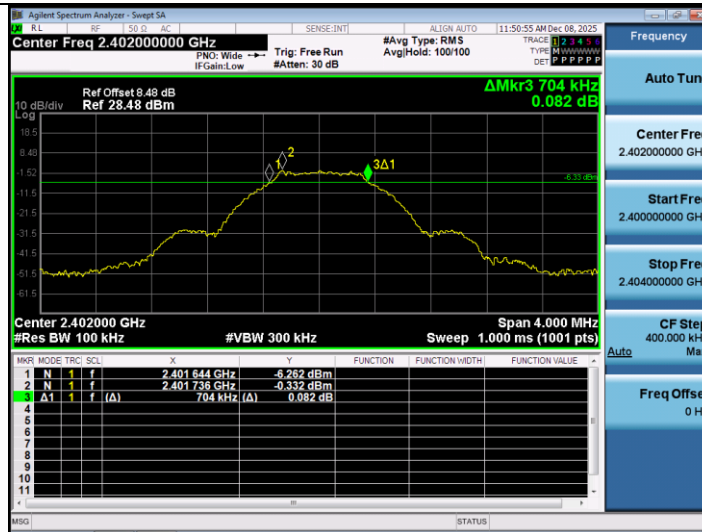
SRD-Ant1-2402-PASS
