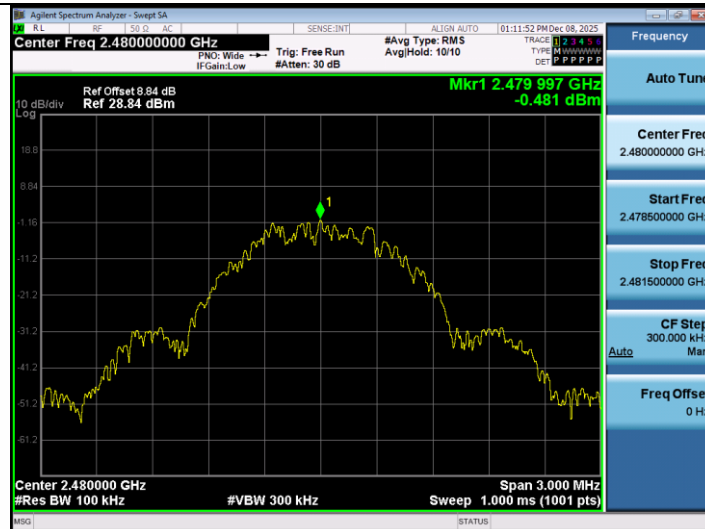
SRD-Ant1-2480-0~Reference-PASS
