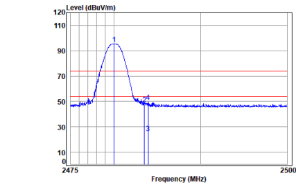
BT_DH5_TX_CH_78_Horizontal
