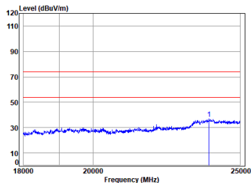
BT_TX_CH_M_Horizontal
