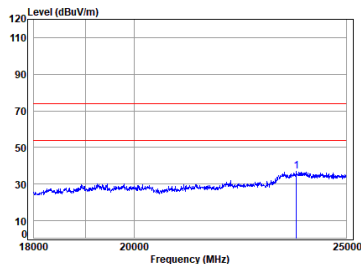
BT_TX_CH_M_Vertical
