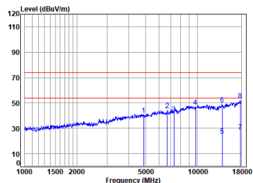
BT_DH5_TX_CH_39_Vertical
