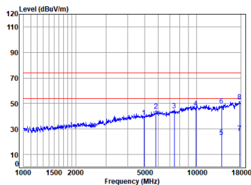
BT_DH5_TX_CH_78_Vertical
