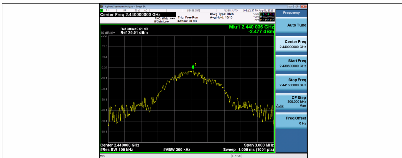
BLE_1M-Ant1-2440-0-Reference-PASS
