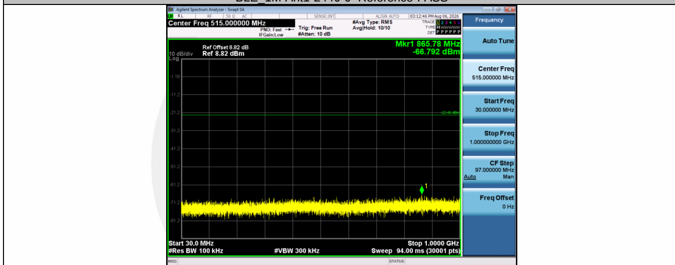
BLE_1M-Ant1-2440-30-1000-PASS
