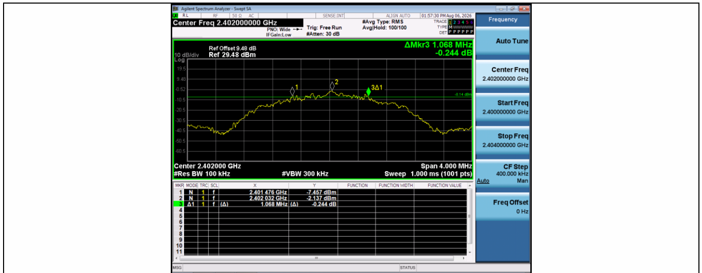
BLE_2M-Ant1-2402-PASS
