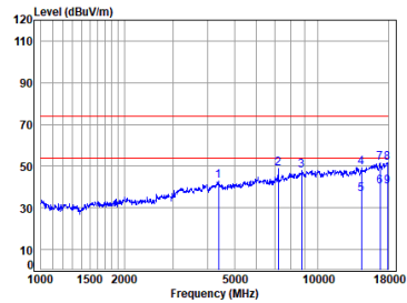
2.4G SRD_TX_CH_00_Vertical
