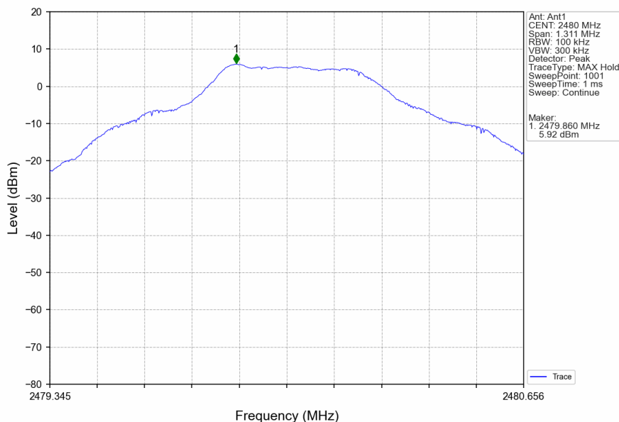
2.4G_HCH_2480MHz_Ant1_NTNV
