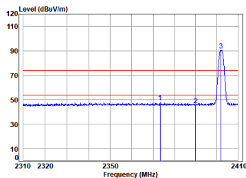
2.4G SRD_TX_CH_00_Vertical
