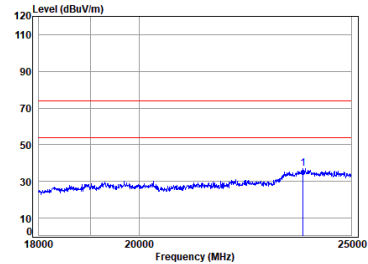
2.4G SRD_TX_CH_00_Vertical
