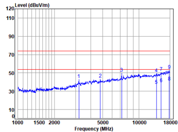
BLE_2M_TX_CH_00_Vertical
