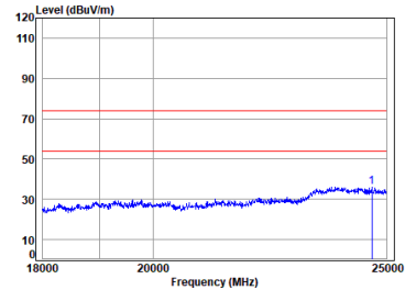
BLE_1M_TX_CH_00_Vertical
