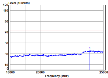
BLE_1M_TX_CH_19_Horizontal
