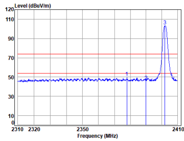
BLE_1M_TX_CH_00_Horizontal
