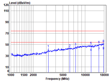
BLE_1M_TX_CH_39_Vertical
