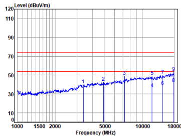
BLE_2M_TX_CH_00_Horizontal
