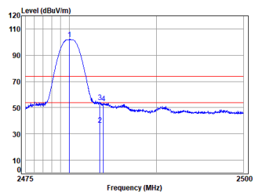
BLE_1M_TX_CH_39_Vertical
