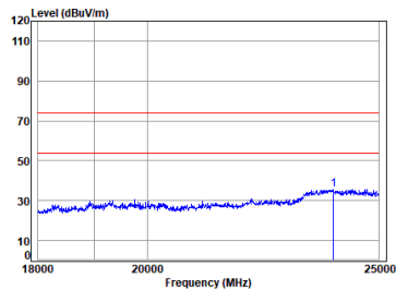
BLE_2M_TX_CH_00_Horizontal
