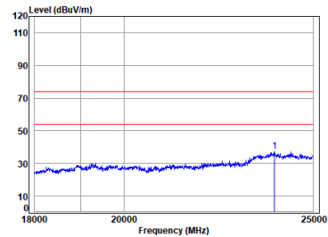
BLE_2M_TX_CH_19_Vertical
