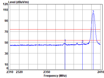
BLE_2M_TX_CH_00_Horizontal
