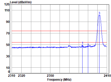
BLE_2M_TX_CH_00_Vertical
