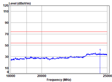
BLE_1M_TX_CH_39_Horizontal
