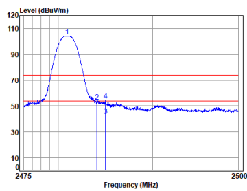
BLE_1M_TX_CH_39_Horizontal
