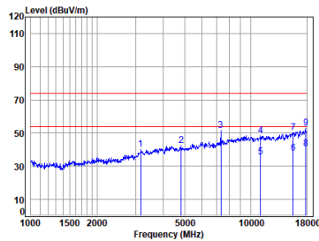
BLE_1M_TX_CH_19_Horizontal
