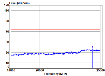
BLE_1M_TX_CH_39_Vertical
