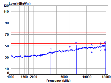
BLE_1M_TX_CH_19_Vertical
