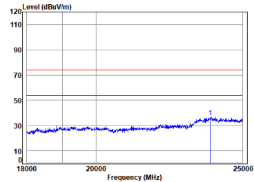
BLE_1M_TX_CH_19_Vertical
