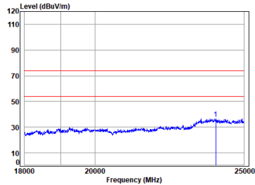
BLE_1M_TX_CH_00_Horizontal
