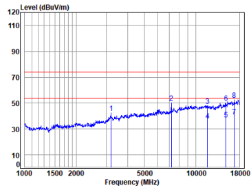
BLE_1M_TX_CH_00_Vertical
