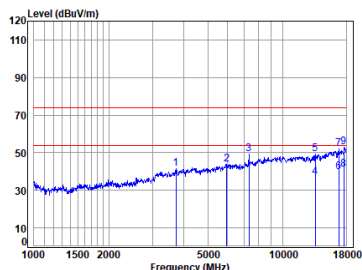
BLE_2M_TX_CH_19_Horizontal
