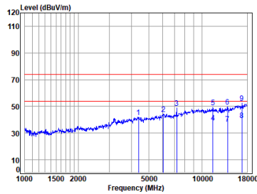
BLE_1M_TX_CH_00_Horizontal
