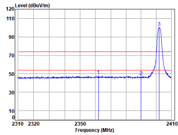
BLE_1M_TX_CH_00_Vertical
