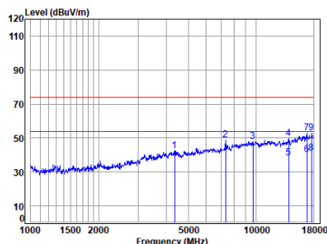
BLE_2M_TX_CH_19_Vertical
