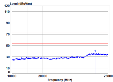
BLE_2M_TX_CH_00_Vertical
