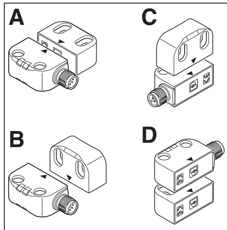
Figure 2-4 Actuation positions
