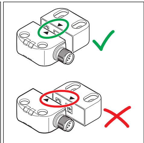
Figure 2-5 Center offset when safety equipment is closed
