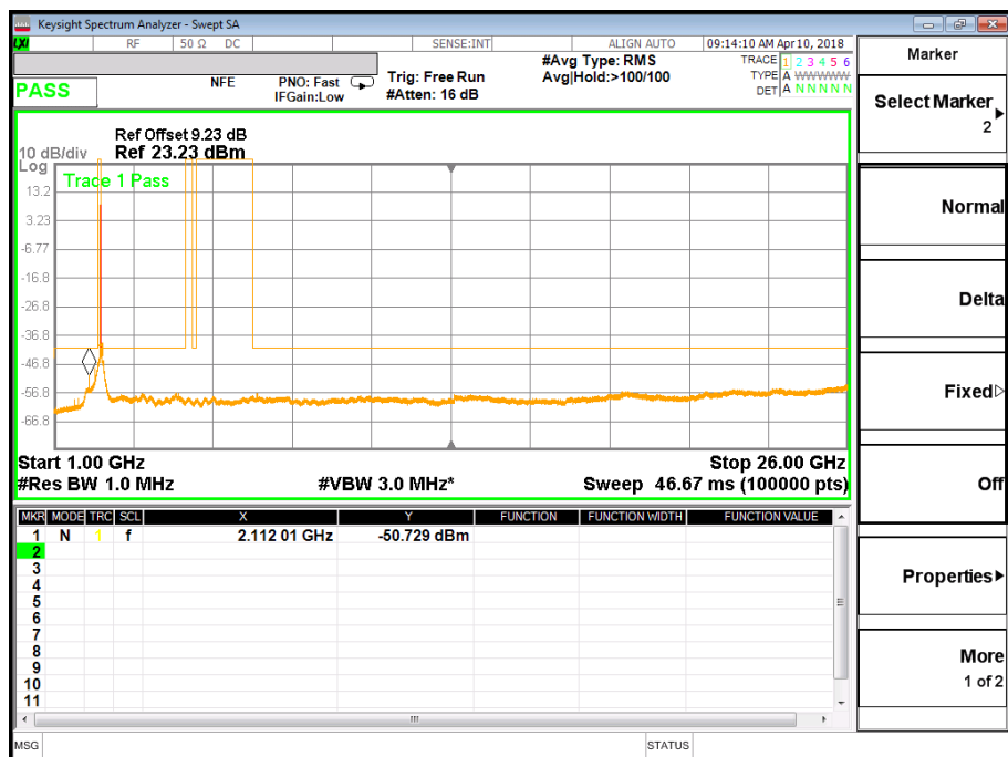
Plot 8: Highest channel / 1GHz to 26GHz / Antenna port 0
