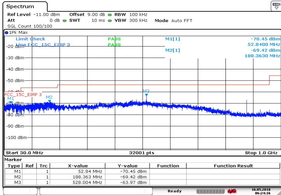
Plot 4: Middle channel / 30MHz to 1GHz / Antenna port 0
