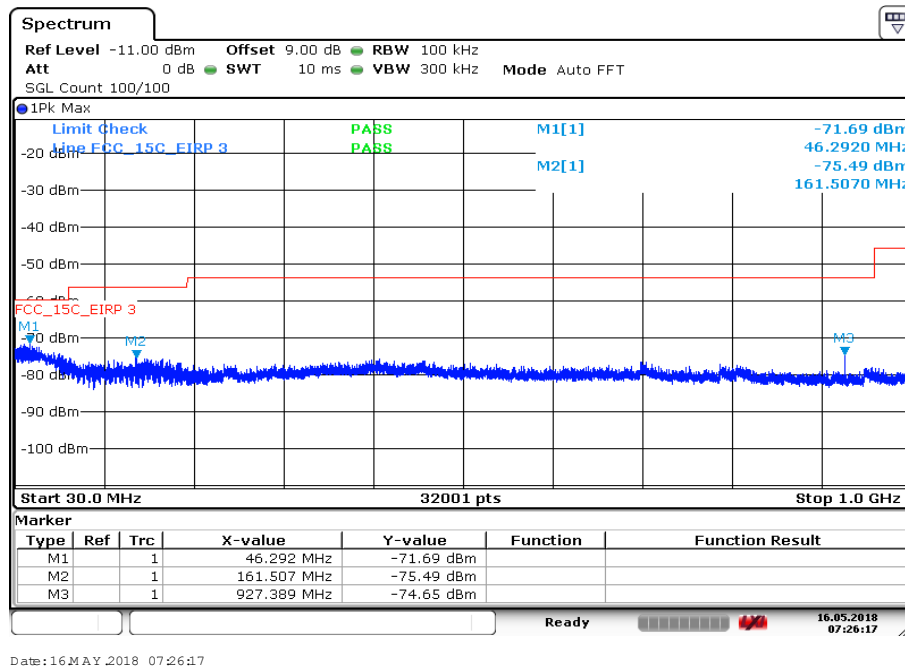
Plot 37: 30 MHz to 1 GHz, U-NII-3; middle channel
