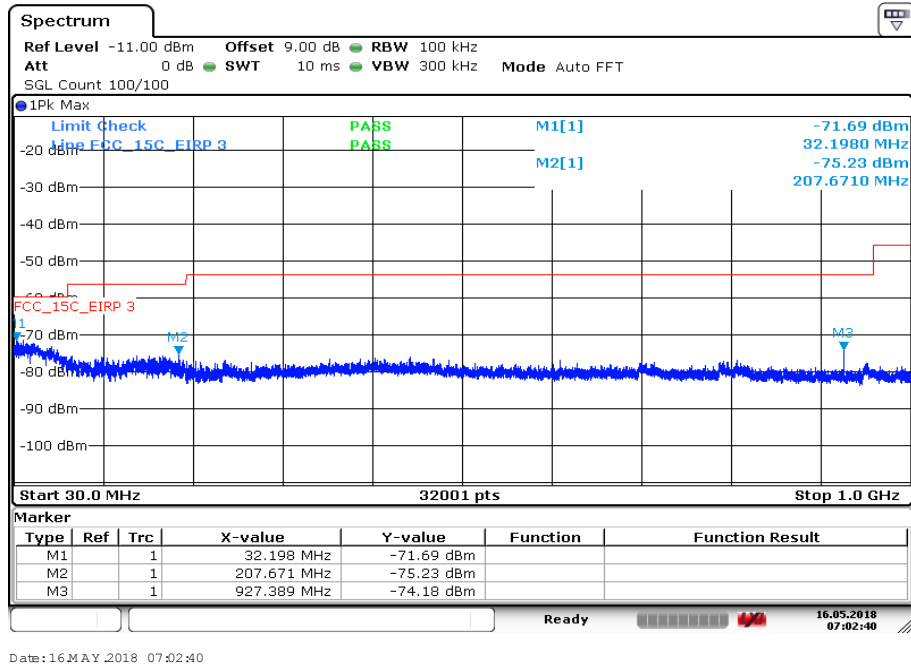
Plot 49: 30 MHz to 1 GHz, U-NII-3; highest channel
