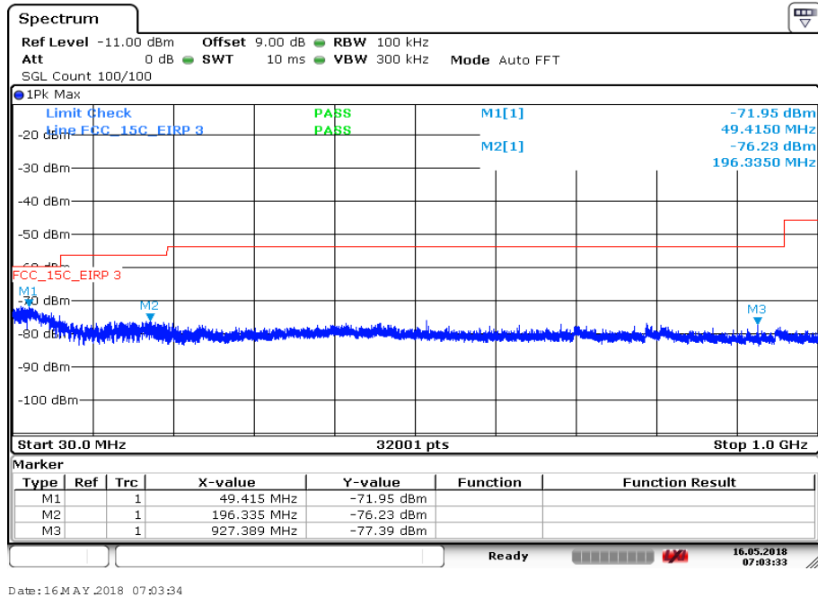
Plot 47: 30 MHz to 1 GHz, U-NII-3; lowest channel
