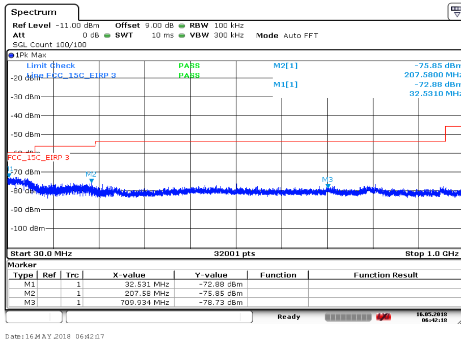
Plot 12: 30 MHz to 1 GHz, U-NII-3; middle channel
