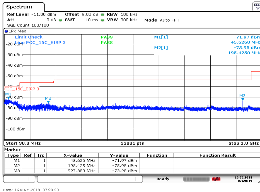
Plot 29: 30 MHz to 1 GHz, U-NII-1; middle channel
