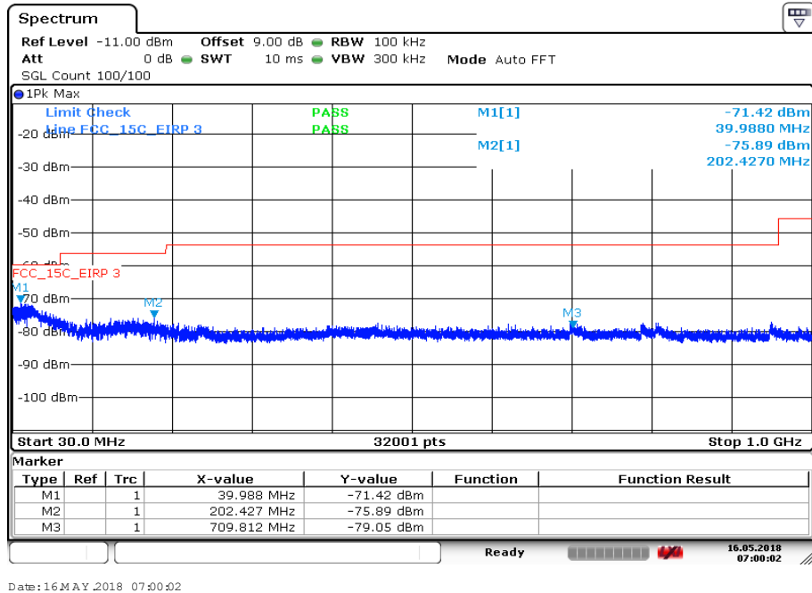
Plot 22: 30 MHz to 1 GHz, U-NII-3; lowest channel
