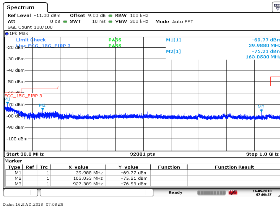
Plot 44: 30 MHz to 1 GHz, U-NII-1; highest channel
