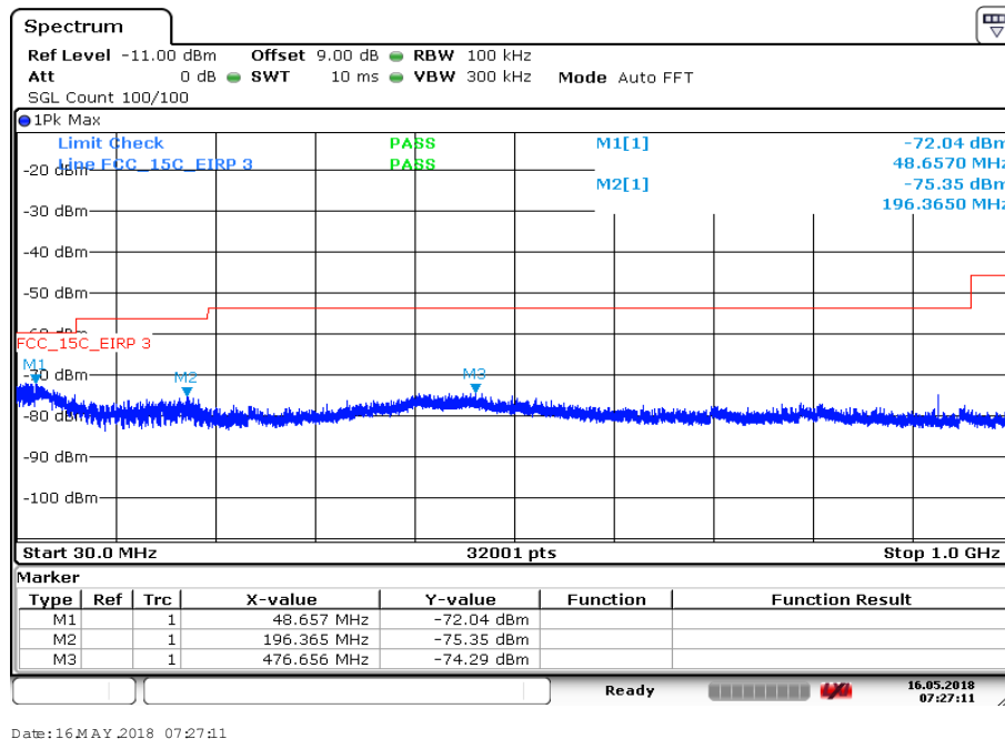
Plot 39: 30 MHz to 1 GHz, U-NII-3; highest channel
