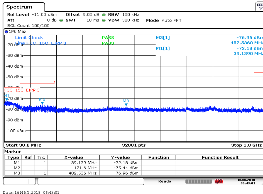
Plot 14: 30 MHz to 1 GHz, U-NII-3; highest channel
