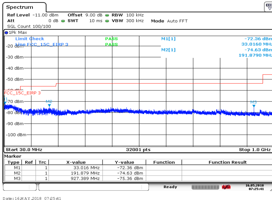
Plot 35: 30 MHz to 1 GHz, U-NII-3; lowest channel
