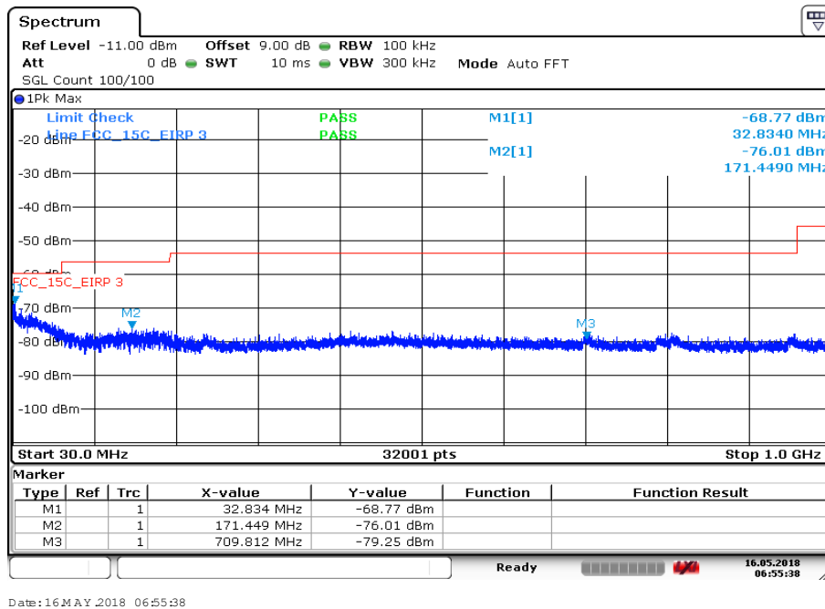
Plot 19: 30 MHz to 1 GHz, U-NII-1; highest channel
