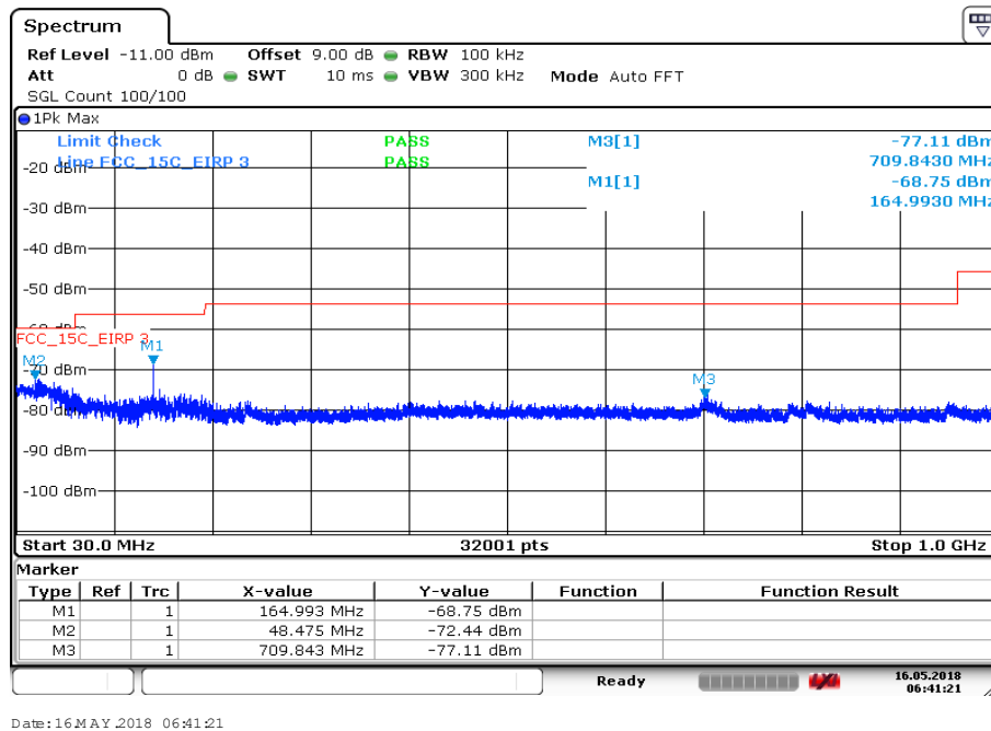
Plot 10: 30 MHz to 1 GHz, U-NII-3; lowest channel
