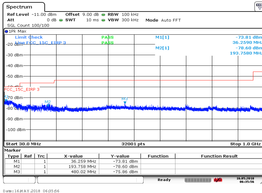
Plot 4: 30 MHz to 1 GHz, U-NII-1; middle channel
