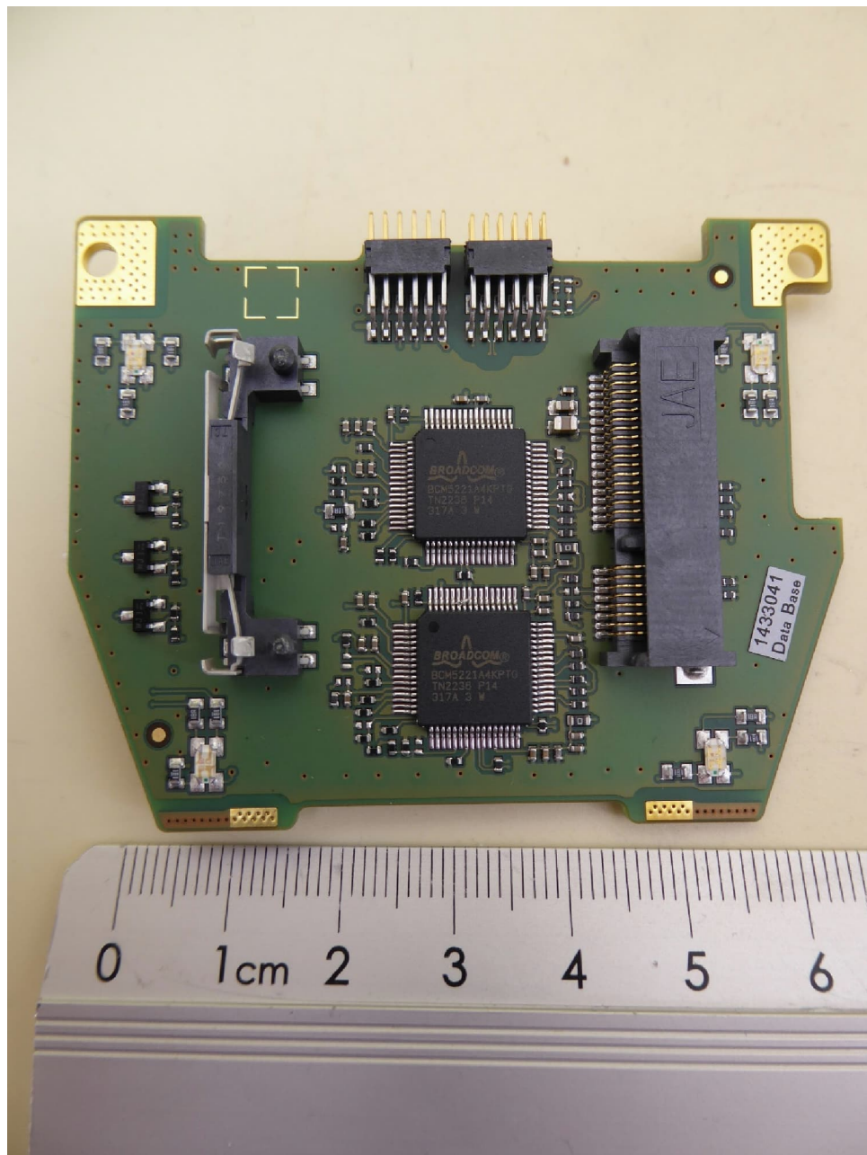
NEARFI 2000 B, data PCB, top view
