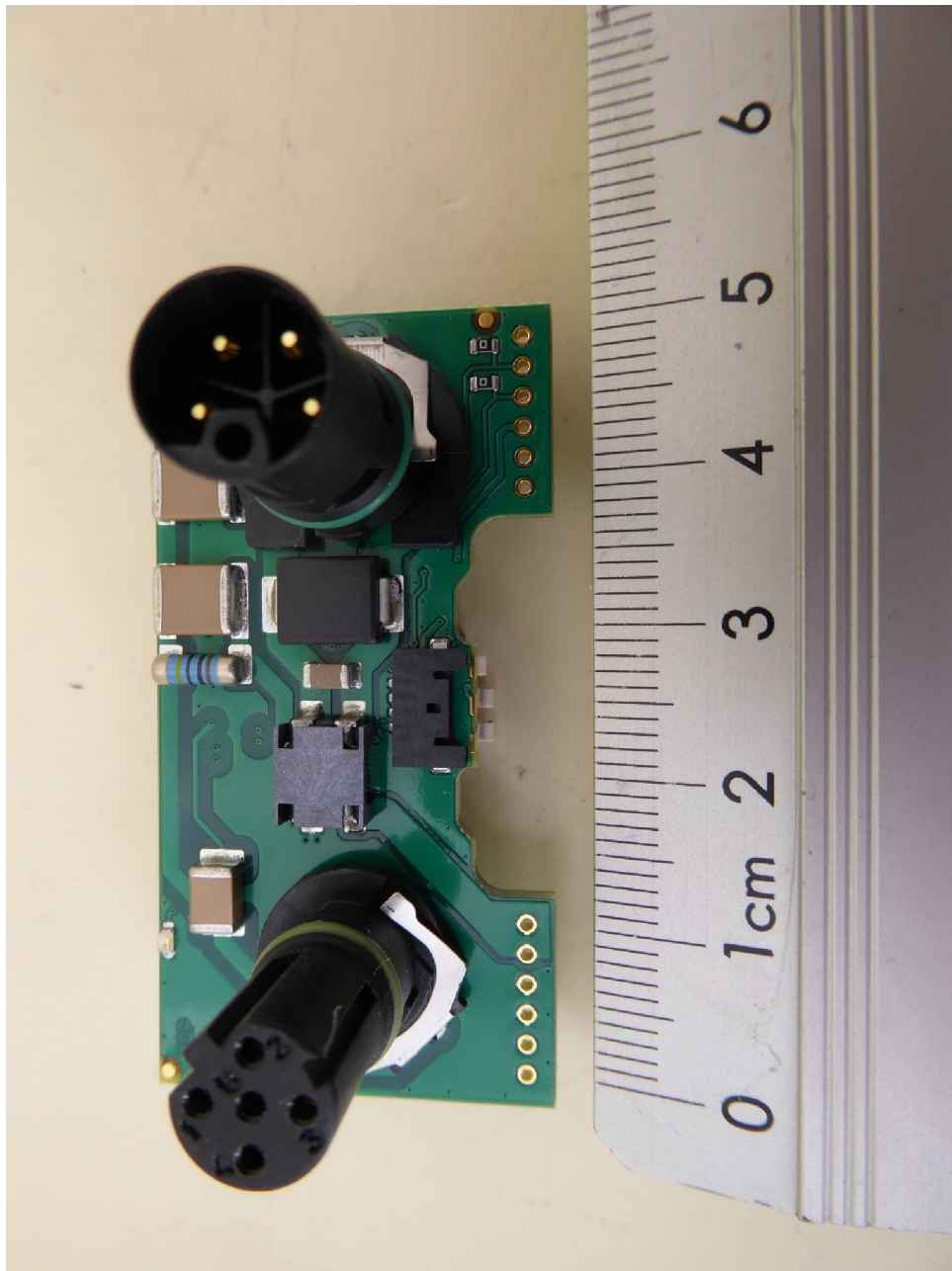
NEARFI 2000 B, interface PCB, top view
