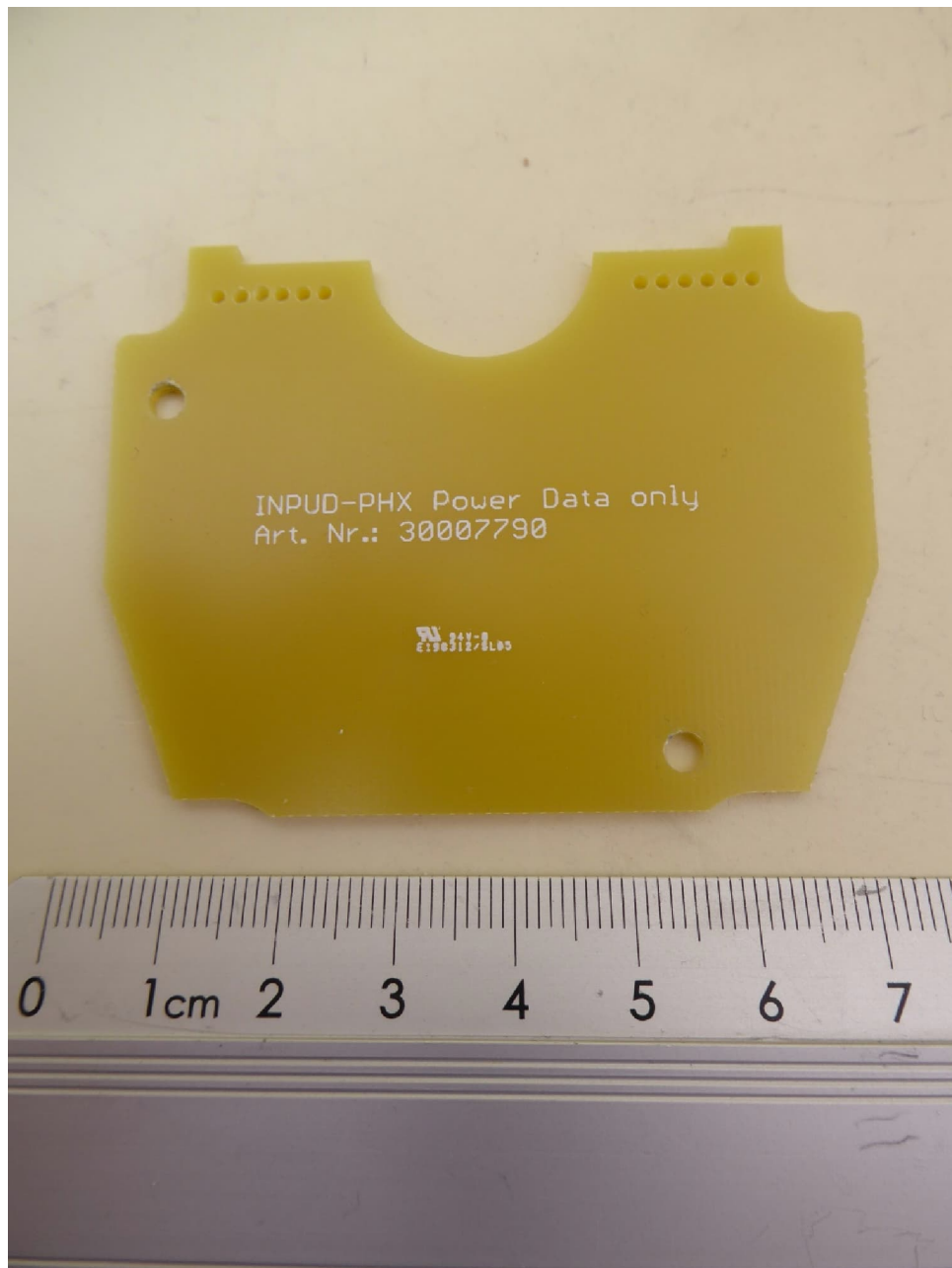
NEARFI 2000 B, dummy PCB, top view
