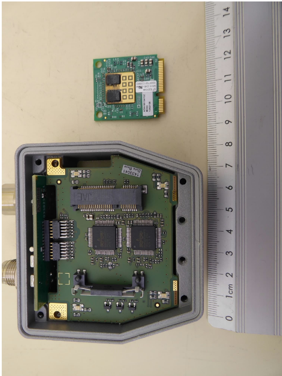
NEARFI 2000 B, internal view 3, RF-PCB removed
