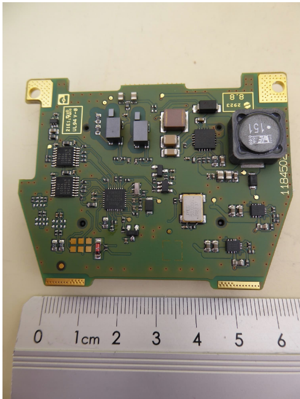
NEARFI 2000 B, data PCB, bottom view
