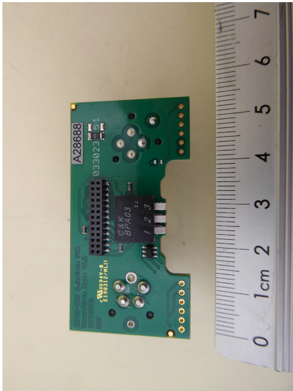
NEARFI 2000 B, interface PCB, bottom view
