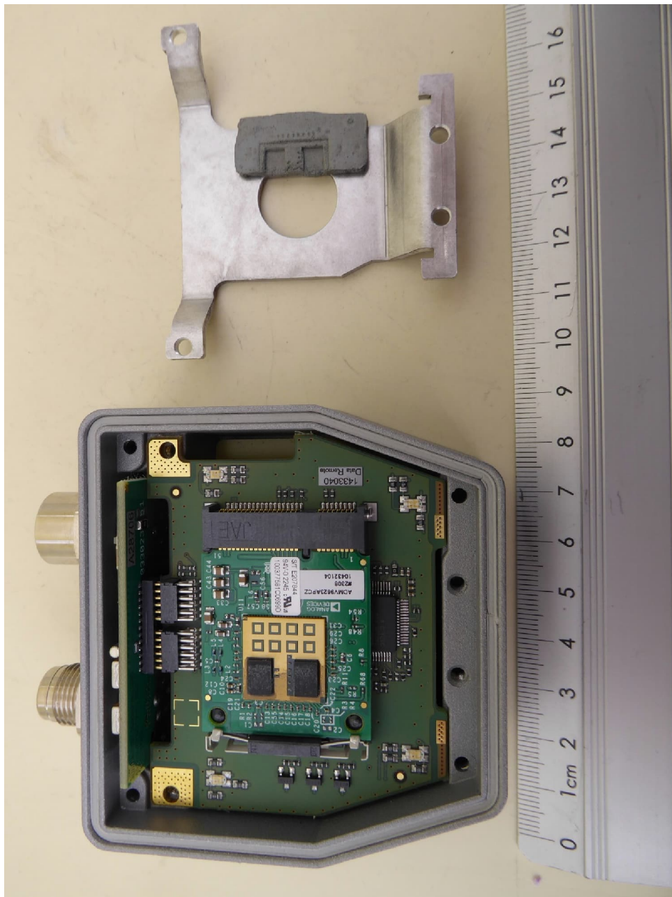
NEARFI 2000 R, internal view 2, shielding removed
