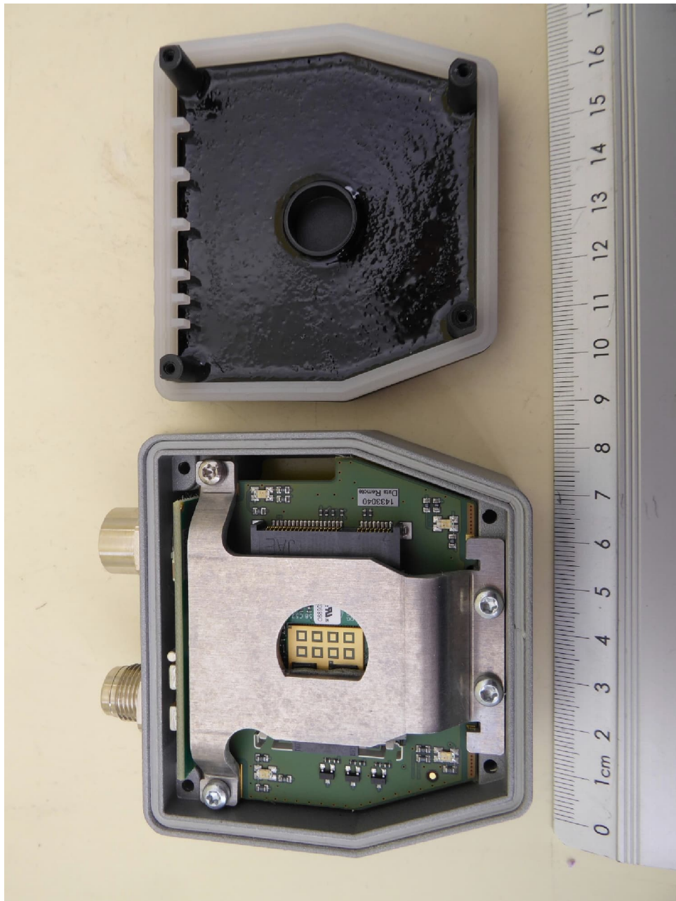
NEARFI 2000 R, internal view 1, housing opened
