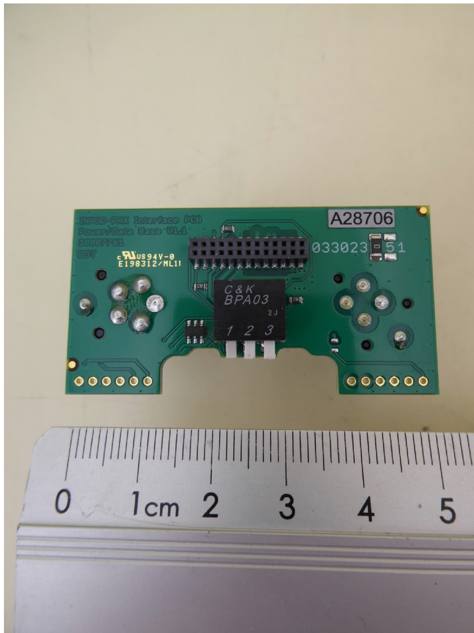
NEARFI 2000 R, interface PCB, bottom view
