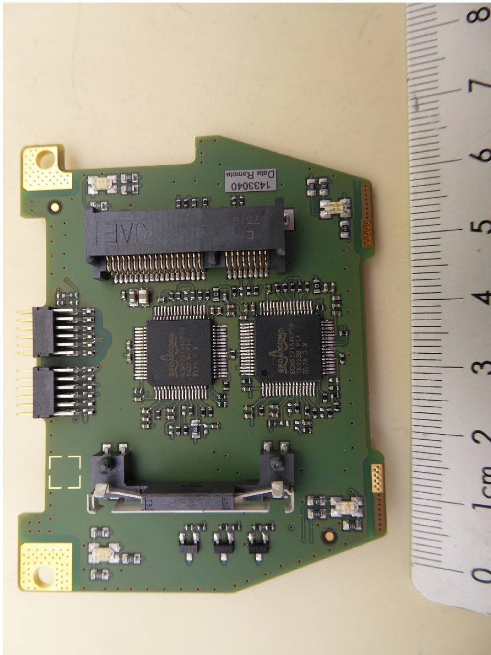
NEARFI 2000 R, data PCB, top view
