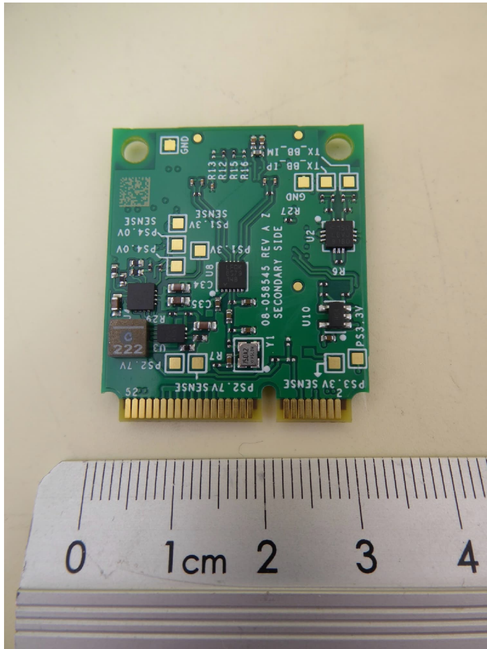
NEARFI 2000 R, RF-PCB, bottom view
