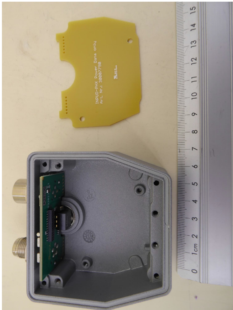
NEARFI 2000 R, internal view 5, dummy PCB removed
