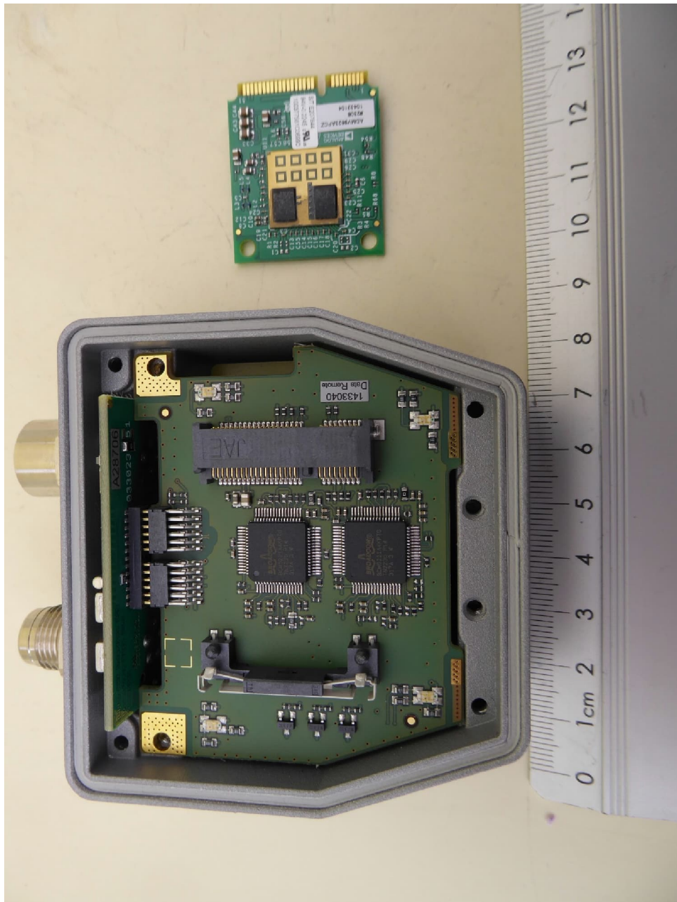
NEARFI 2000 R, internal view 3, RF-PCB removed
