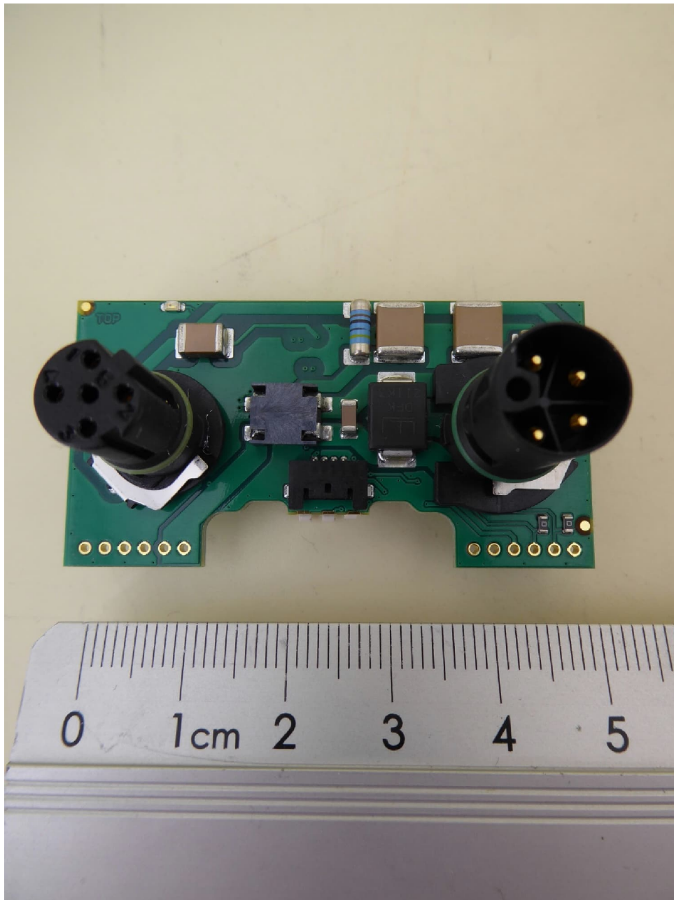
NEARFI 2000 R, interface PCB, top view
