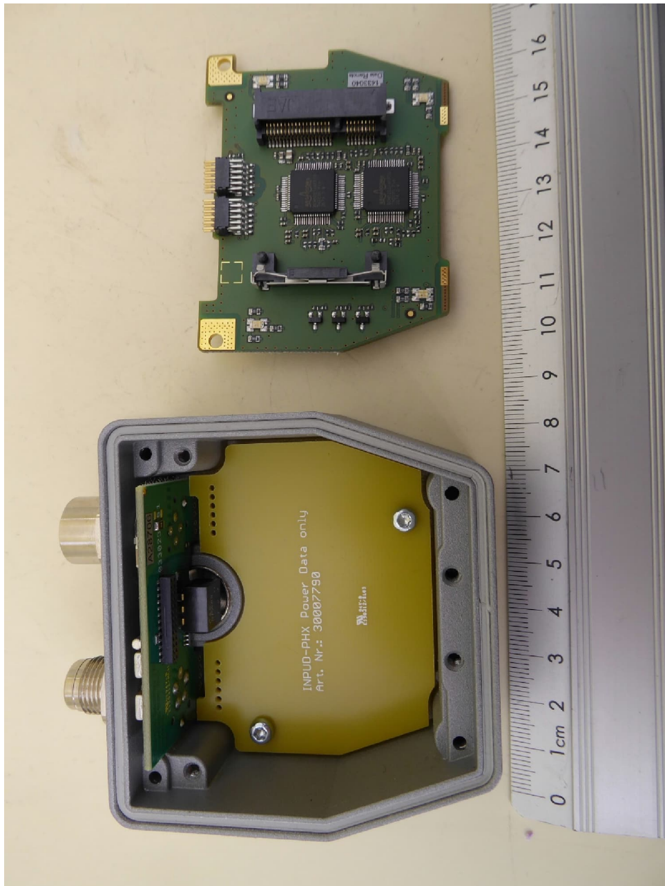
NEARFI 2000 R, internal view 4, data PCB removed
