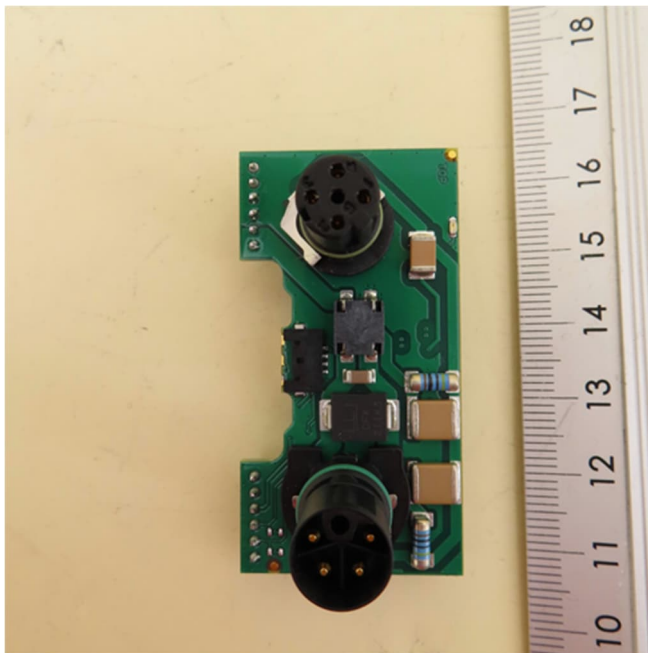
Interface PCB Bottom
