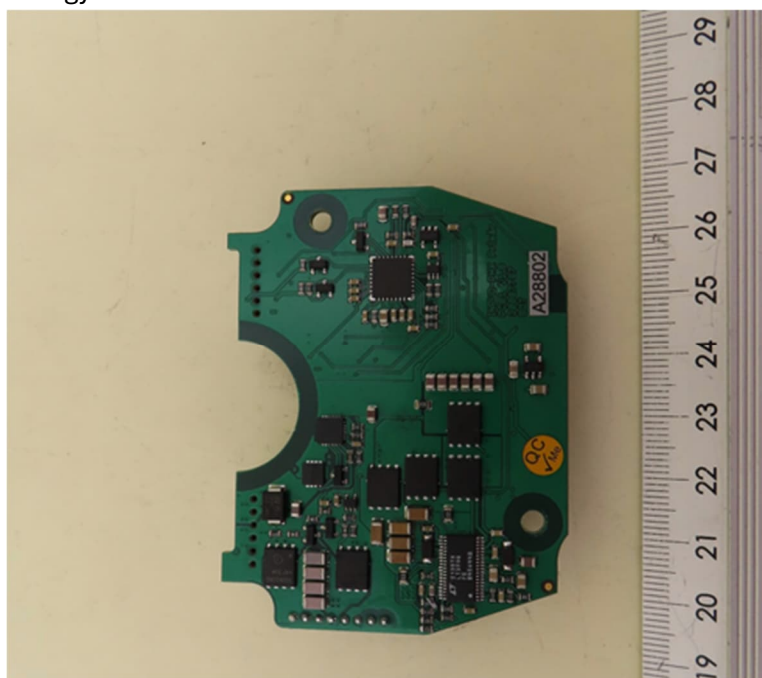
Energy PCB Bottom
