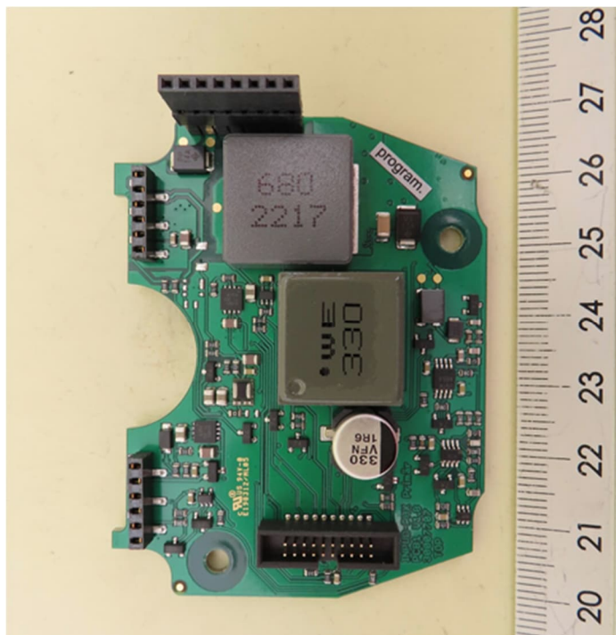
Energy PCB Top
