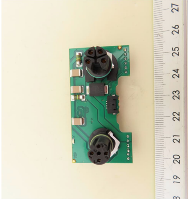
Interface PCB Bottom
