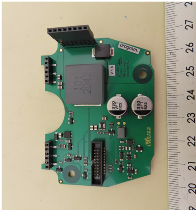
Energy PCB Bottom
