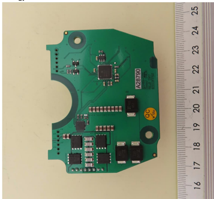
Energy PCB Bottom
