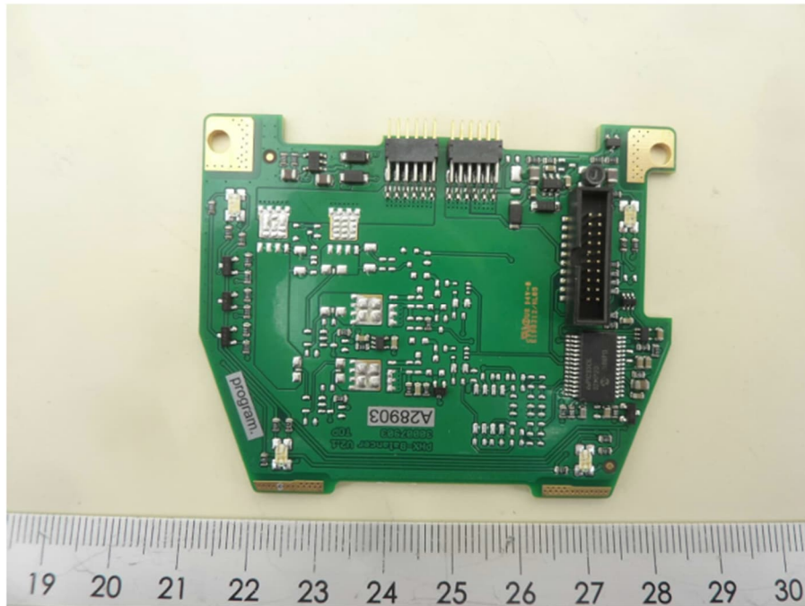
Balancer PCB Bottom
