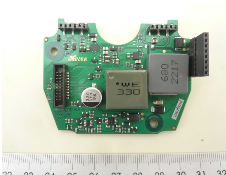
Energy PCB Top
