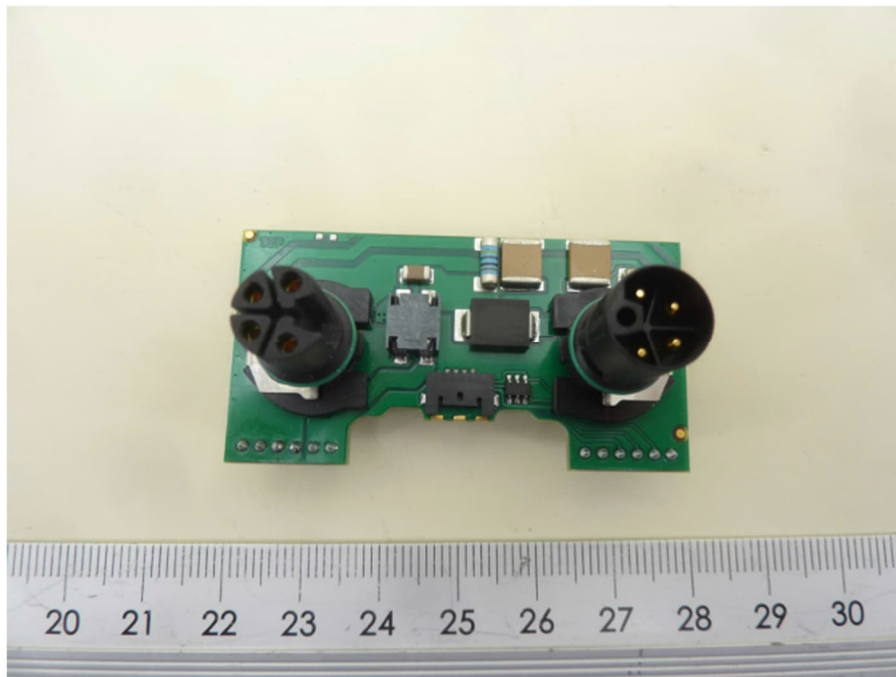
Interface PCB Top
