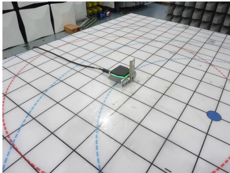
Test setup semi anechoic chamber (position 3)
