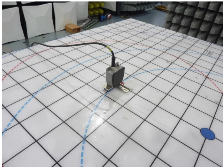
Test setup semi anechoic chamber (position 1)
