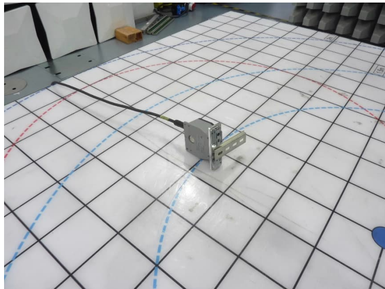
Test setup semi anechoic chamber (position 2)
