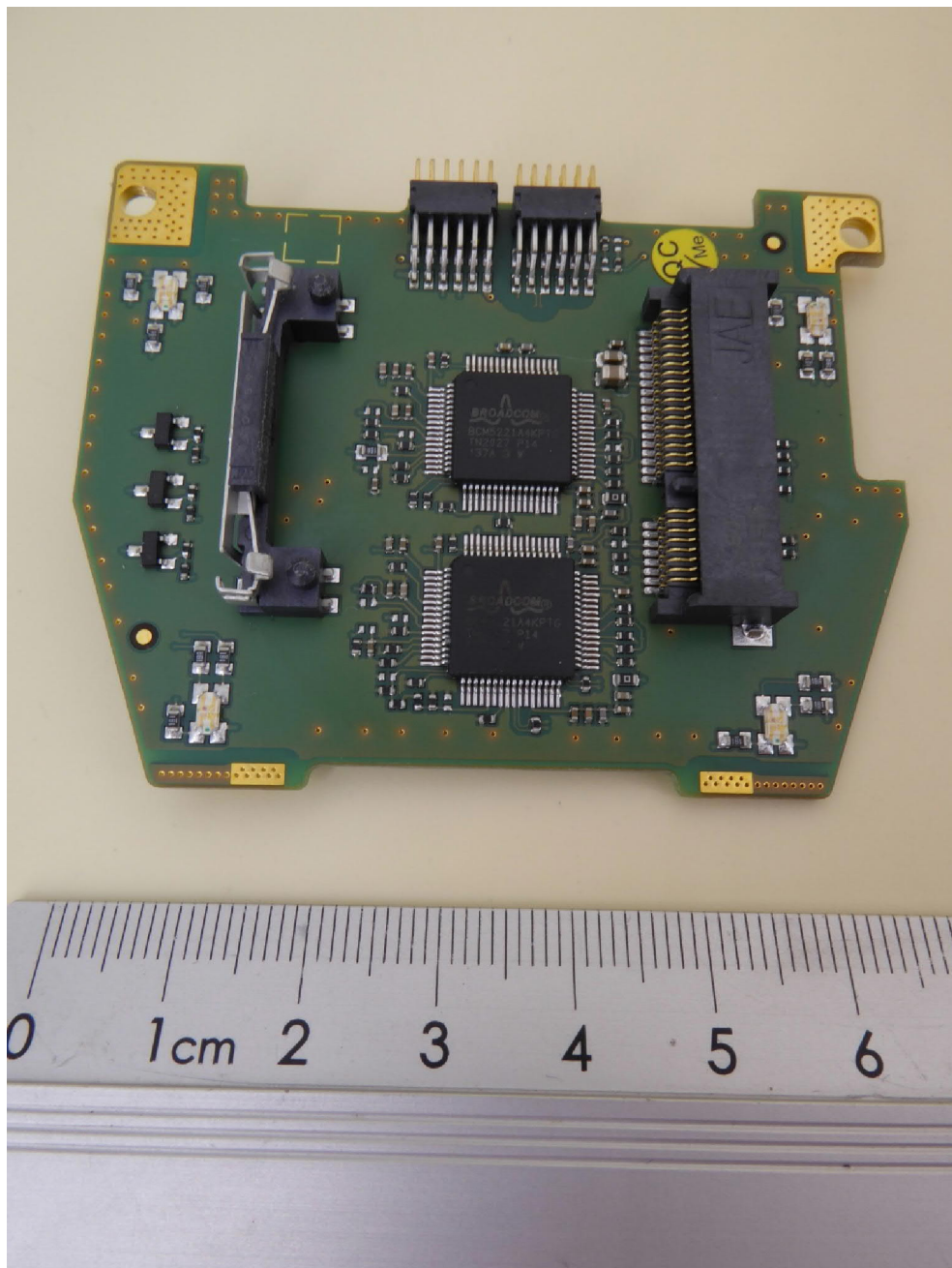
NEARFI D ETH B, data PCB, top view
