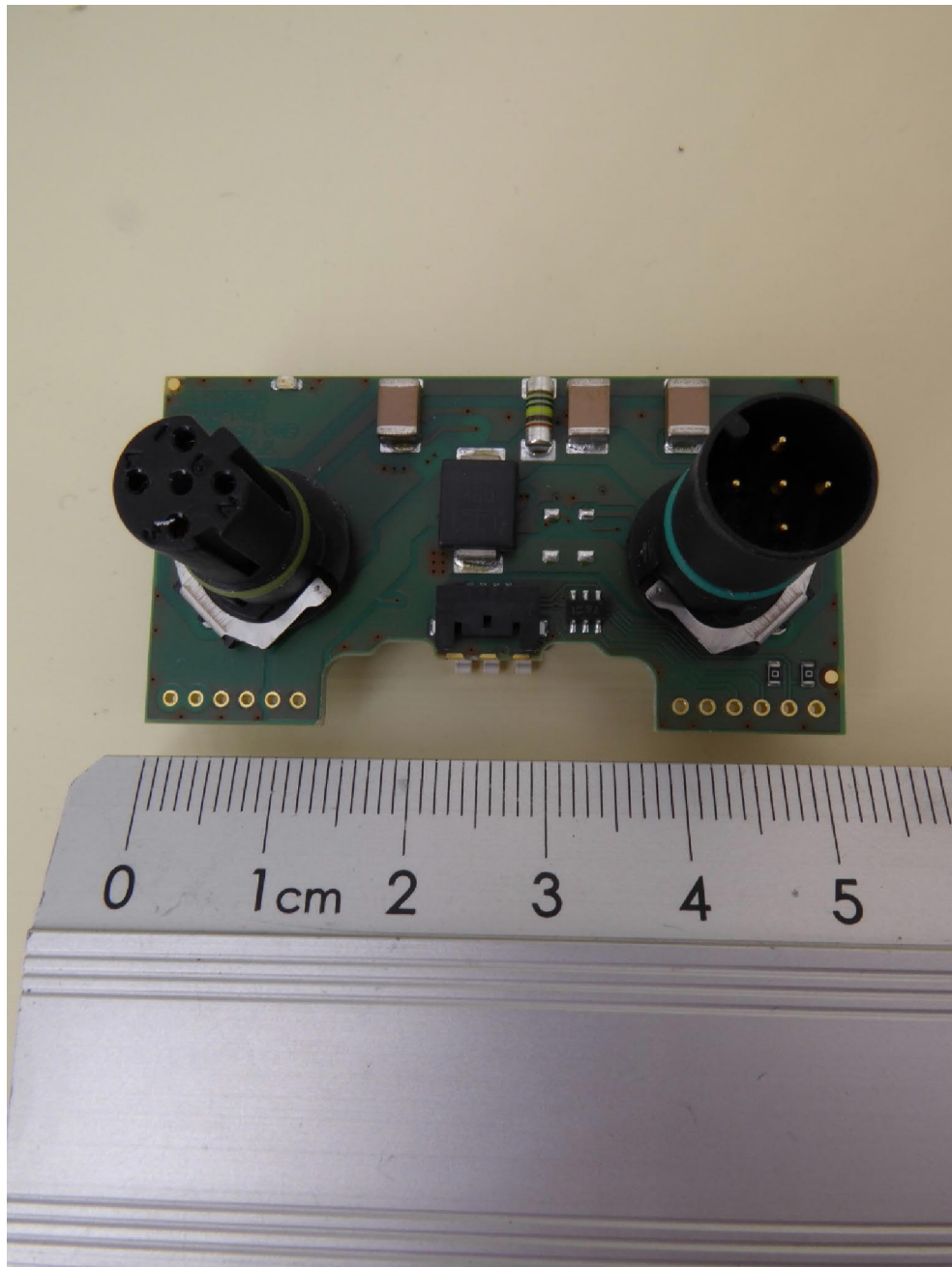
NEARFI D ETH B, interface PCB, top view
