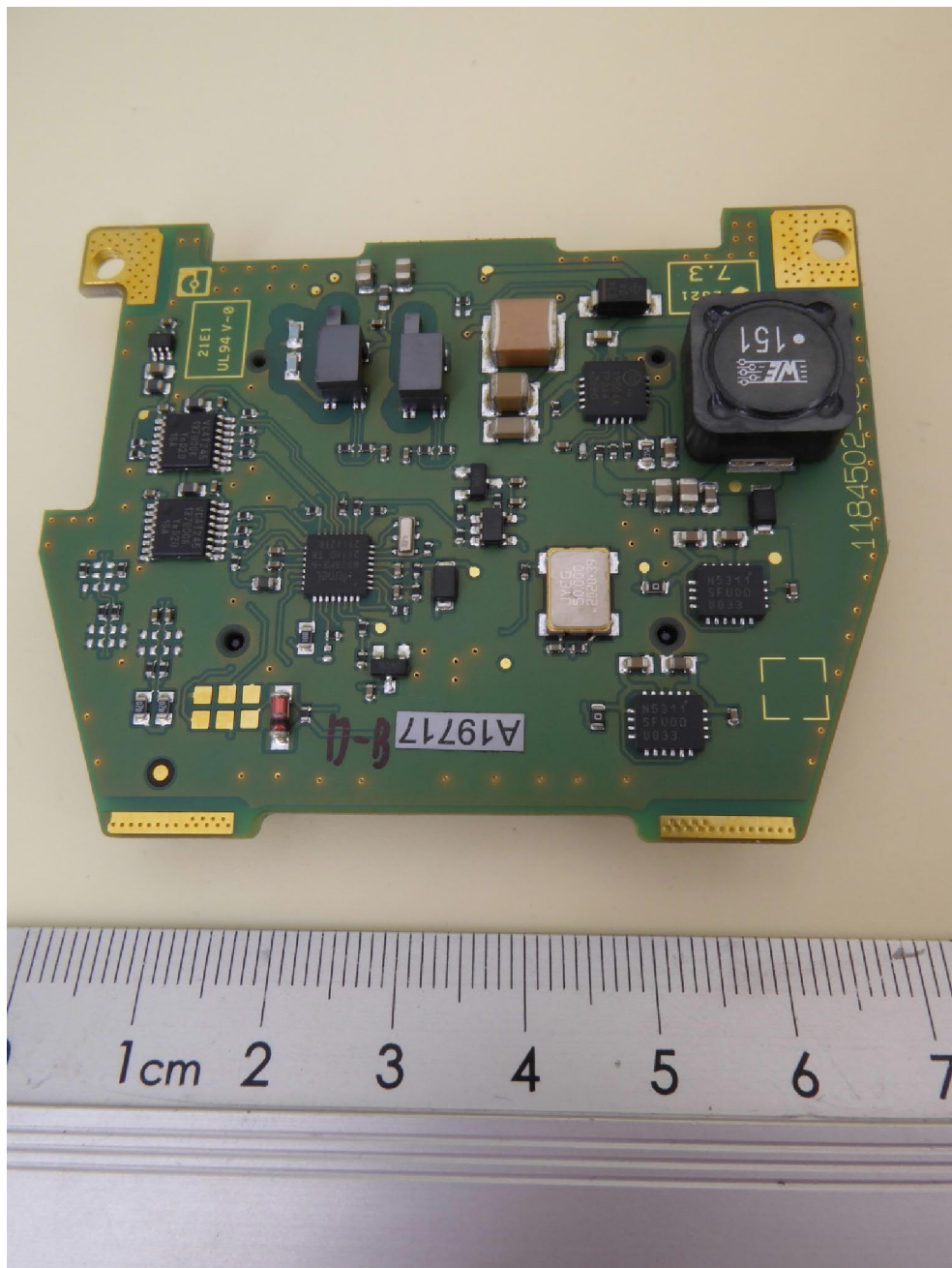
NEARFI D ETH B, data PCB, bottom view
