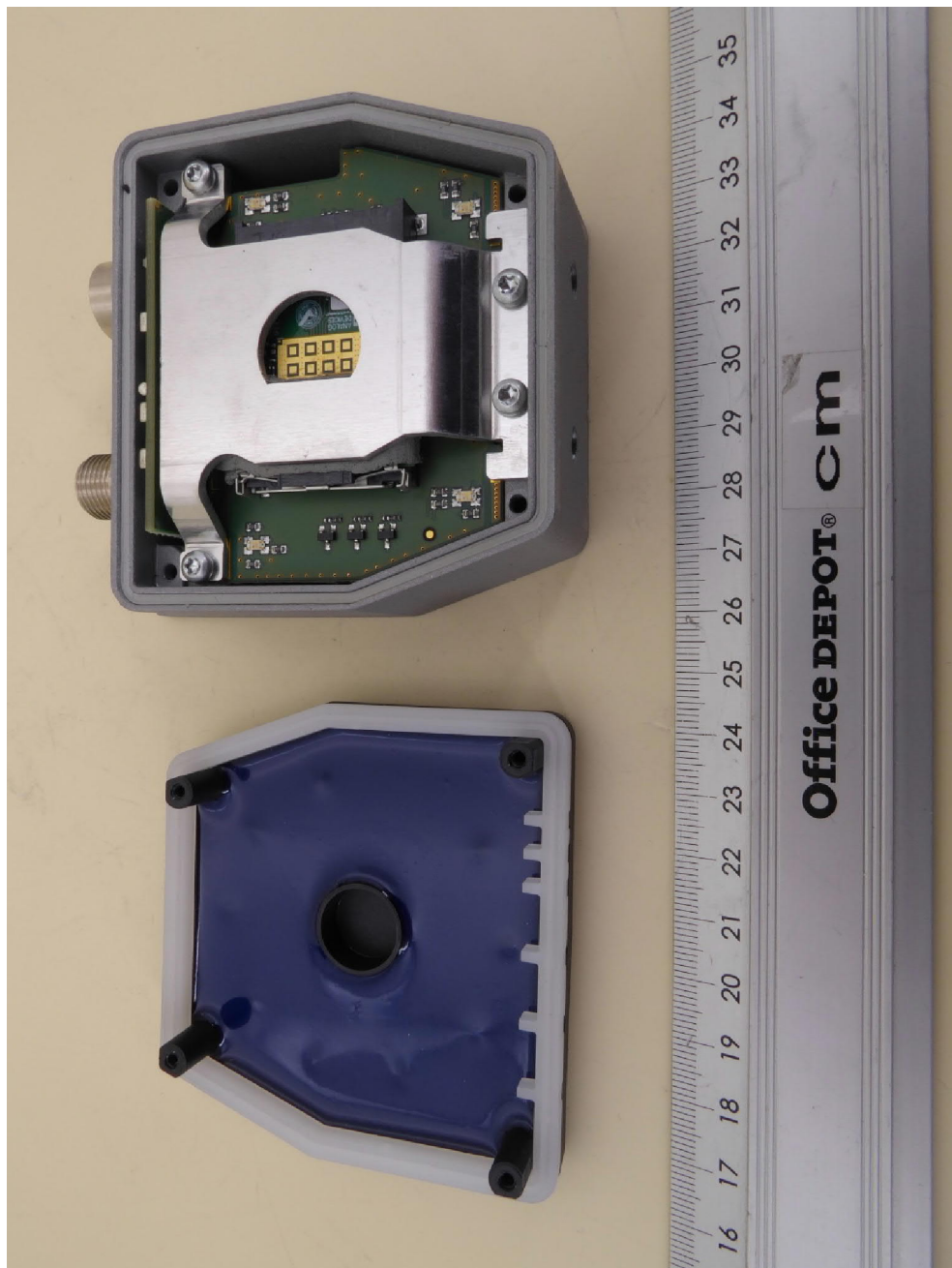
NEARFI D ETH B, internal view 1, housing opened
