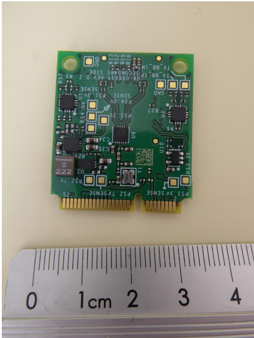
NEARFI D ETH B, RF-PCB, bottom view
