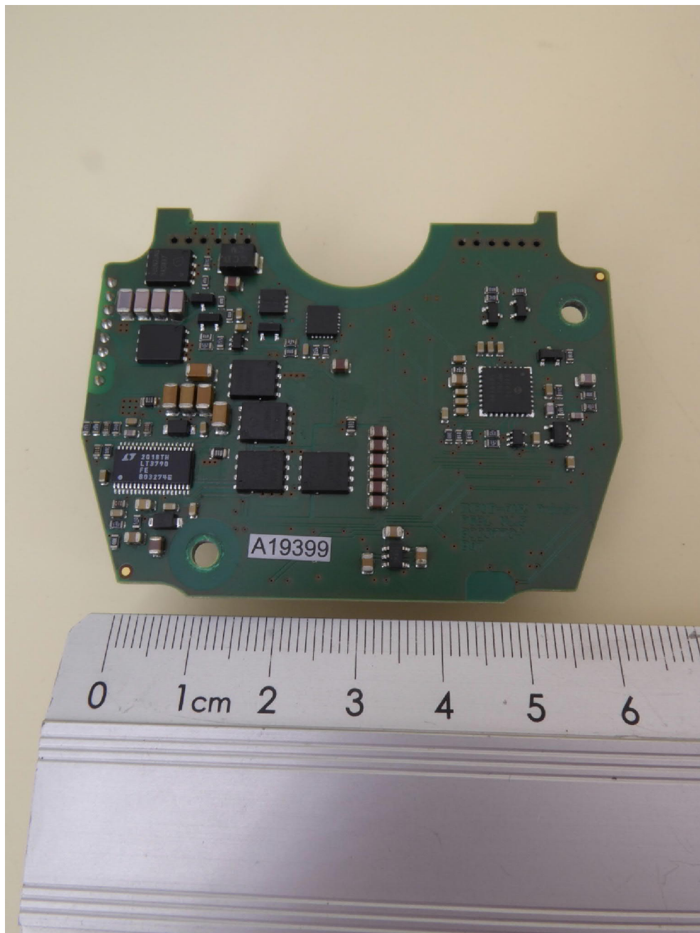
NEARFI PD 2A ETH B, energy PCB, bottom view
