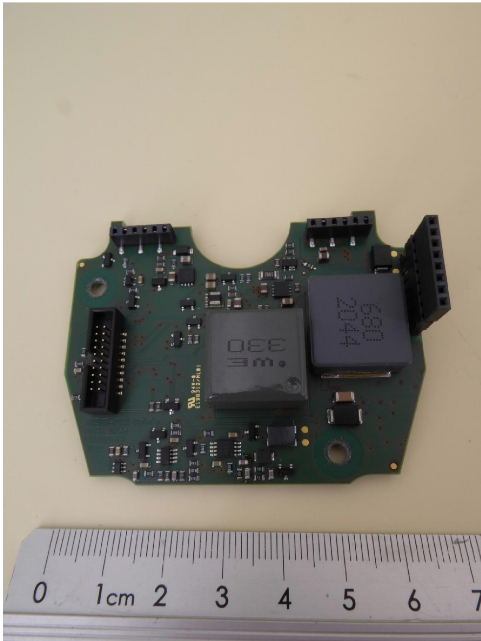
NEARFI PD 2A ETH B, energy PCB, top view
