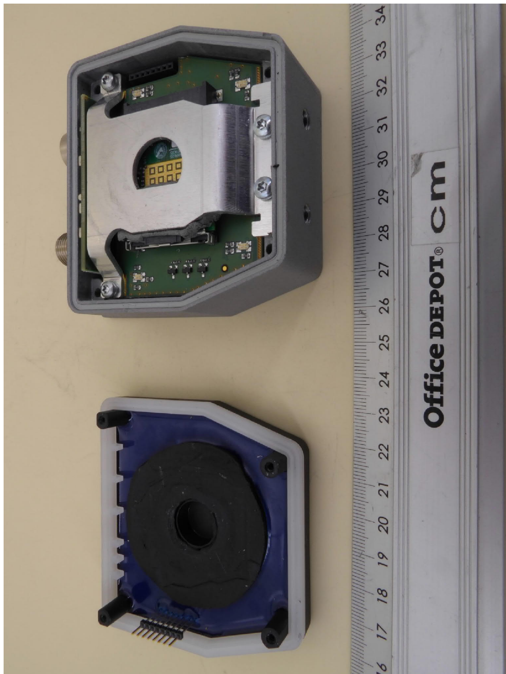
NEARFI PD 2A ETH B, internal view 1, housing opened
