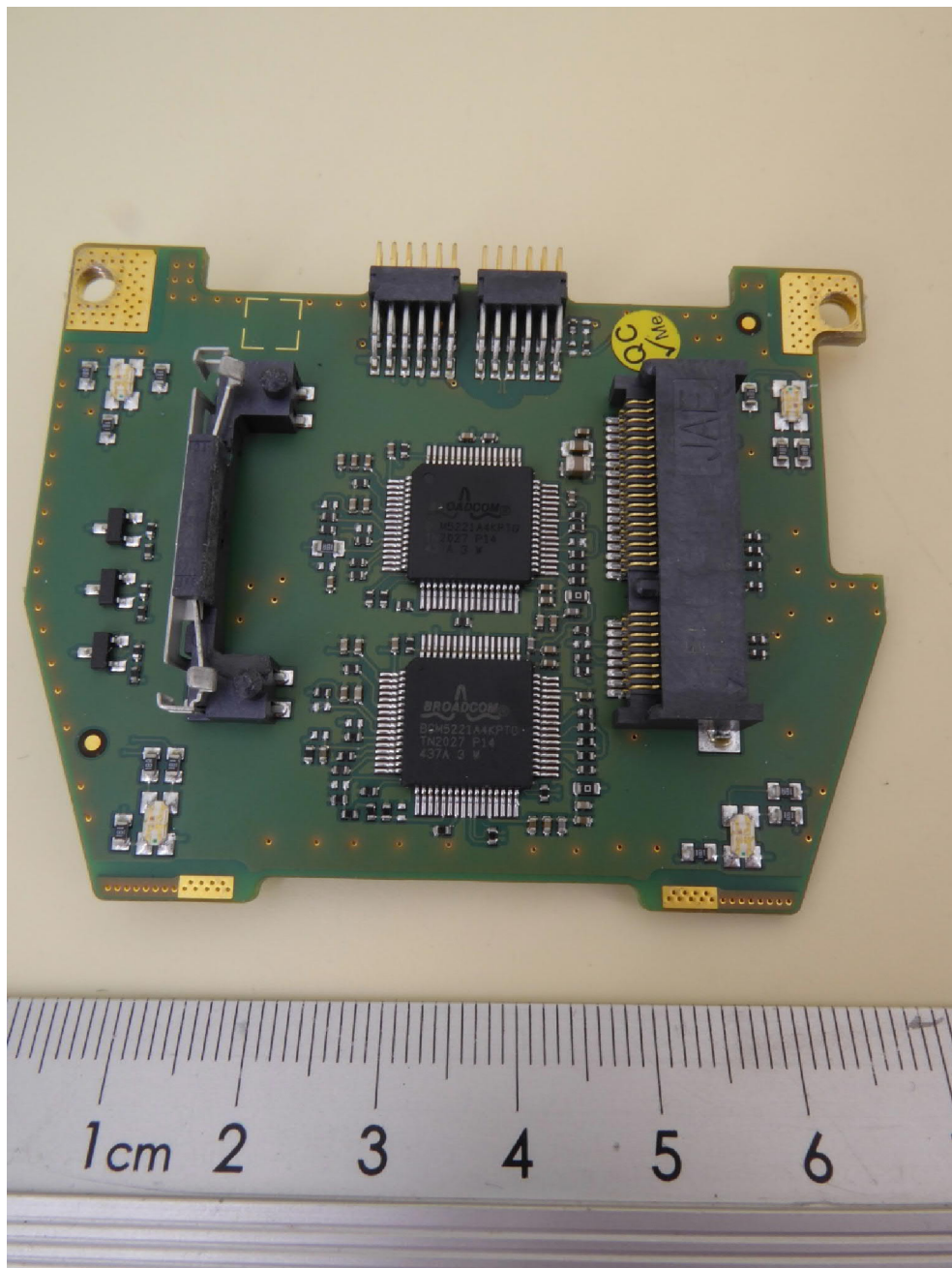
NEARFI PD 2A ETH B, data PCB, top view
