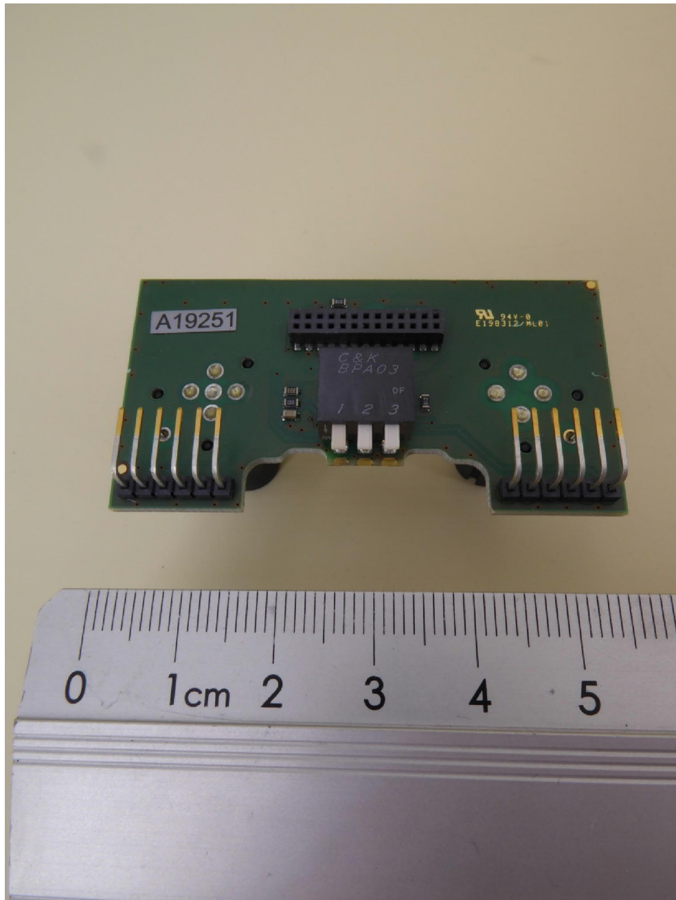
NEARFI PD 2A ETH B, interface PCB, bottom view
