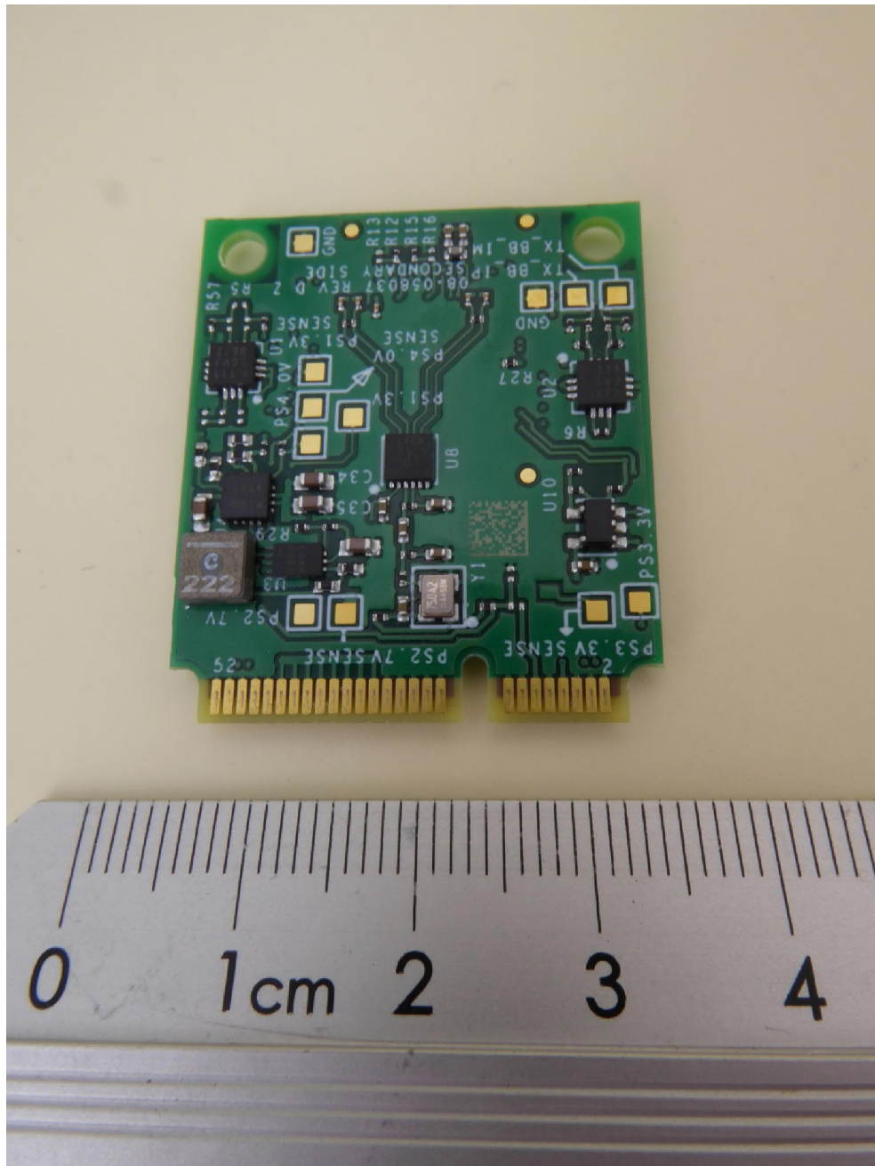
NEARFI PD 2A ETH B, RF-PCB, bottom view
