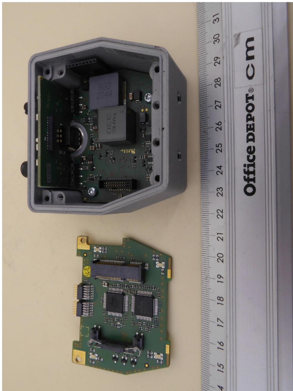
NEARFI PD 2A ETH B, internal view 4, data PCB removed
