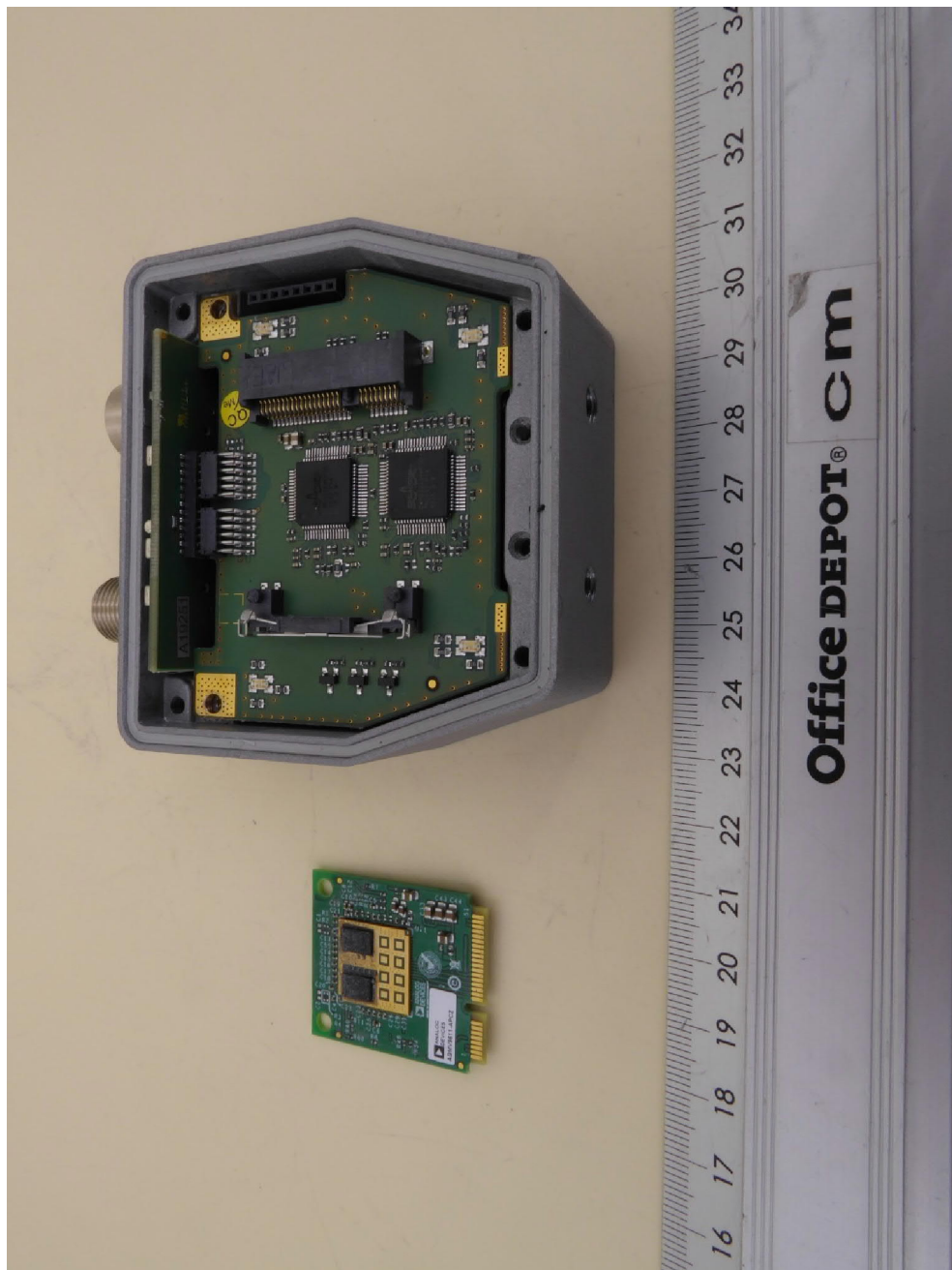
NEARFI PD 2A ETH B, internal view 3, RF-PCB removed
