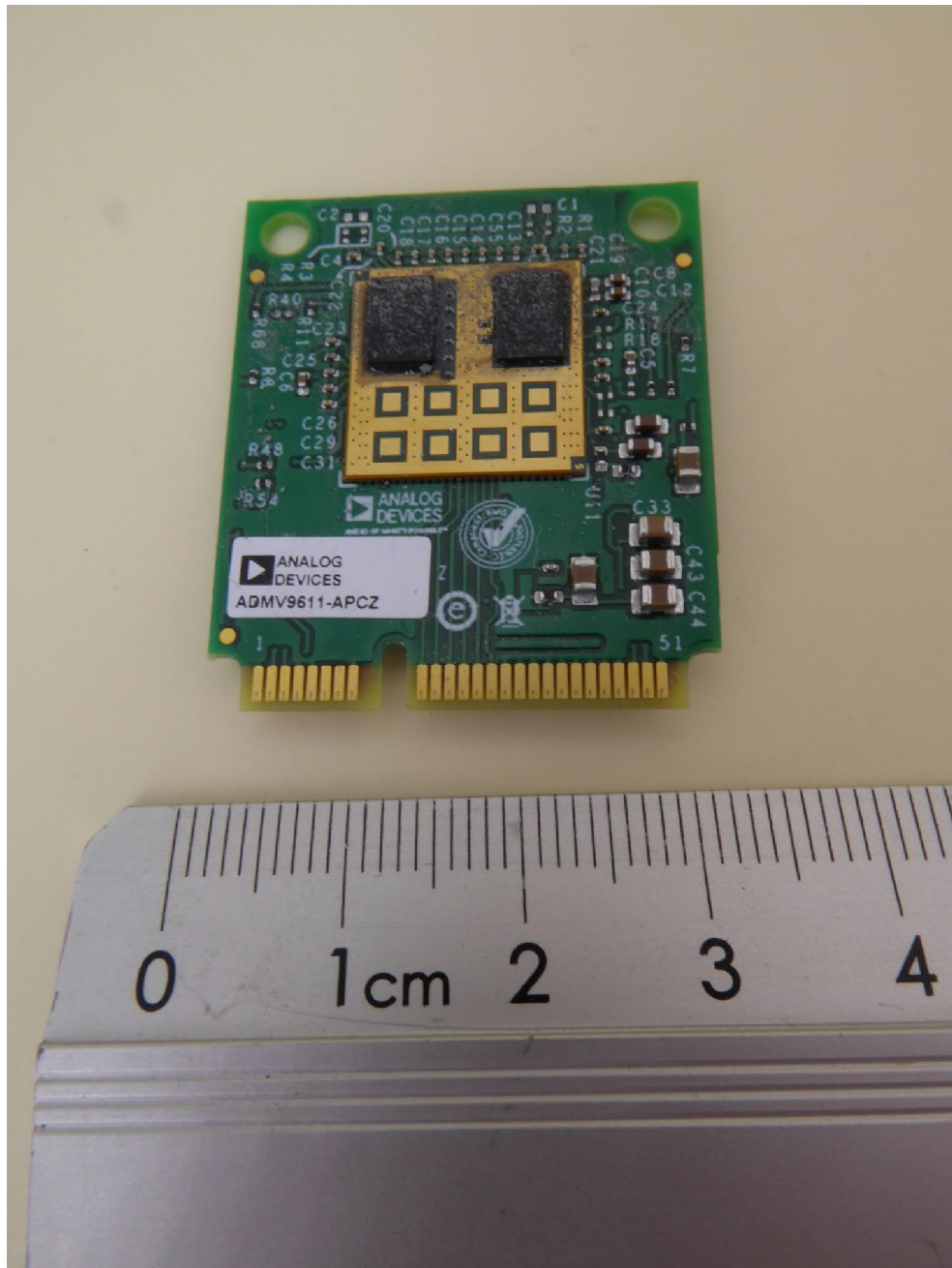
NEARFI PD 2A ETH B, RF-PCB, top view
