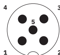
Figure 32 Power-IN (X1), M12 male, A-coded
