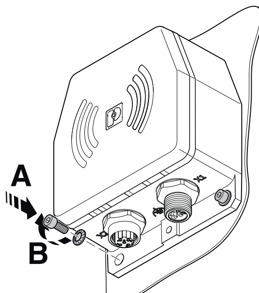
Figure 25 Mounting with two M5 screws
