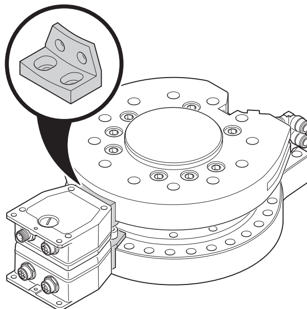
Figure 45 Installation example with external heatsink (machine head)
