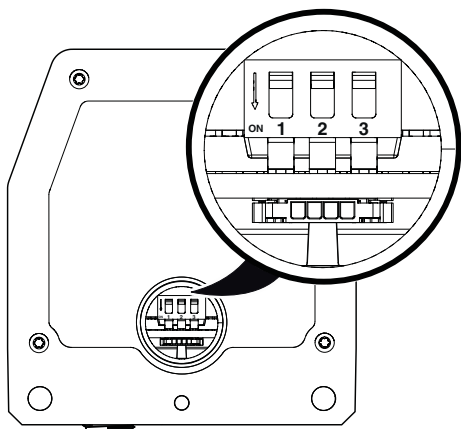
Figure 9 DIP switches
