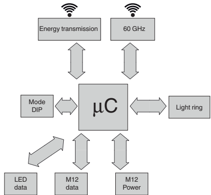
Figure 5 Basic circuit diagram of power and data couplers
