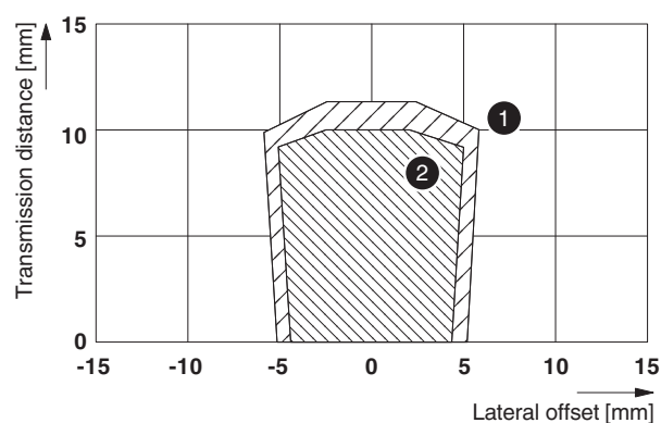
Figure 13 Transmission distance for lateral offset, NEARFI PD...
