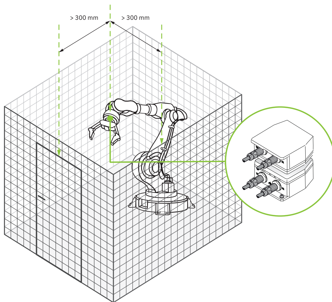
Figure 1 Industrial robots
