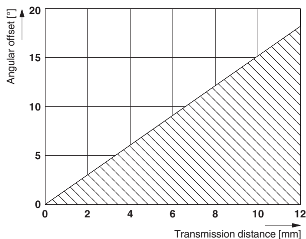
Figure 14 Transmission distance for angular offset, NEARFI PD...
