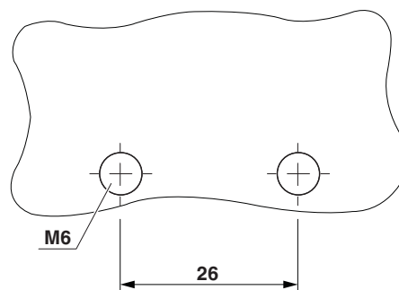
Figure 28 Drilling diagram
