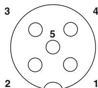
Figure 31 Power-OUT (X1), M12 female, A-coded
