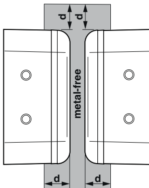
Figure 20 Metal-free area
