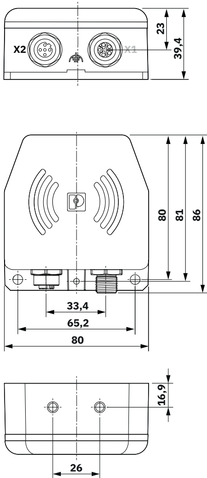
Figure 4 Housing dimensions
