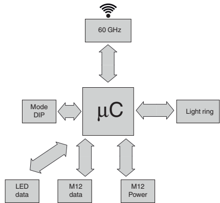
Figure 7 Basic circuit diagram of data coupler
