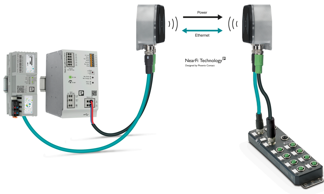
Figure 3 Example design for contact-free transmission of power and data between a controller and a decentral I/O device with Ethernet interface
