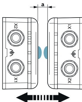
Figure 10 Transmission distance
