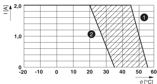
Figure 42 Derating curve
