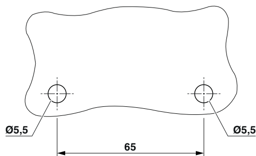
Figure 24 Drilling diagram
