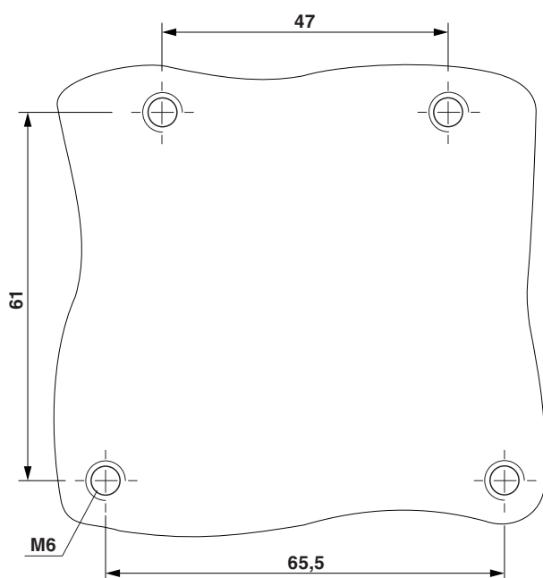
Figure 26 Drilling diagram
