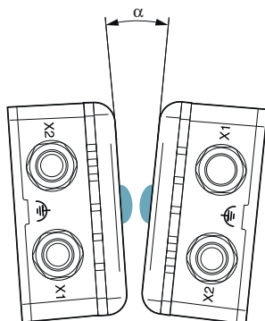
Figure 12 Angular offset
