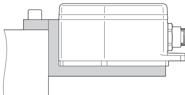
Figure 43 Optimal thermal connection
