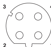
Figure 33 Data IN/OUT (X2), M12 female, D-coded
