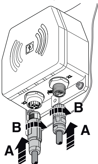
Figure 34 Connecting the cables
