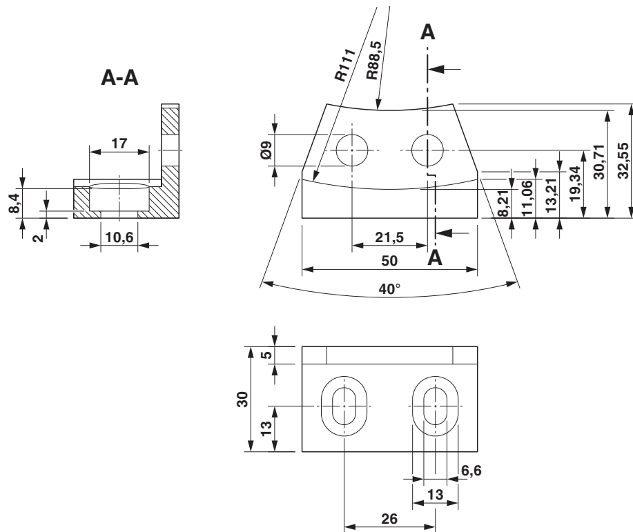
Figure 47 Dimensions of adapter
