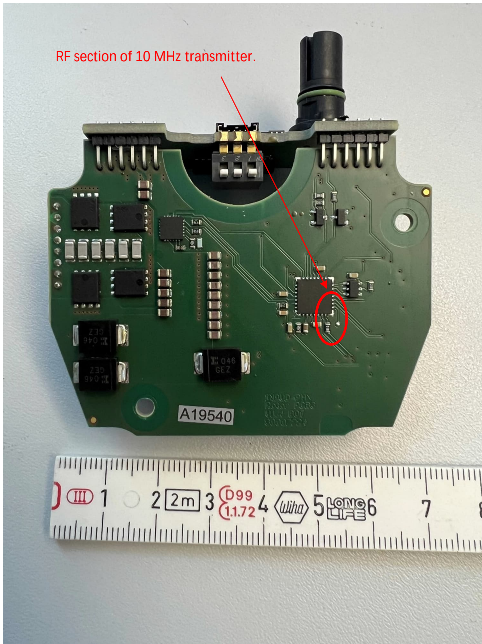
PCB Base bottom
