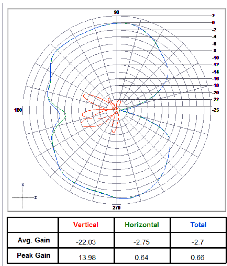
2450.00_XZ Plane
