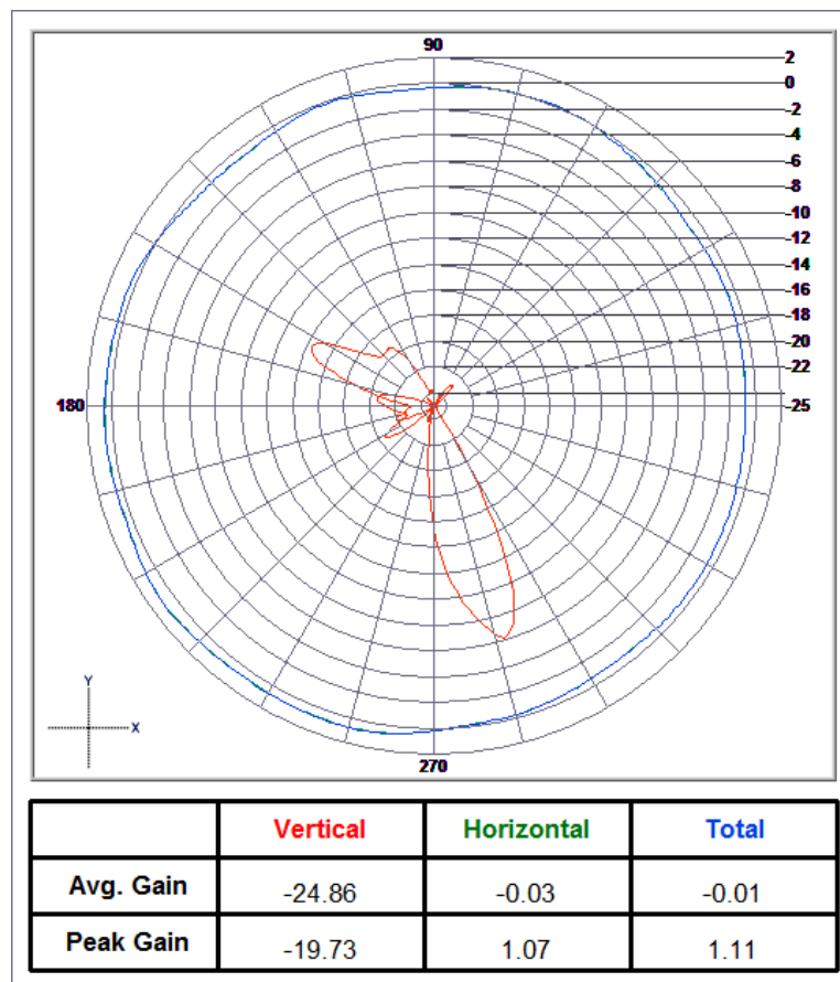
2500.00_XY Plane
