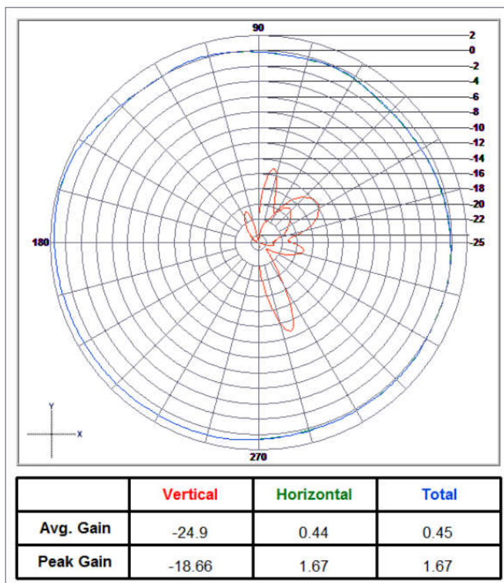
2400.00_XY Plane
