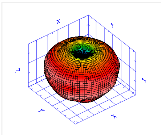
2440.00_3D
