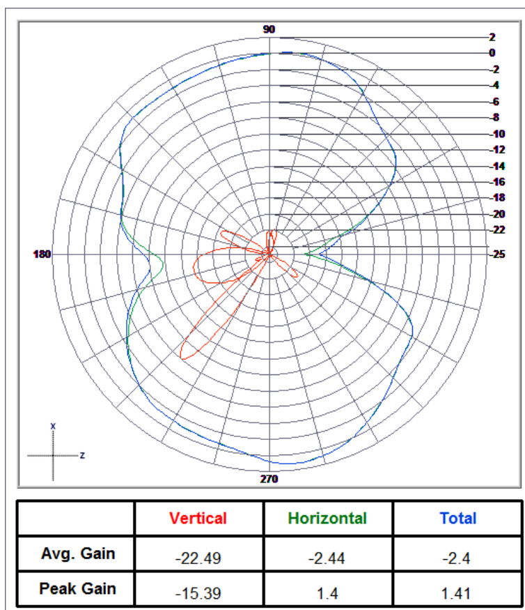
2400.00_XZ Plane
