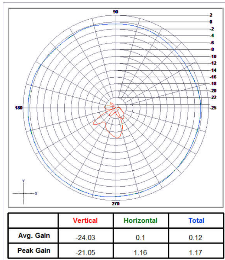
2450.00_XY Plane
