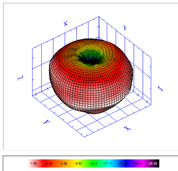
2500.00_3D
