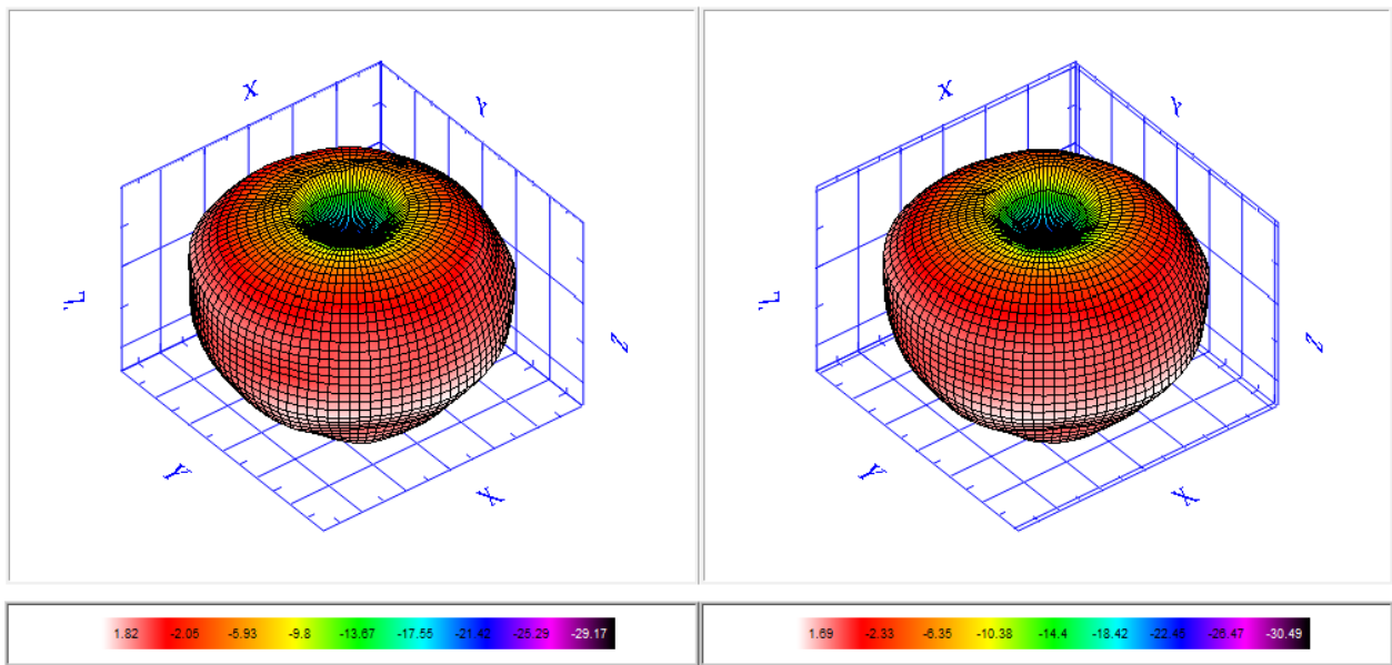
2480.00_3D
