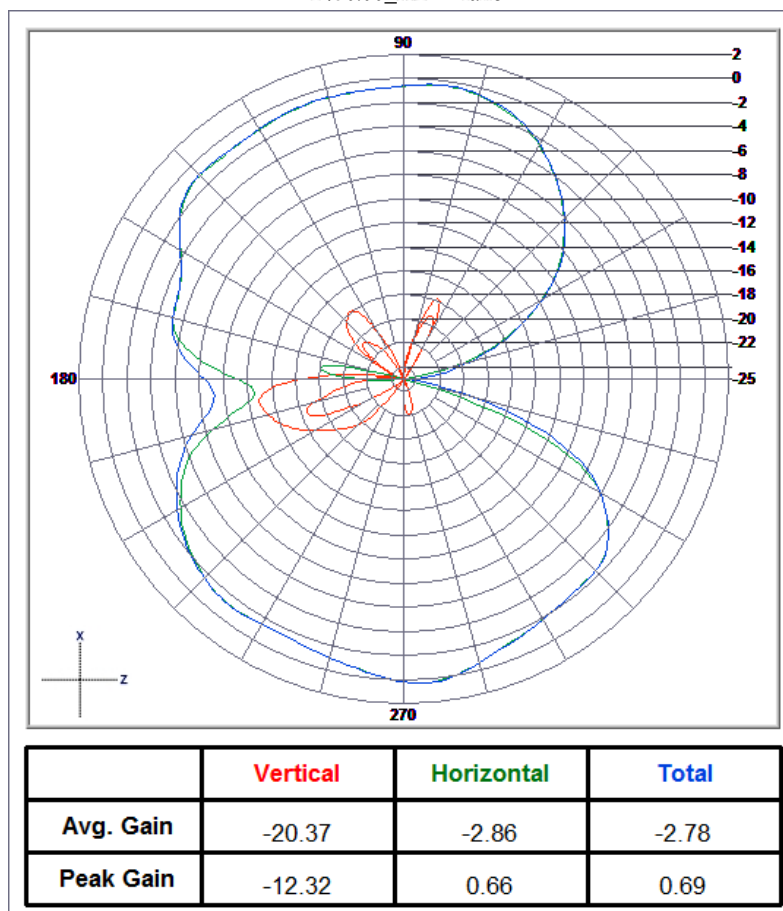
2450.00_XZ Plane
