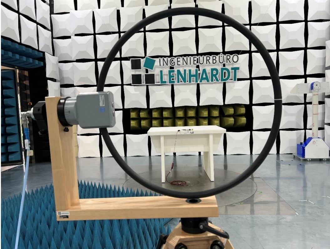
Photo No. 12, measurement in SAC, overall view 1:
