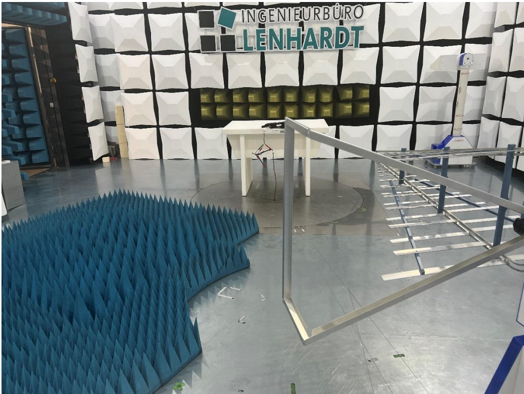
Photo No. 8, measurement in SAC, overall view 2:
