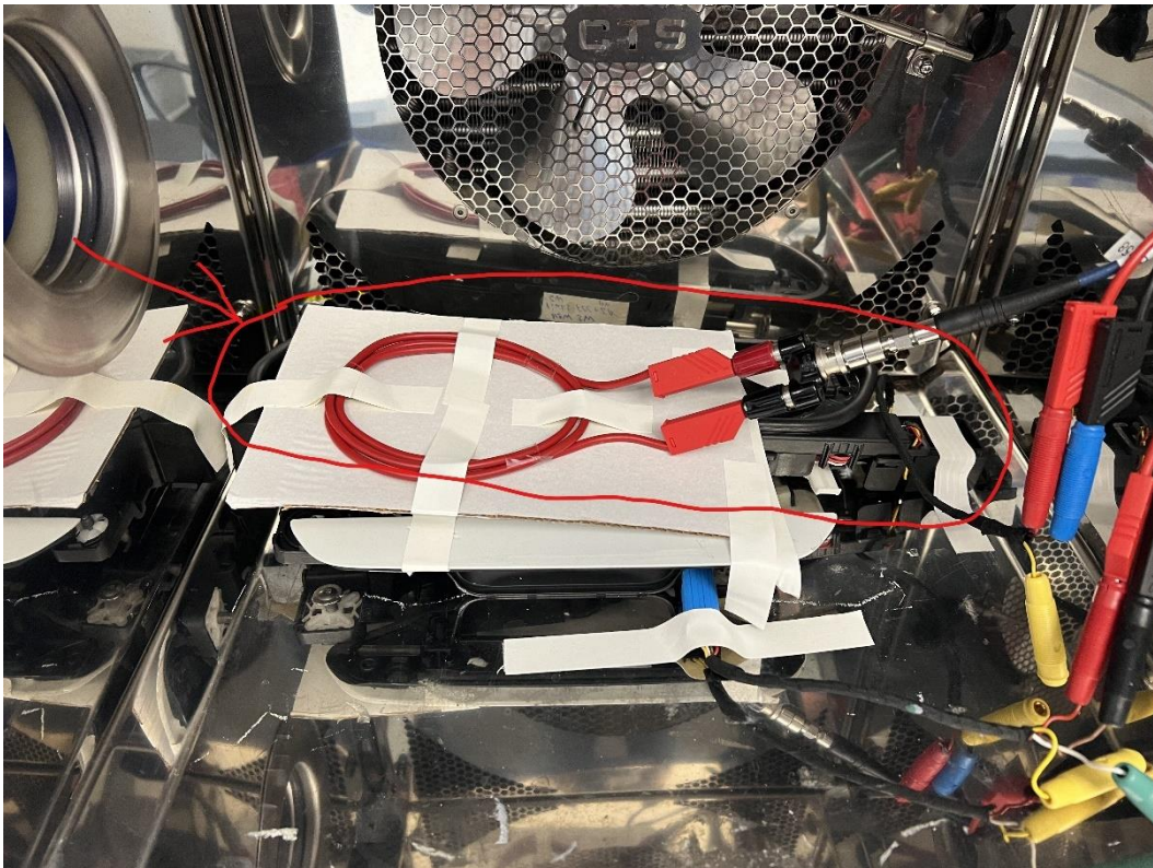
Photo No. 12, measurement in climatic chamber, close view:
