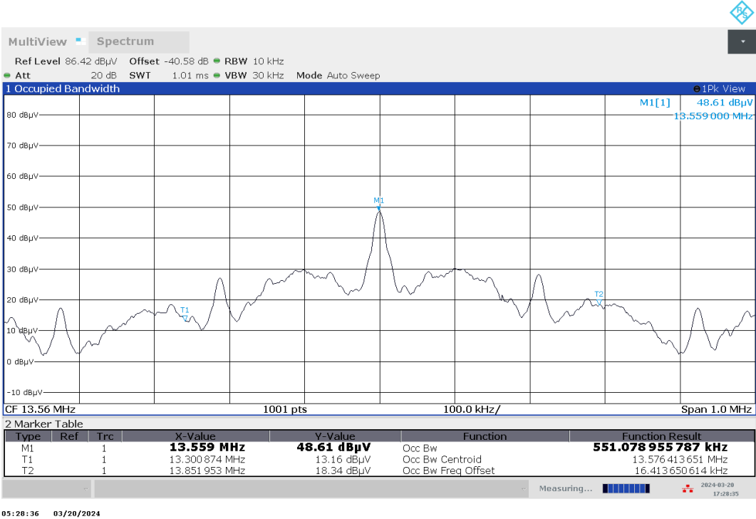
Plot no. 13: Frequency tolerance @ -40 °C, EUT A, Vnom
