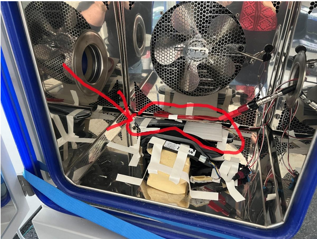
Photo No. 14, measurement in climatic chamber, close view:
