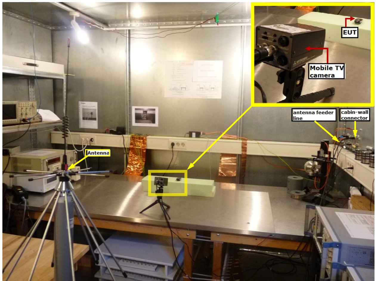
Photo 2: Setup for the test "Blocking" (inside the shielded cabin)
