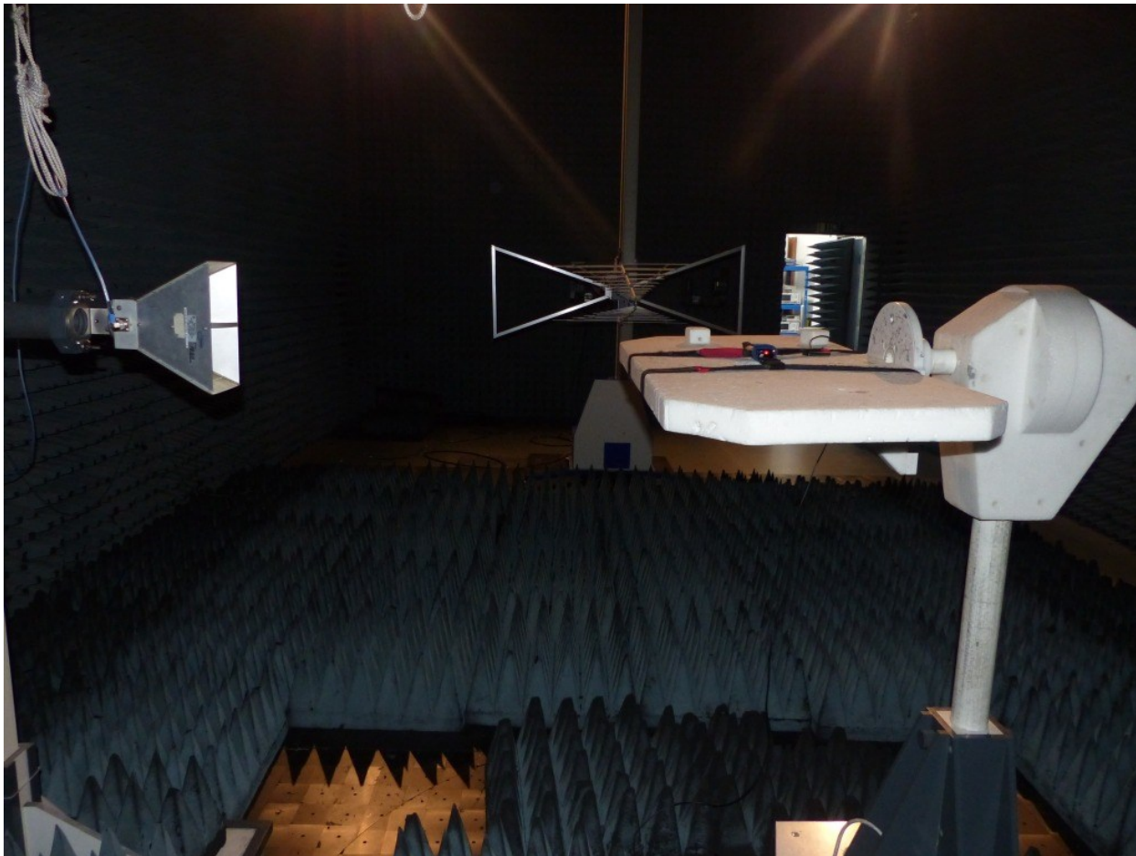
Photo 1: Test setup for radiated measurements
