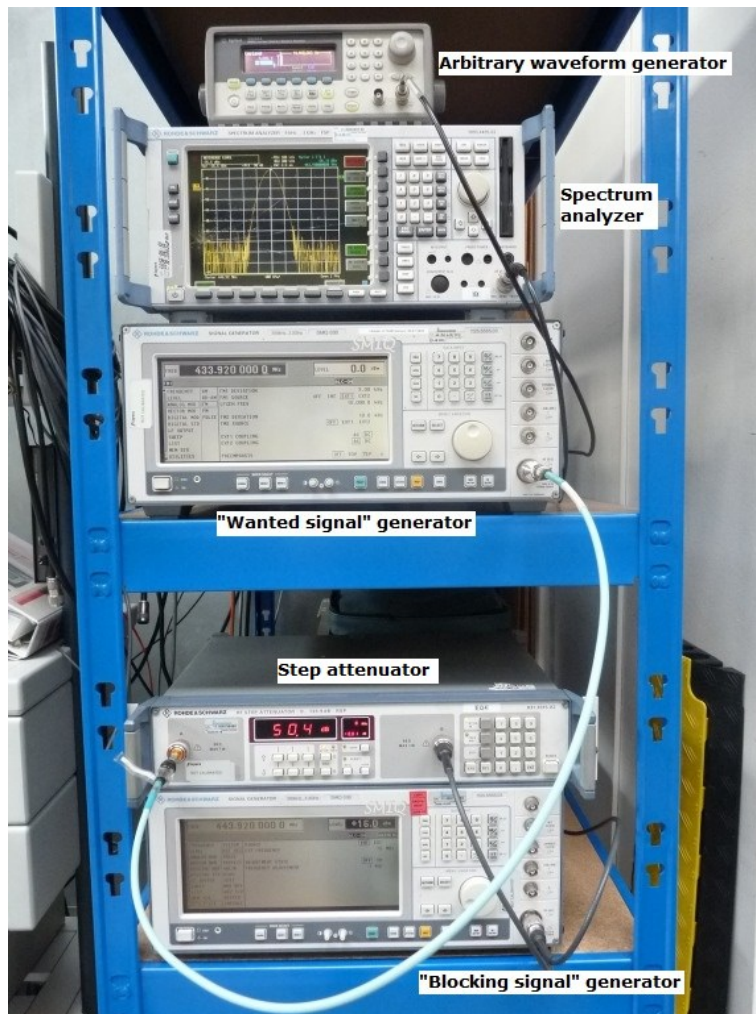
Photo 3: Setup for the test "Blocking" (outside the shielded cabin)
