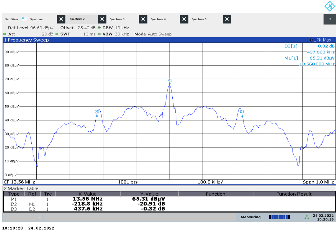
Plot No. 15: 20 dB bandwidth, Left handle
