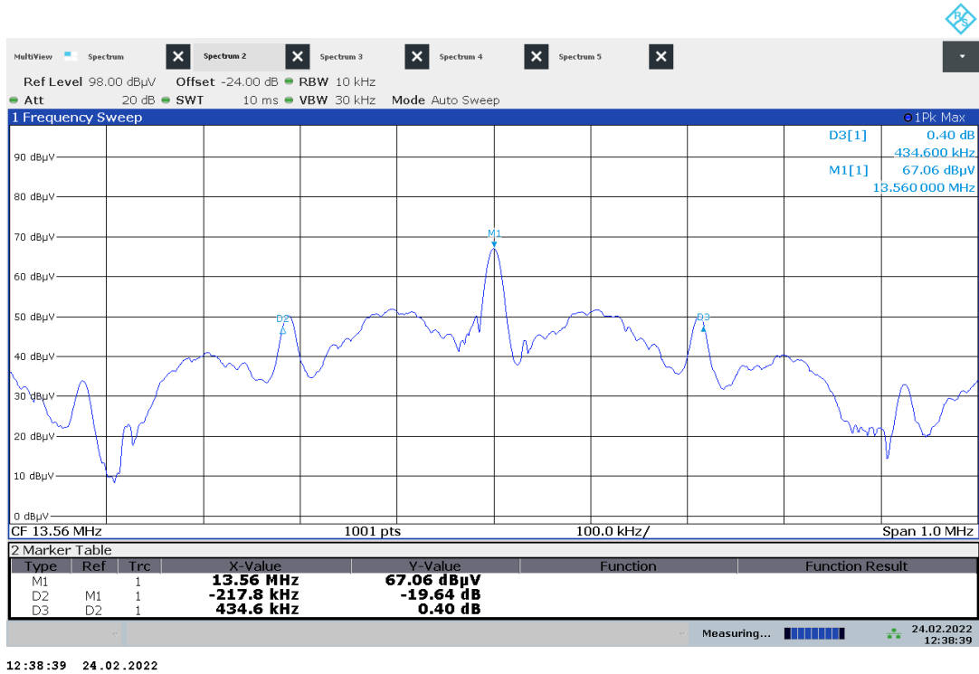
Plot No. 16: 20 dB bandwidth, Right handle
