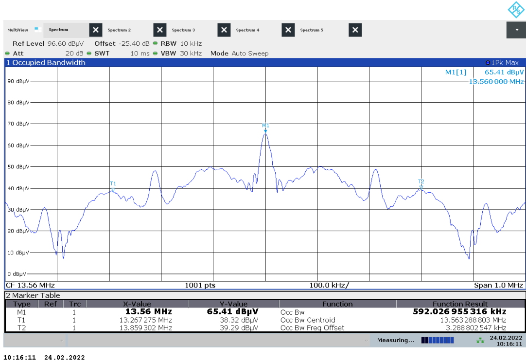
Plot No. 13: 99% Occupied bandwidth, Left handle
