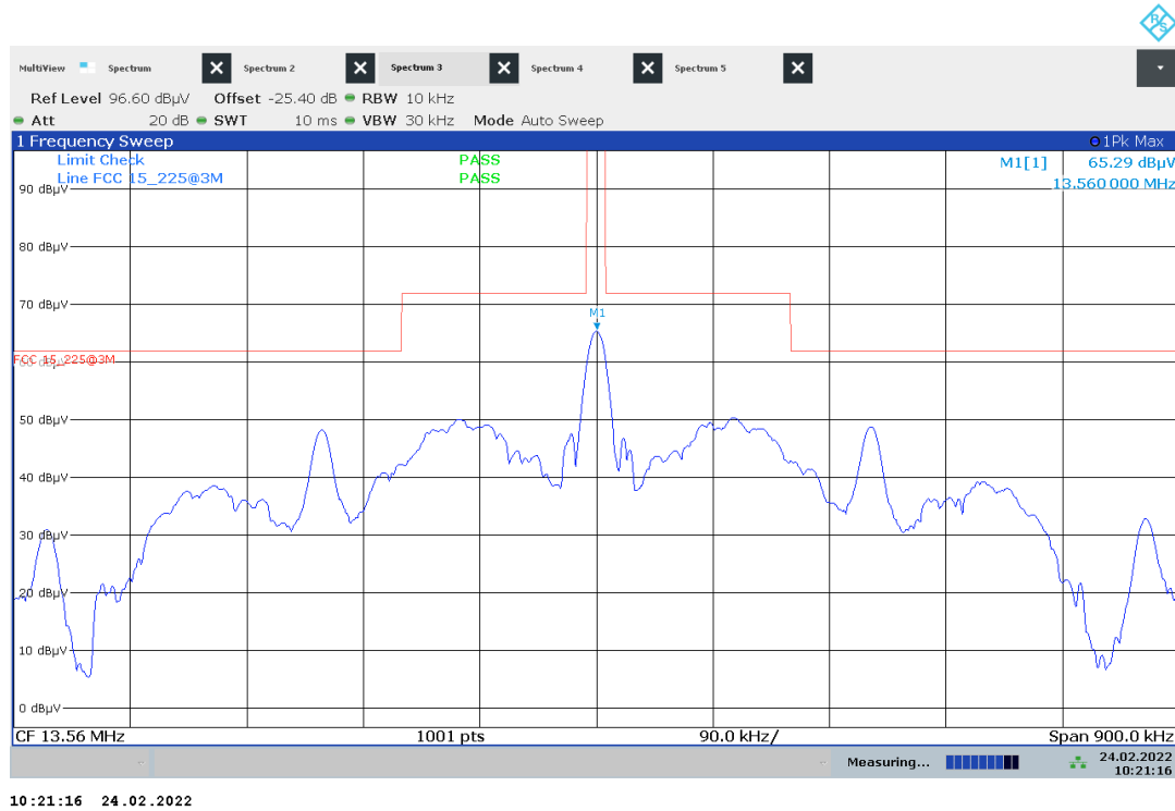
Plot no. 1: Transmitter Spectrum Mask (TSM), Left handle
