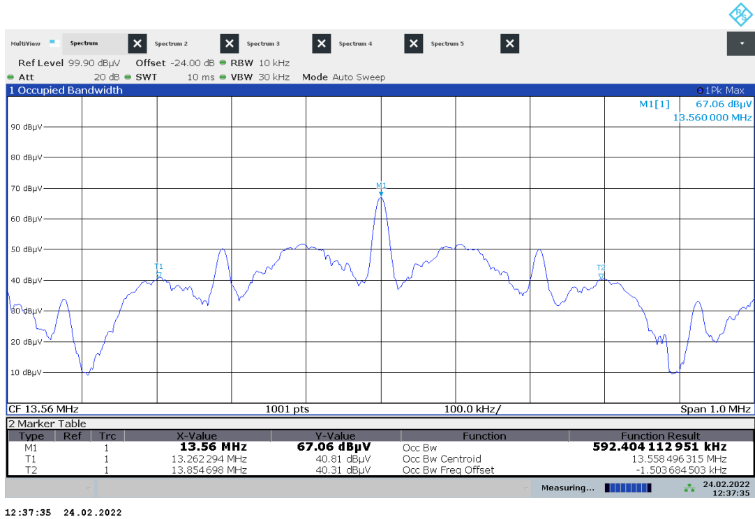
Plot No. 14: 99% Occupied bandwidth, Right handle
