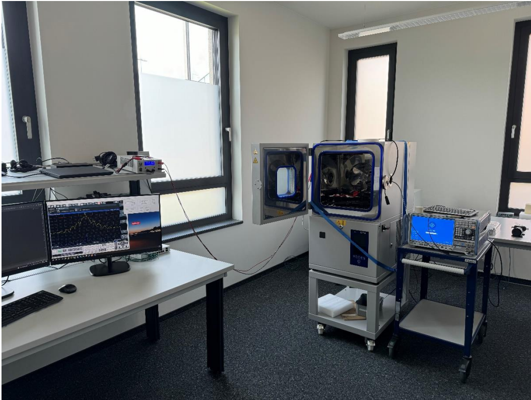
Photo No. 10, measurement in climatic chamber, overall view:
