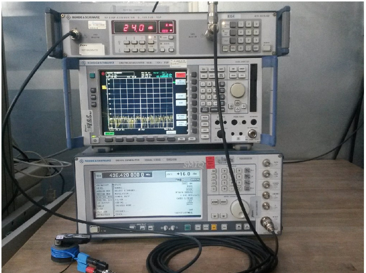
Photo 3: Setup for the test "Blocking" (outside the shielded cabin)
