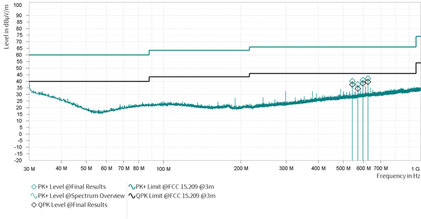
Plot no. 6: Radiated emissions 30 MHz – 1 GHz, hor./vert. polarization, EUT standing (see photos in annex B for EUT position)
