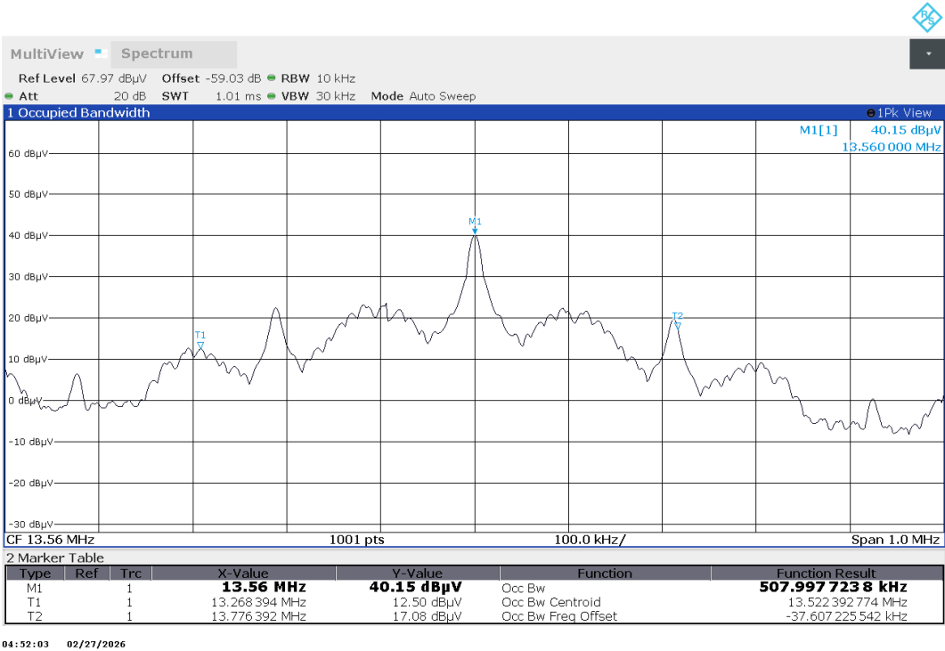
Plot No. 16: 99% Occupied bandwidth
