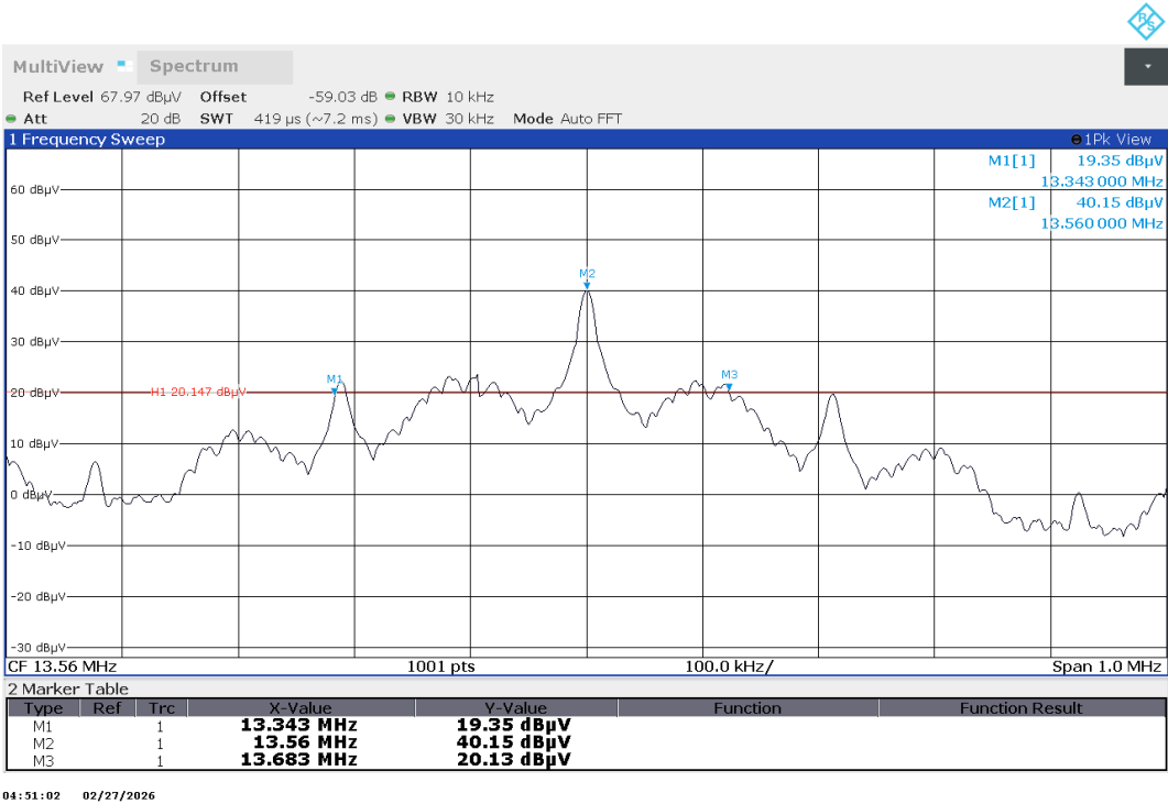
Plot No. 17: 20 dB bandwidth
