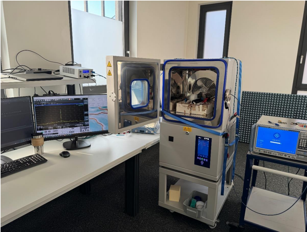
Photo No. 15, measurement in climatic chamber, overall view:
