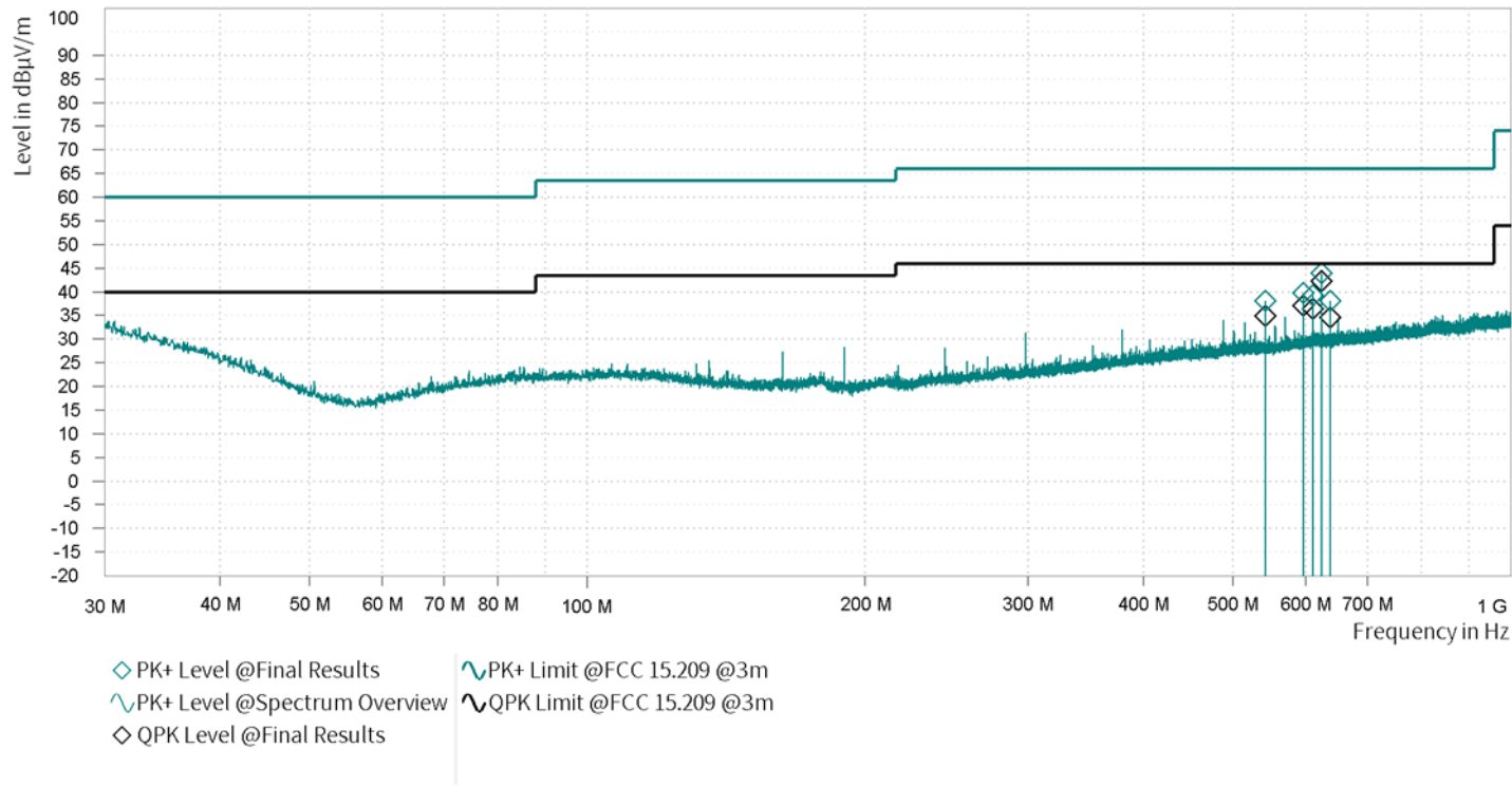
Plot no. 5: Radiated emissions 30 MHz – 1 GHz, hor./vert. polarization, EUT lying (see photos in annex B for EUT position)
