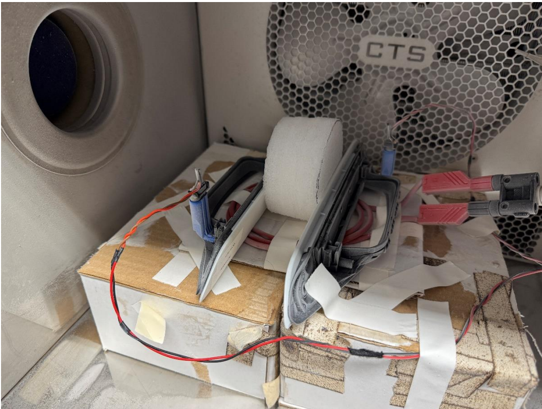
Photo No. 16, measurement in climatic chamber, close view:
