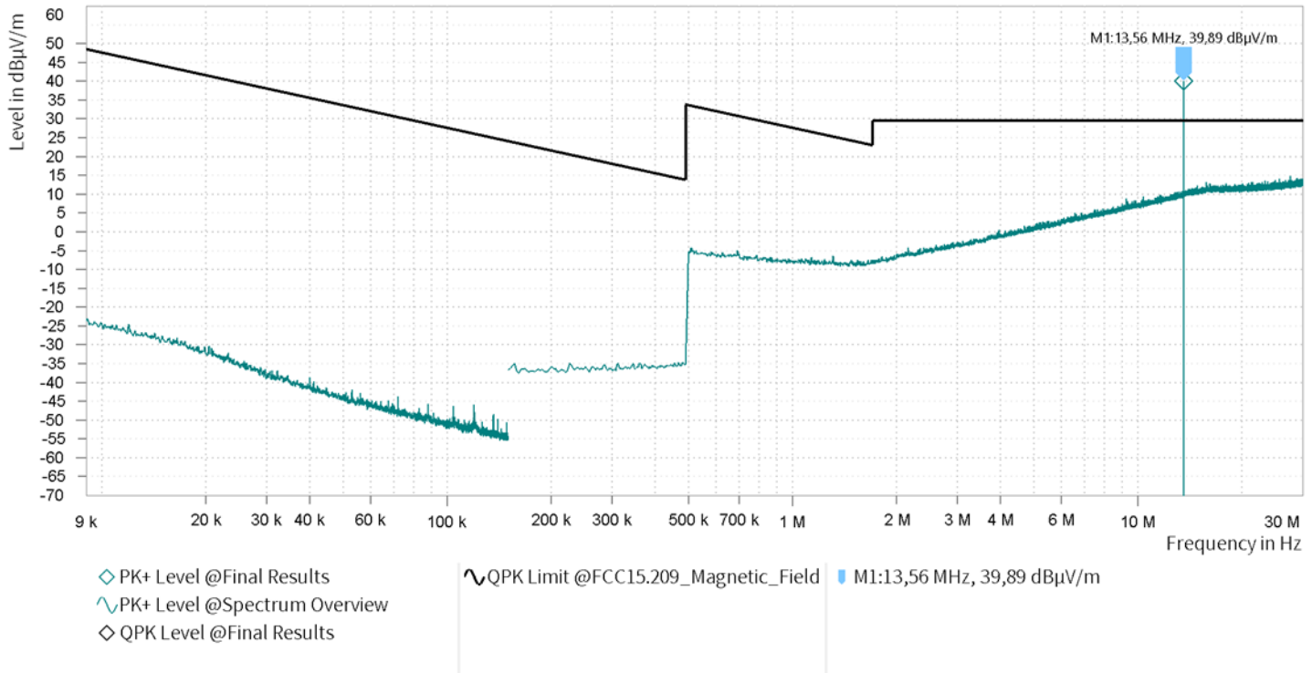
Plot no. 3: Radiated emissions 9 kHz – 30 MHz, EUT lying (see photos in annex B for EUT position)
