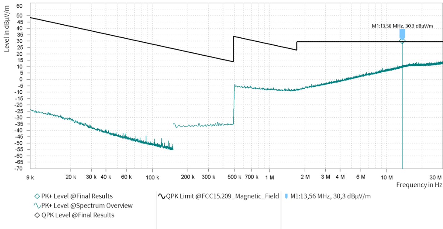
Plot no. 4: Radiated emissions 9 kHz – 30 MHz, EUT standing (see photos in annex B for EUT position)
