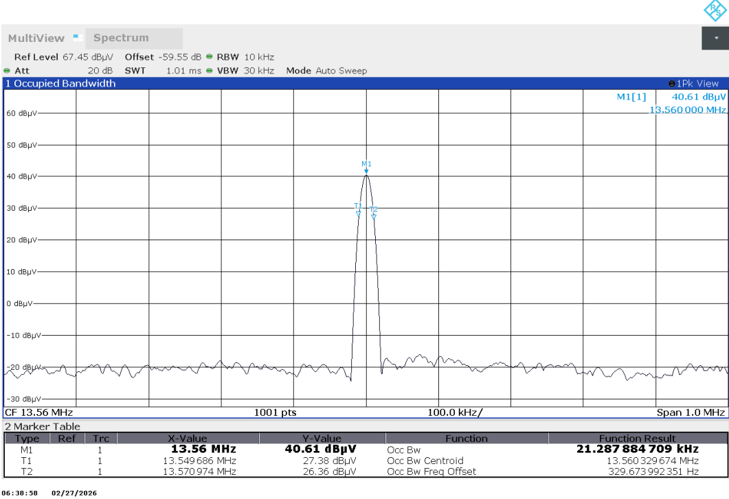
Plot no. 12: Frequency tolerance @ -40 °C, EUT A, Vmax
