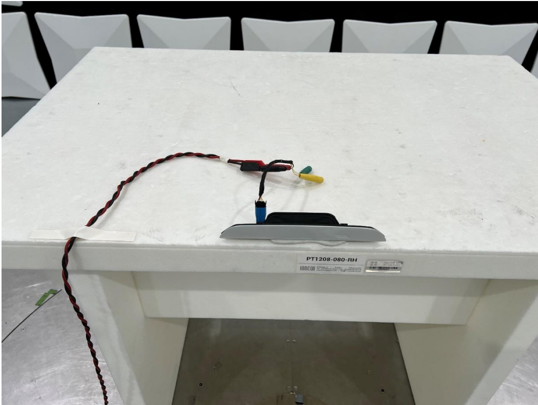
Photo No. 13, measurement in SAC, close view, EUT staying:
