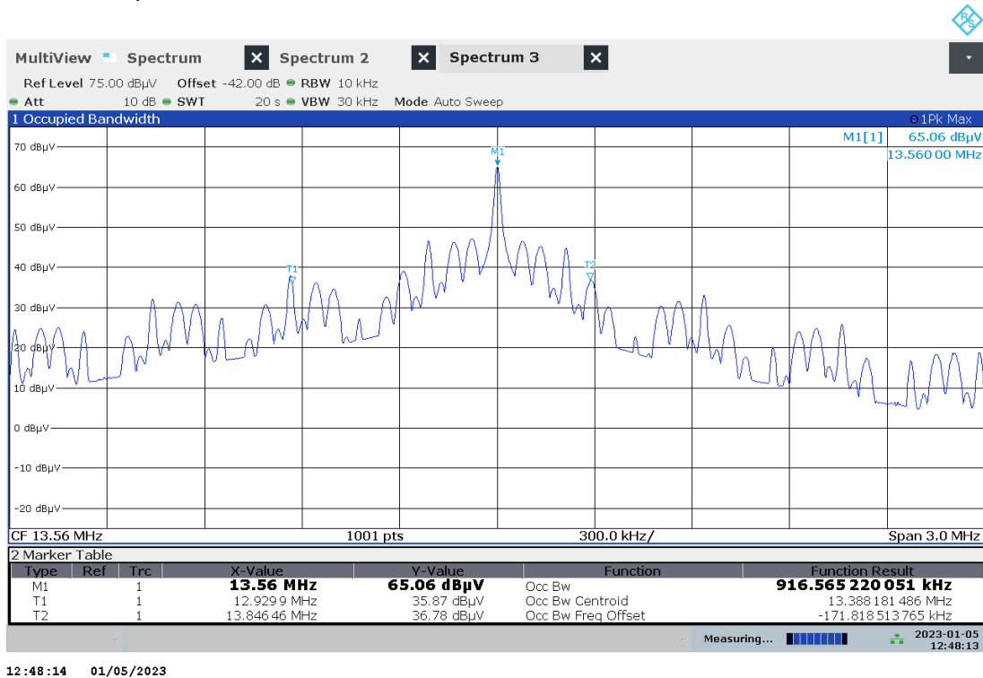
Plot No. 10: 99% Occupied Bandwidth
