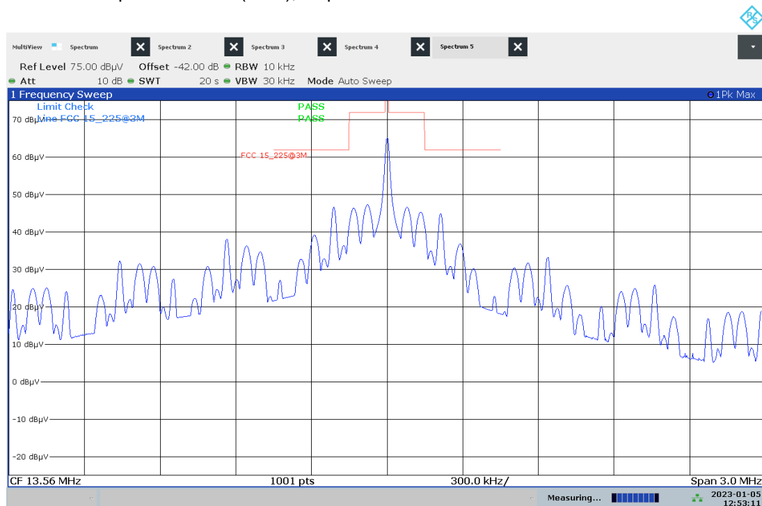
Plot no. 1: Transmitter Spectrum Mask (TSM), loop antenna
